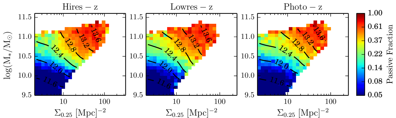
Figure 10. Fraction of passive galaxies as a function of density on the scale \Sigma_{0.25} and stellar mass for mass rank 1 galaxies (in the adaptive aperture) using hires-z (left panel), lowres-z (central panel), and photo-z (right panel) at z = 1.08 . The contours are drawn from the median halo mass in the same bins.
