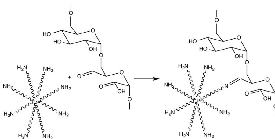
FIGURE 5. Dextran-PEG adhesive: the oxidized dextran aldehyde reacts with an aminated PEG to form a crosslinked hydrogel network through imine bond formation. (Reproduced from Ref. 89).
