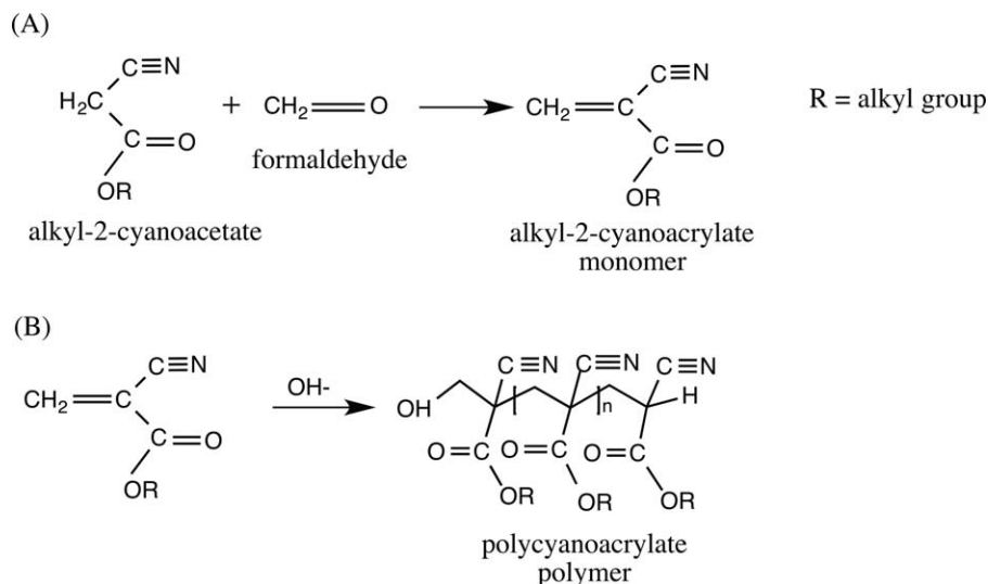
FIGURE 6. Cyanoacrylate chemistry: (A) Synthesis of alkyl-2-cyanoacrylate monomer and (B) polymerization reaction.
