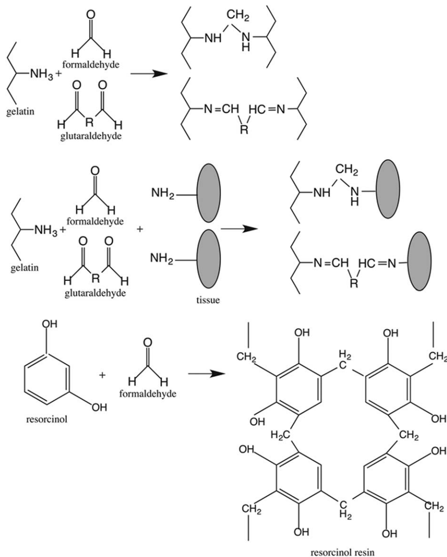
FIGURE 2. Crosslinking of gelatin with aldehydes and resorcinol (Reproduced from Ref. 2).
