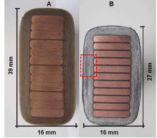
Figure 1. Cross sections of two coils under test. A) Type-A and B) Type-B ground-wall insulation. The dotted lines indicates qualitatively the coil portion removed and scanned with X-CT.
