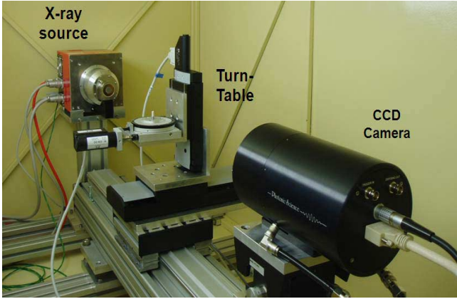
Figure 2. The X-CT set-up.
