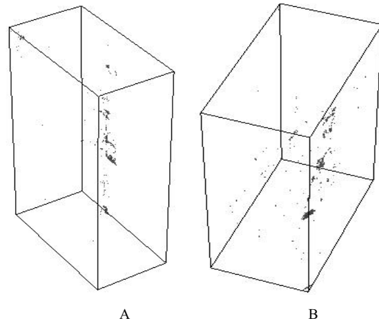
Figure 17. The segmented 3D digital image of a VOI relevant to insulation Type-B. A) Type-B1 and B) Type-B2 coil samples.
