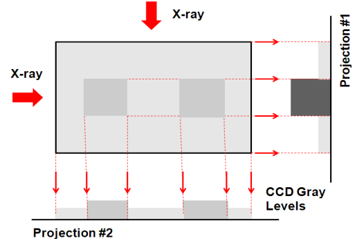
Figure 3. Sketch of the X-CT projections of an object having higher density inclusions.
