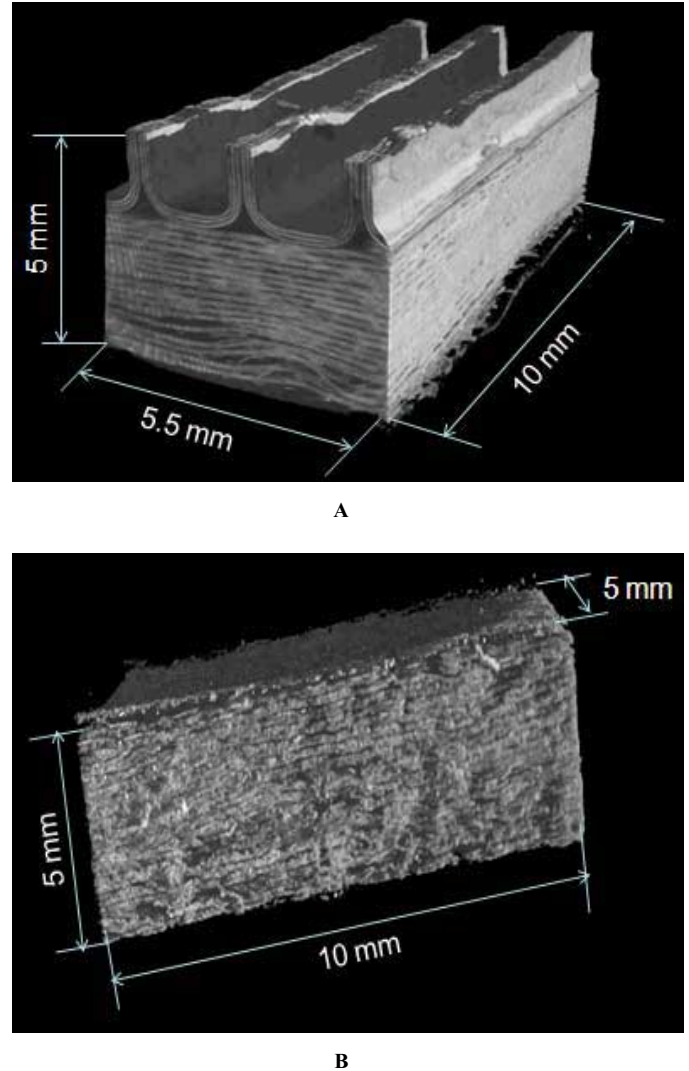
Figure 5. Different views of two samples: A) Type-B2 and B) Type-A1 ground-wall insulation.
