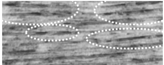
Figure 19. Detail of rounded voids within Type-B1 sample.
