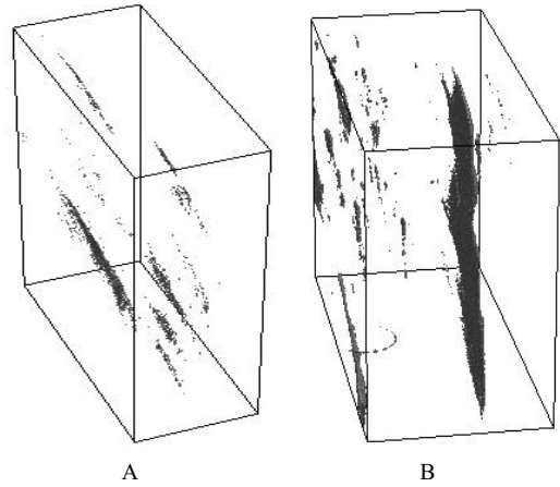
Figure 16. The segmented 3D digital image of a VOI relevant to insulation Type-A. A) Type-A1 and B) Type-A2 coil samples.
