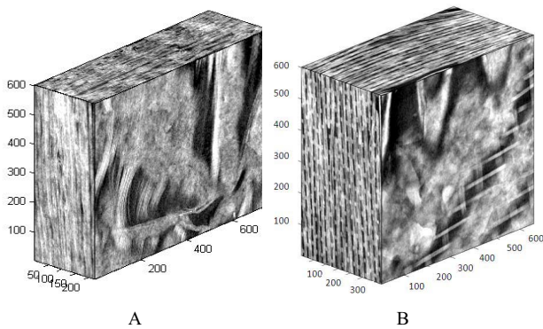
Figure 15. Examples of 3D digital images of VOIs relevant to A) Type-A2 and B) Type-B1 insulation.
