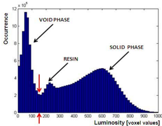
Figure 9. Example of luminosity histogram related to a coil sample.
