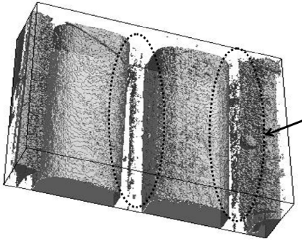
Figure 14. Detail of the void distribution relevant to the sample Type-B2 after a multi-phase segmentation.
