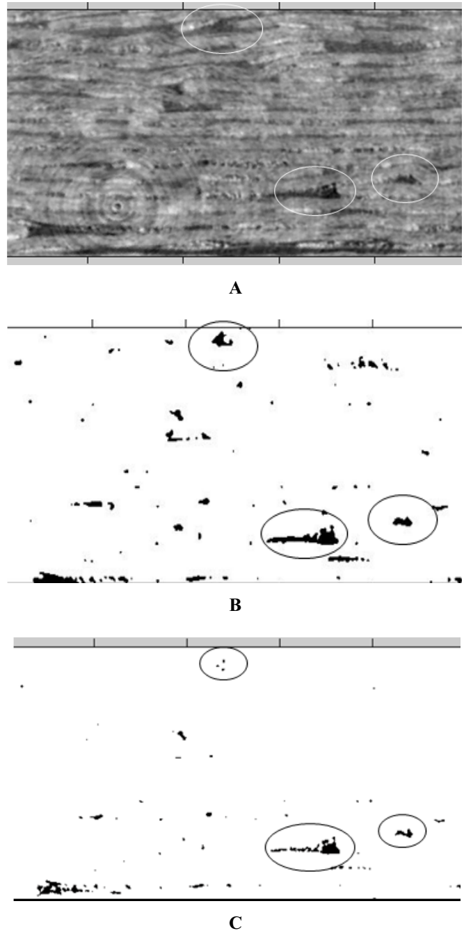
Figure 11. Detail of a slice relevant to sample Type-A2 of Figure 10, (A) and the relevant void distributions assuming 150 and 50 luminosity threshold level values.
