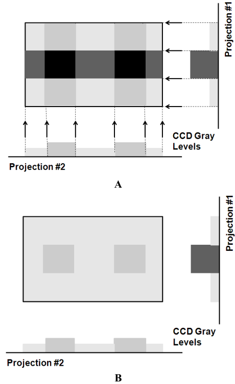
Figure 4. Sketch of the back-projection algorithm. A) the back projection of the radiographies; B) the object reconstruction after data normalization.
