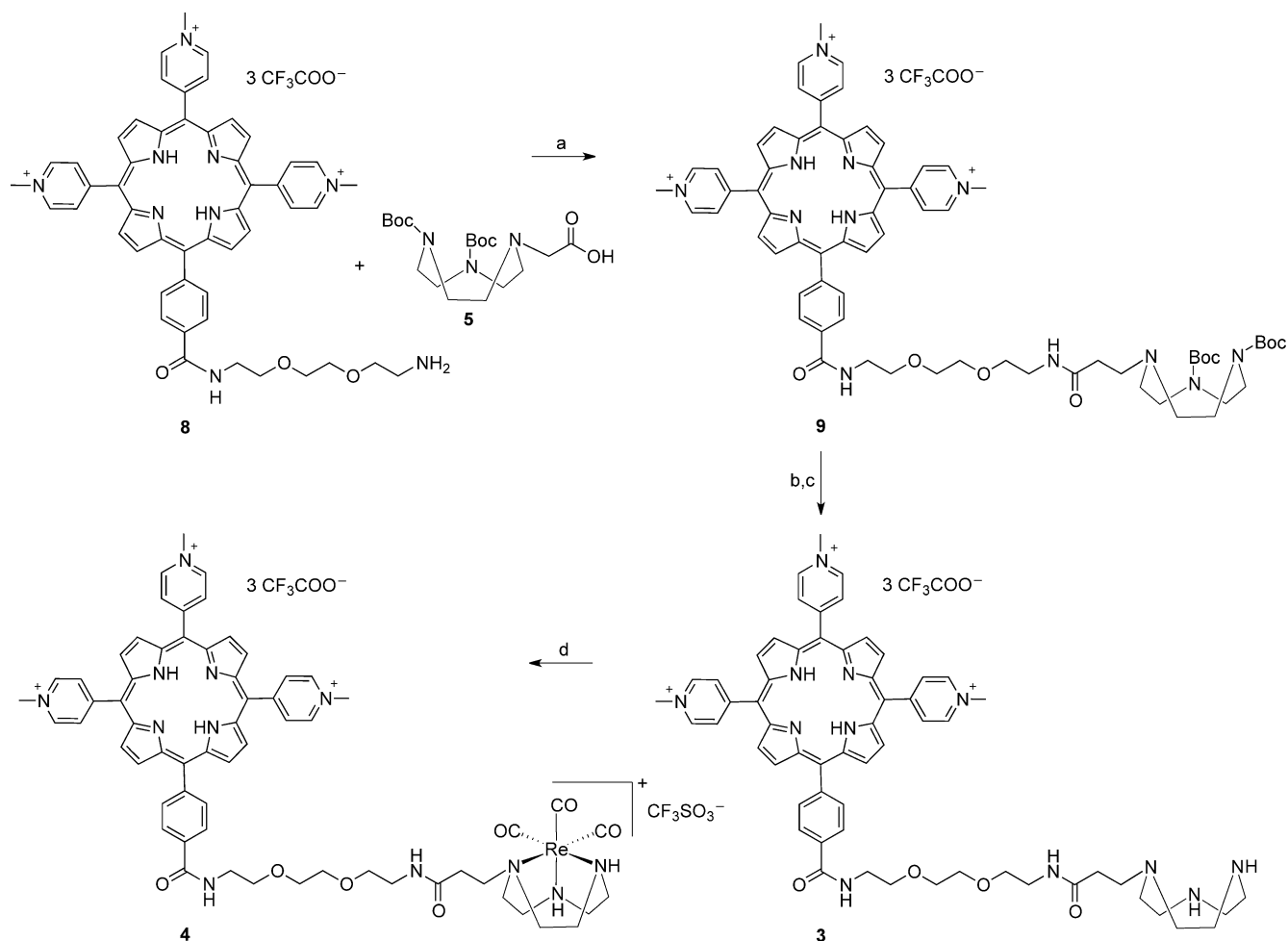
Scheme 2. Synthetic route to 3 and 4 . Reagents and conditions: a) DMAP, EDCl, HOBT, DMF, MW 6 min, 60 °C, 66%; b) TFA, CH 2 Cl 2 , 3 h, RT; c) TEA, CH 3 OH/Et 2 O, 98%; d) fac -[Re(CO) 3 (dmsO-O) 3 ](CF 3 SO 3 ), CH 3 OH, MW 10 min, 110 °C, 73%.
