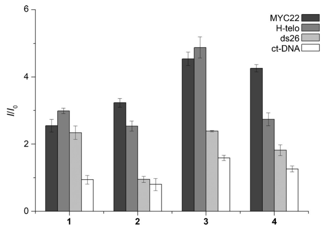
Figure 5. Bar chart showing changes in the emission intensity (determined by integration of the emission between \lambda = 600 –850 nm) of the compounds (Tris/KCl buffer) upon addition of 20 equiv Myc22, H-telo, ds-26, and ct-DNA; \lambda_{\text{ex}} : 1 , 430 nm; 2 , 430 nm; 3 , 445 nm; 4 , 445 nm.
