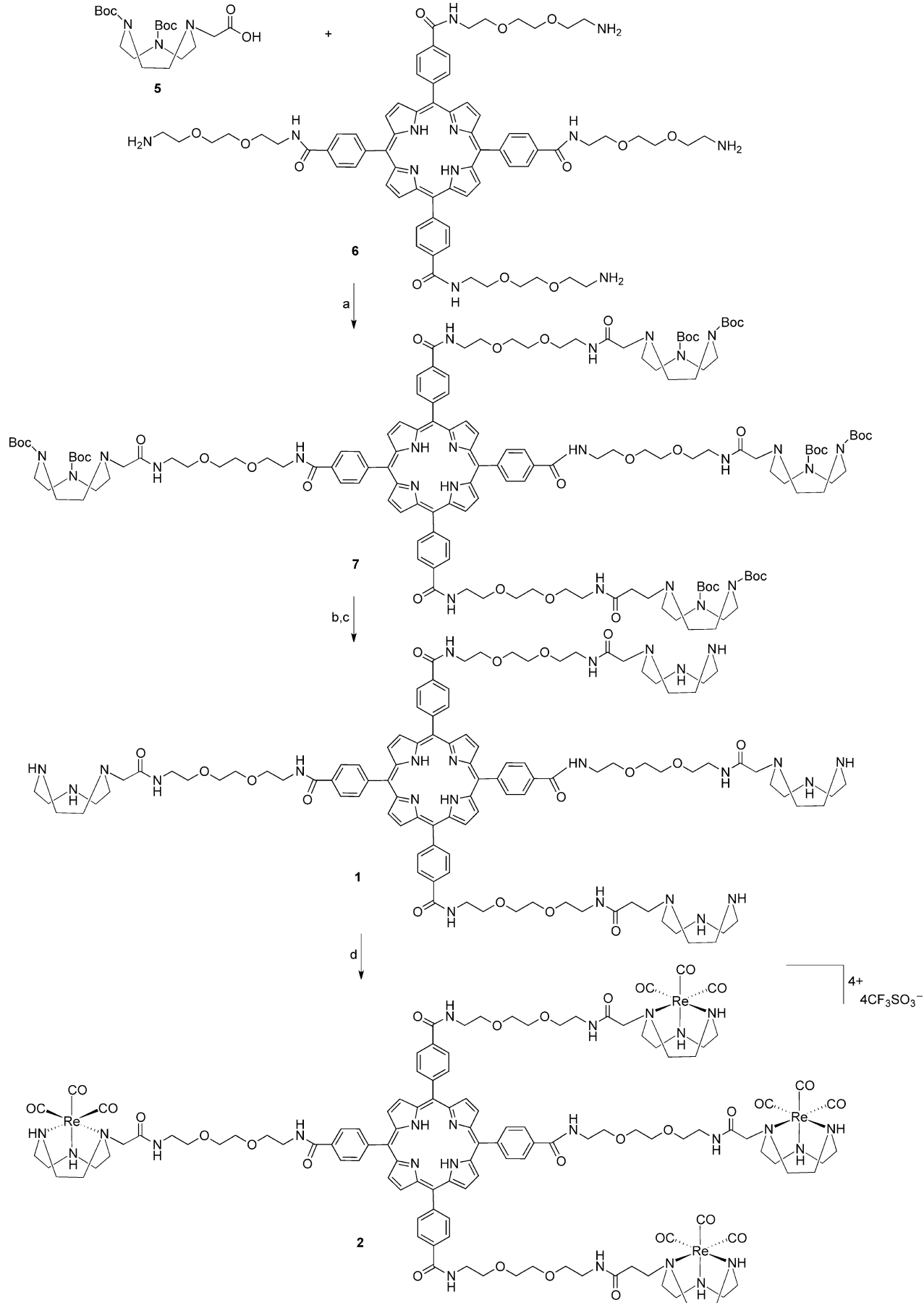
Scheme 1. Synthetic route to 1 and 2 . Reagents and conditions: a) DMAP, EDCI, HOBT, DMF, 24 h, RT, 66%; b) CH_2Cl_2 , TFA, 3 h, RT; c) CH_3OH , TEA, Et_2O , 97%; d) fac-[Re(CO)_3(dmsO)_3](CF_3SO_3) , anhydrous CH_3OH , 48 h, 70 °C, reflux, 65%.
