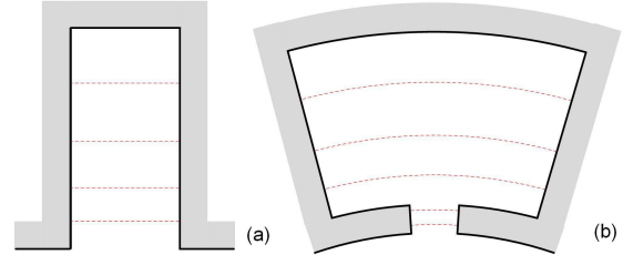
Fig. 2. Simplified leakage flux patterns (dashed lines) for (a) open rectangular slot and (b) semi-closed slot shape.
