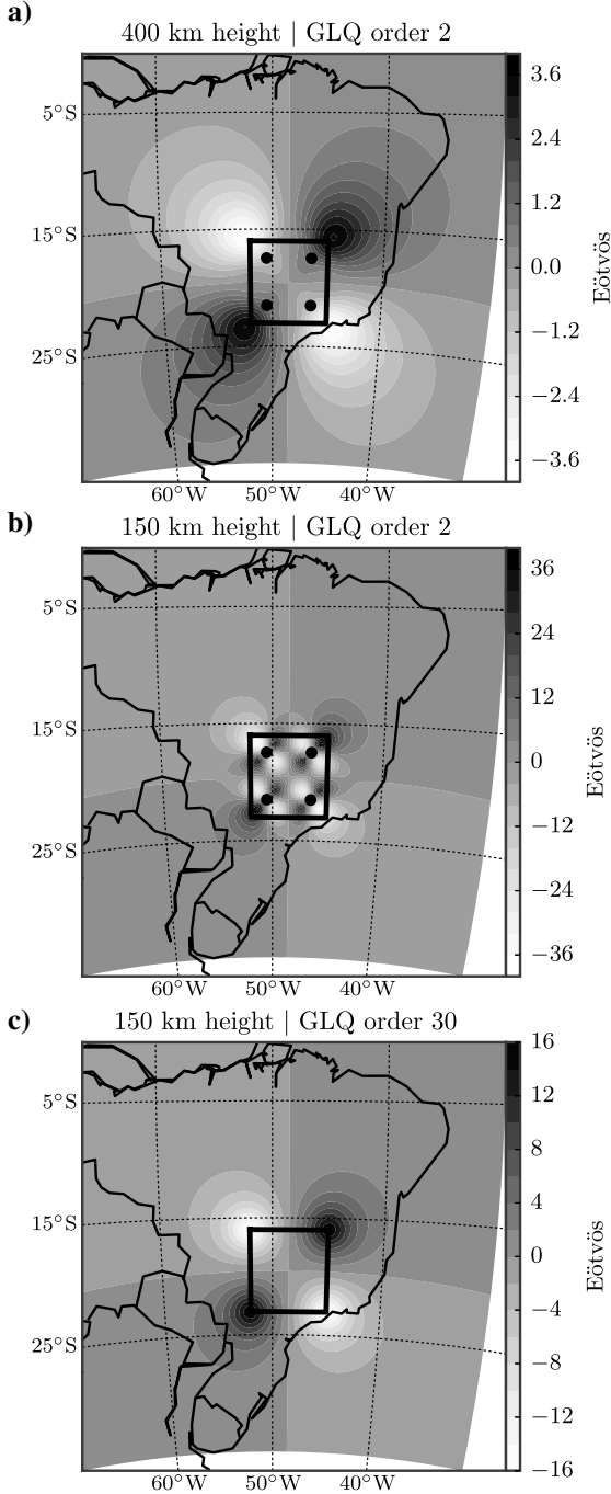
Figure 2. Example of the effect of varying the computation height and the number of point masses in the GLQ. Black circles represent the horizontal location of the point masses. (a) g_y calculated at 400 km height using GLQ order 2 ( 2 \times 2 \times 2 = 8 point masses). (b) At 150 km height and GLQ order 2, the result resembles that of four point masses instead of a single tesseroïd. This effect is shown by Ku (1977) . (c) At 150 km but with a higher GLQ order of 30. In panel (c), the horizontal locations of the point masses were not shown. Note that the results shown in panel (c) are similar to that expected for a single mass source.
