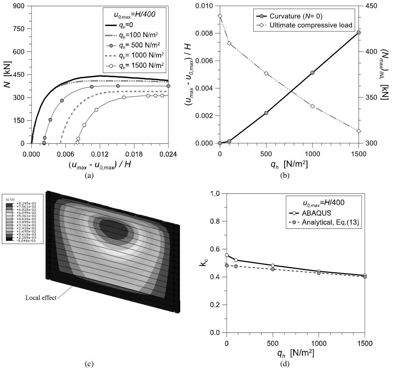
Fig. 12 Effect of out-of-plane pressures q_h acting simultaneously to in-plane compressive loads N ( H=2.95 m, L=3 m, b=8 cm; RF configuration), with u_{0,max} = H/400 : (a) dimensionless compressive load – out-of-plane deflection curves. (b) Qualitative effect of out-of-plane pressures q_h and initial curvatures u_{0,max} on the buckling response of an in-plane compressed timber log-wall with a (c) typical deformed configuration due to N - q_h loads (displacements in meters, N=420 kN, q_h=1500 N/m 2 ). (d) buckling coefficient k_c depending on out-of-plane pressure q_h
