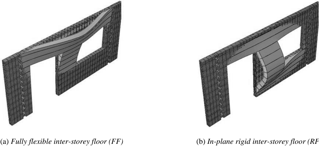
Fig. 2 Qualitative fundamental buckling shape for log-walls with (a) fully flexible or (b) in-plane rigid inter-storey floor, under in-plane compressive loads (Bedon and Fragiacomò 2015)
