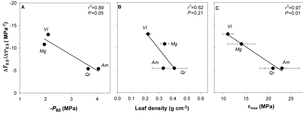
Fig. 5. Relationships between the slope of leaf shrinkage at \Psi_L = -0.5 MPa ( \Delta T_{0.5}/\Delta \Psi_{0.5} ) and (A) leaf water potential inducing 80% loss of hydraulic conductance ( P_{80} ), (B) leaf density (mean values \pm SD), and (C) bulk modulus of elasticity ( \epsilon_{max} , mean values \pm SD) as recorded in the species under study. Regression curves are expressed by the following function: y = y_0 + ax . Values of correlation coefficients ( r^2 ) and P -values are indicated. See Table 1 for abbreviations of species' names.
