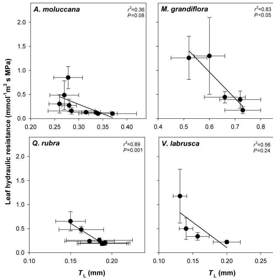
Fig. 4. Mean values ( \pm SD) of leaf hydraulic resistance versus leaf thickness ( T_L ) as recorded at 0.5 MPa intervals during dehydration in leaves of the study species. Regression curves are expressed by the following function: y = y_0 + ax . Correlation coefficients ( r^2 ) and P -values are indicated.
