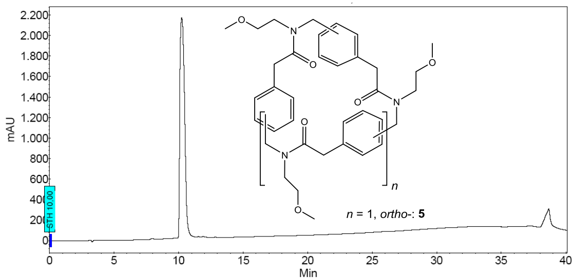
Figure S19: HPLC chromatogram of trimeric cyclic 3-5 as crude mixture Conditions: 5 → 100% A in 30 min (A, 0.1% TFA in acetonitrile, B, 0.1% TFA in water); flow: 1 mL min -1 , 220 nm
