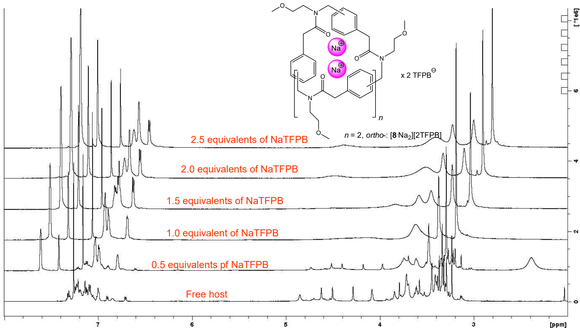
Figure S16. Titration experiment on compound 8 to give complexes [\mathbf{8}\cdot\text{Na}]^+ and [\mathbf{8}\cdot 2\text{Na}]^{2+} . ^1\text{H-NMR} : 600 MHz, \text{CDCl}_3 . Offset: 0.1 ppm.
