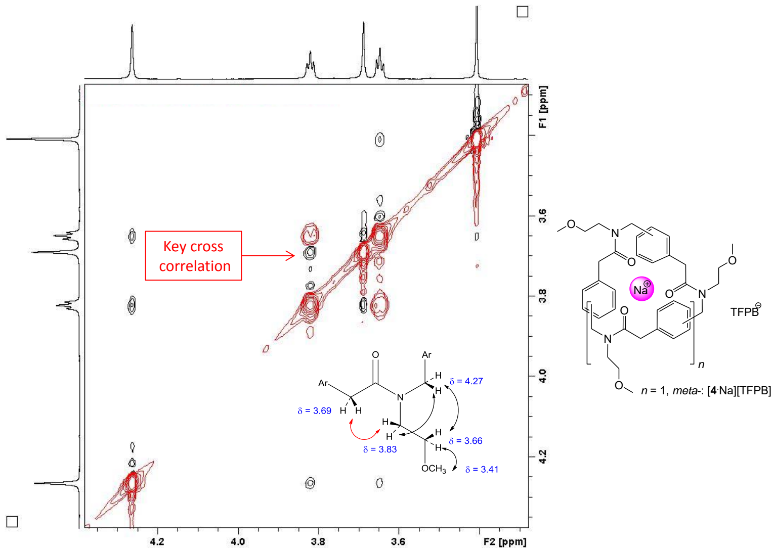
Figure S8. Enlargement of the ROESY experiment for the complexed benzyloptoid [4 \cdot \text{Na}]^+ (600 MHz, \text{CDCl}_3 ). Note: dipolar coupling in black and scalar coupling in red.
