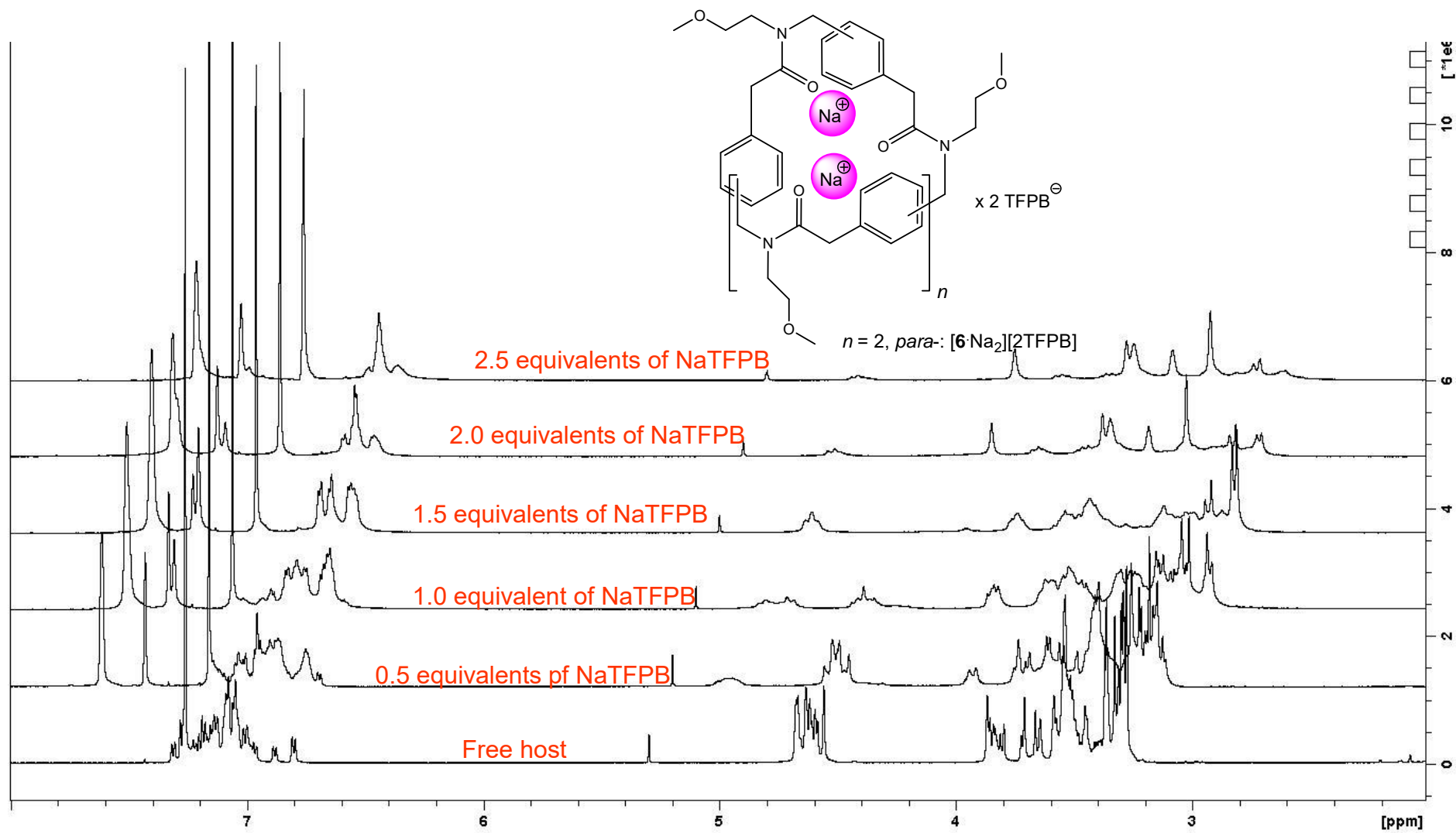
Figure S14. Titration experiment on compound 6 to give complex [\text{6} \cdot 2\text{Na}]^{2+} . ^1\text{H-NMR} : 600 MHz, \text{CDCl}_3 . Offset: 0.1 ppm.
