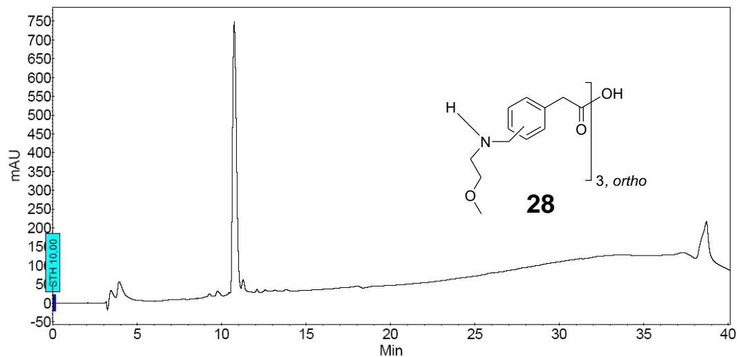
Figure S17: HPLC chromatograms of trimeric linear 26-28 as crude mixture. Conditions: 5 → 100% A in 30 min (A, 0.1% TFA in acetonitrile, B, 0.1% TFA in water); flow: 1 mL min -1 , 220 nm.
