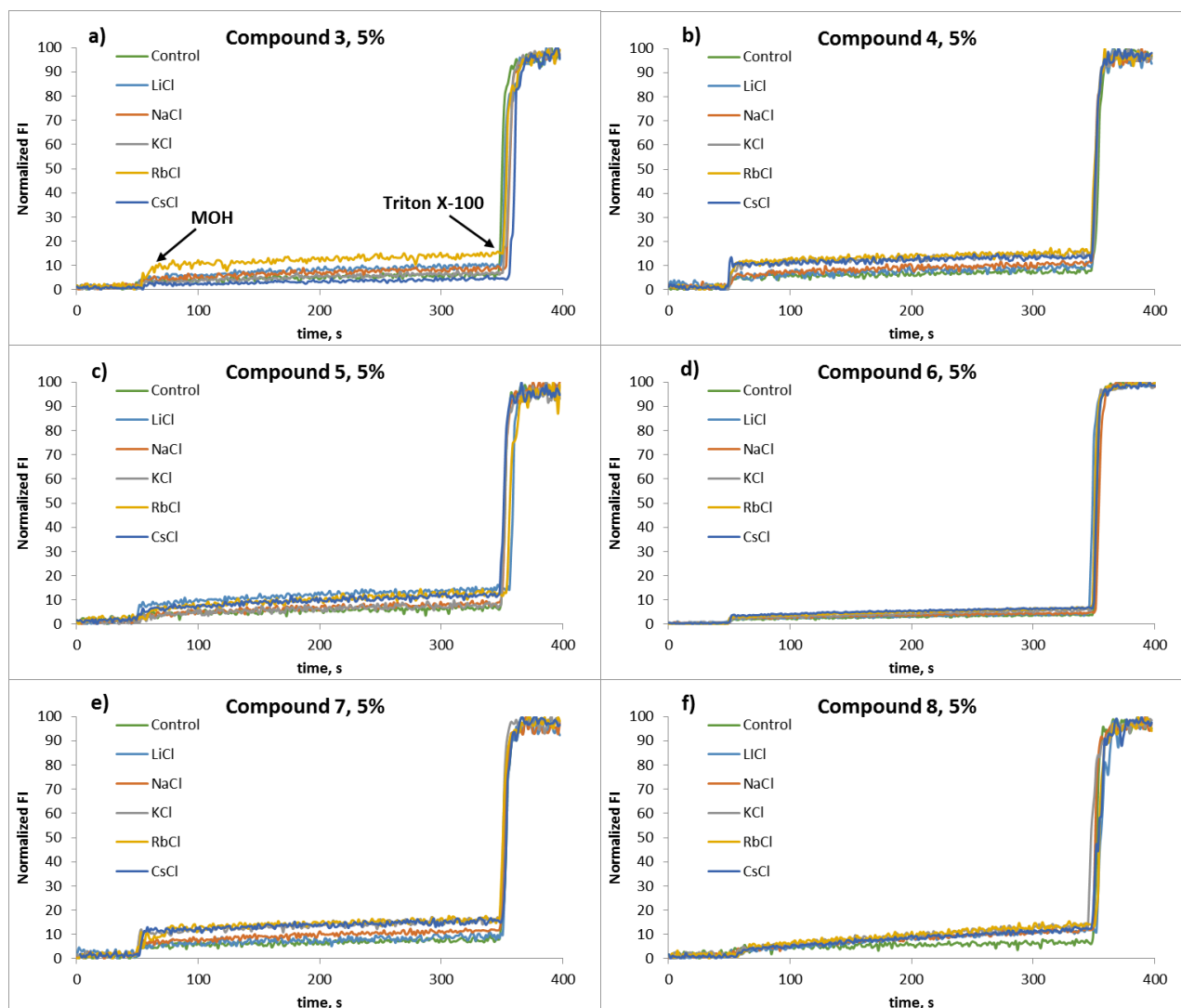
Figure S21: Normalized fluorescence change in HPTS emission as a function of time after addition of the base (50 \mu\text{L} of 0.5 M MOH, with M = \text{Li}^+ , \text{Na}^+ , \text{K}^+ , \text{Rb}^+ , \text{Cs}^+ , depending on the cation present in the extravesicular buffer solution) to 95:5 EYPC/EYPG LUVs (100 nm diameter) loaded with HPTS (0.1 mM HPTS, 0.17 mM total lipid concentration, 25 mM HEPES pH 7.0) and 100 mM MCl (with M = \text{Li}^+ , \text{Na}^+ , \text{K}^+ , \text{Rb}^+ , \text{Cs}^+ ), in the presence of a 5% concentration of compounds 3-8 . The concentration of the ionophore is given in percent with respect to the total lipid concentration. The control trace has been recorded in the absence of ionophore. The arrows indicate the time of MOH and Triton X-100 addition.
