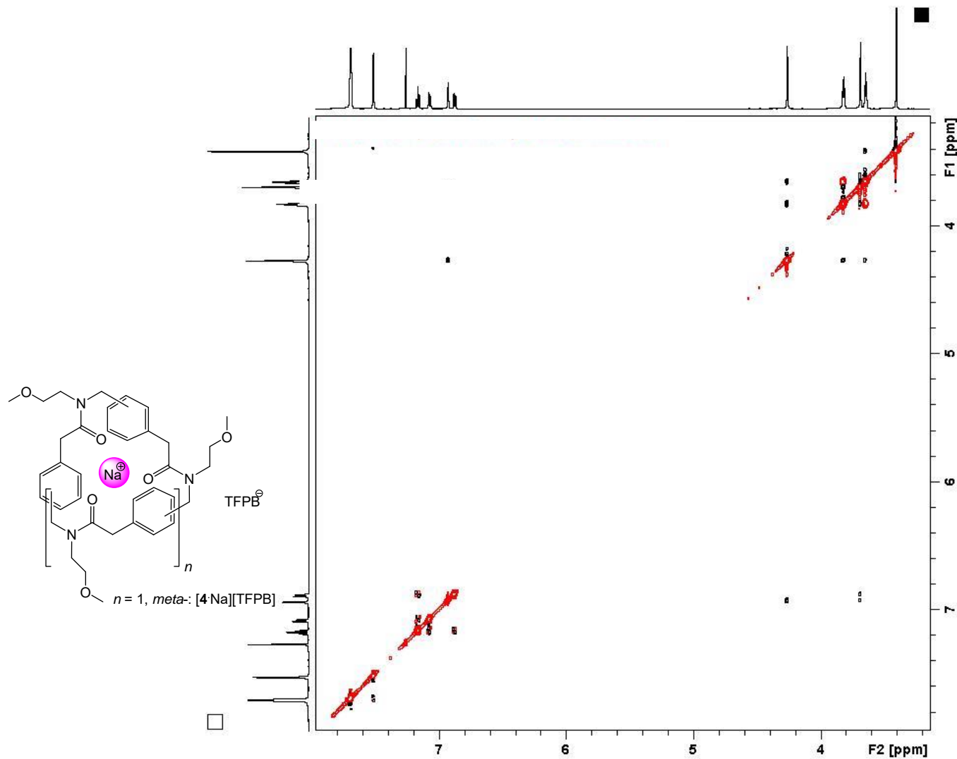
Figure S7. ROESY experiment for the complexed benzyloptoid [4\cdot\text{Na}]^+ (600 MHz, \text{CDCl}_3 ). Note: dipolar coupling in black and scalar coupling in red.
