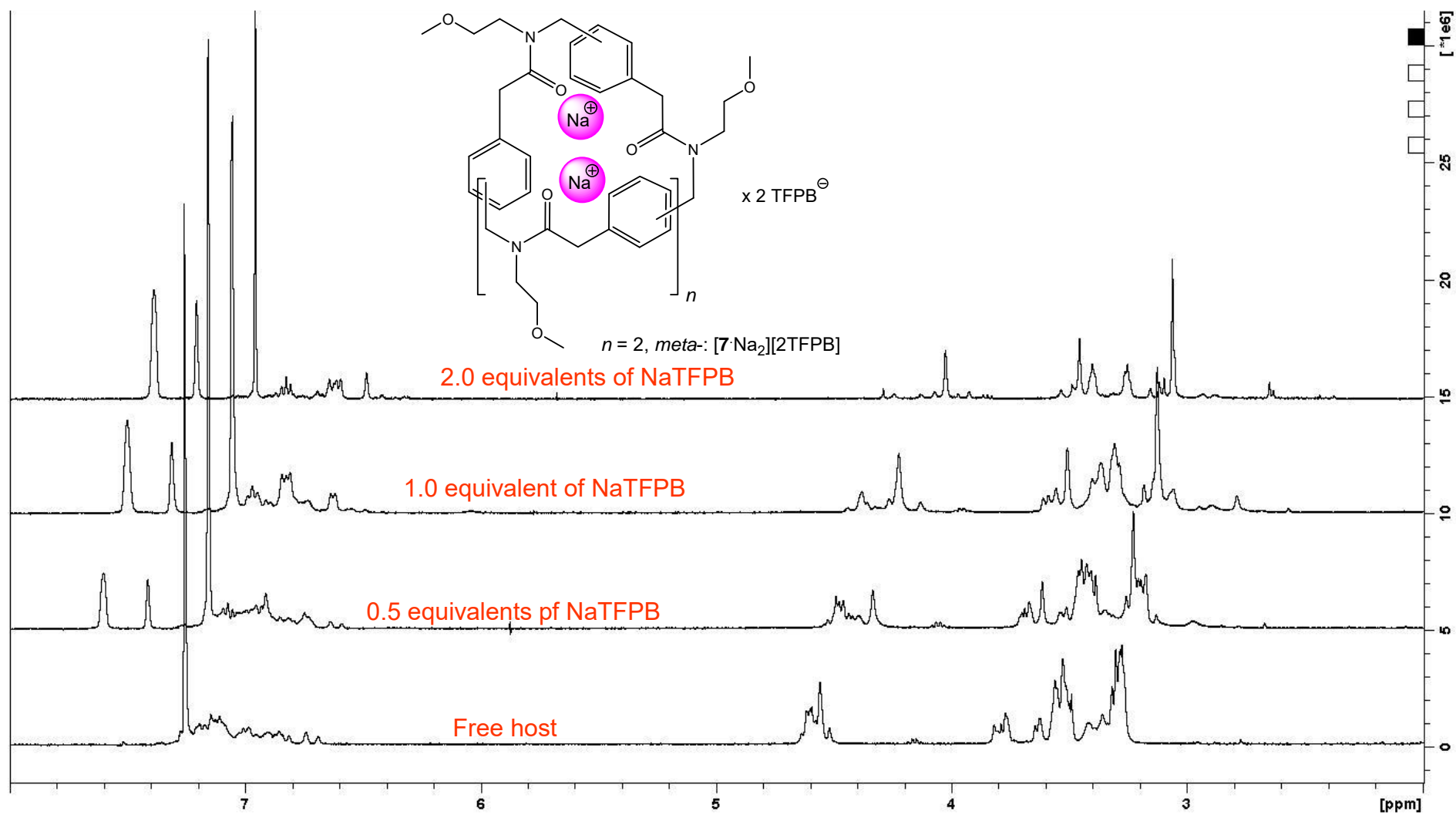
Figure S15. Titration experiment on compound 7 to give complex [7_2Na]^{2+} . ^1H -NMR: 600 MHz, CDCl_3 . Offset: 0.1 ppm.
