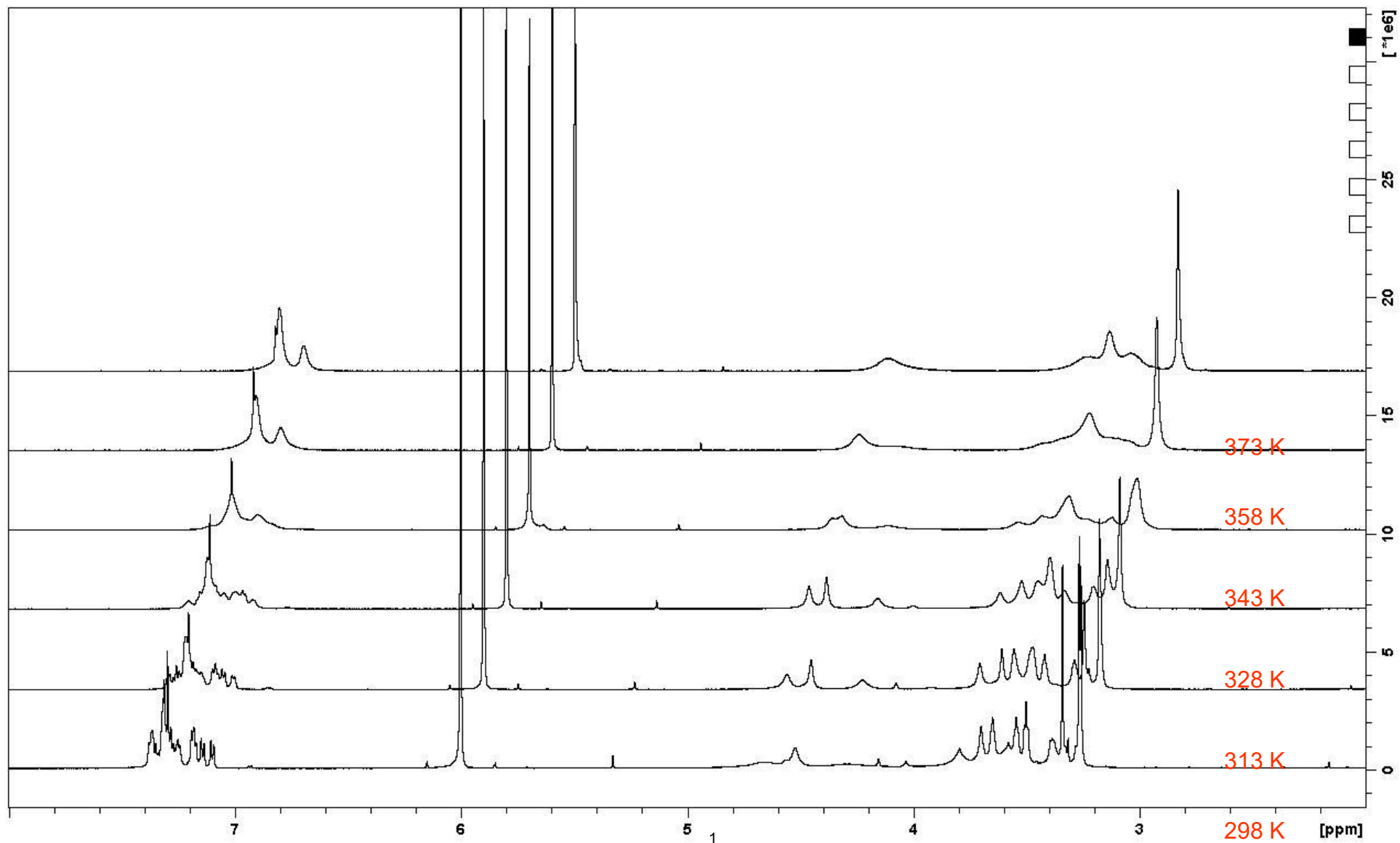
Figure S9. Variable temperature experiment on compound 5. ^1\text{H-NMR} : 600 MHz, TCDE.
