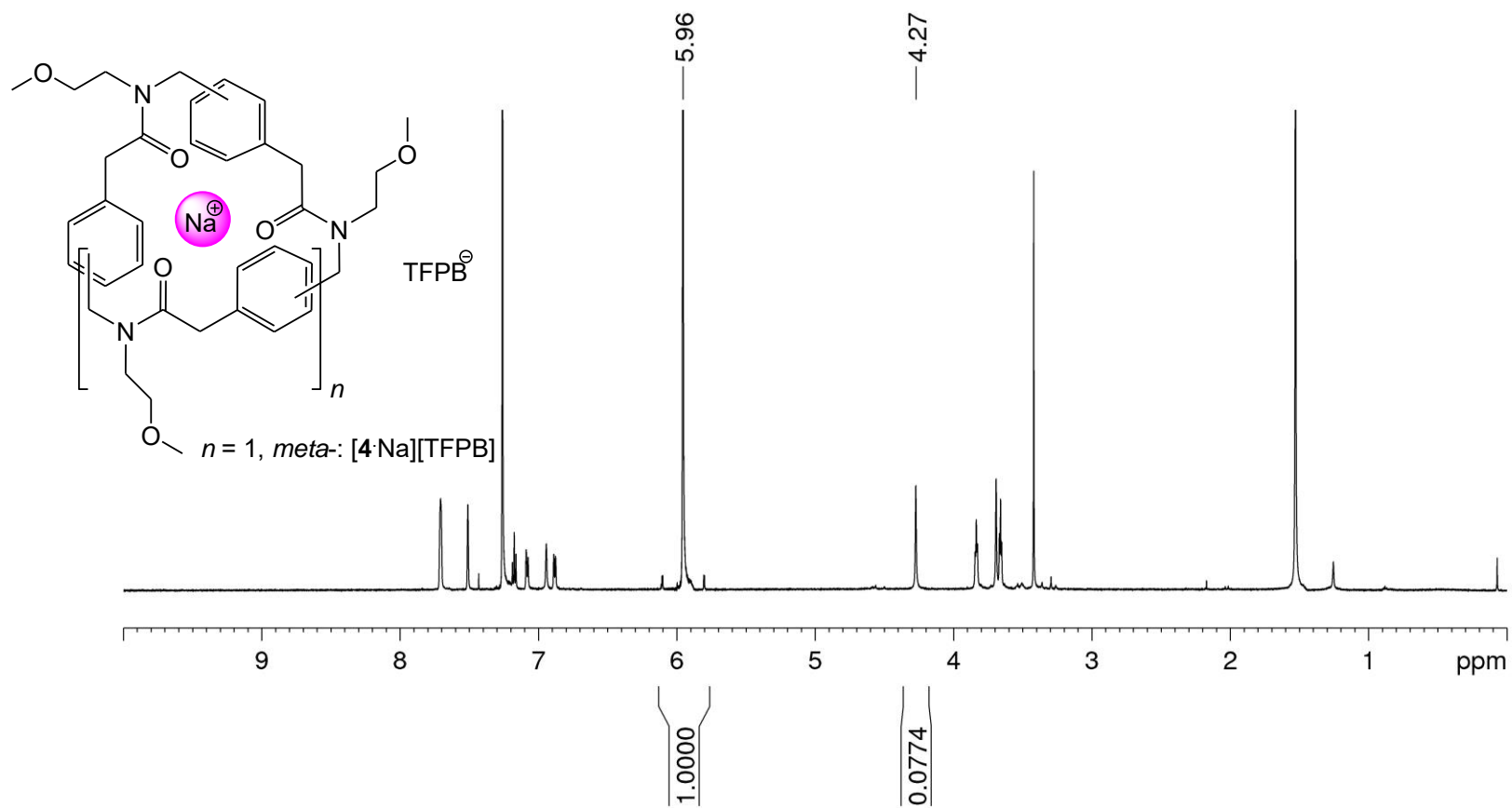
Figure S2. K_a evaluation for the complexed benzyloptoid [4 \cdot Na]^+ . ^1H -NMR: (600 MHz, CDCl_3 ).
