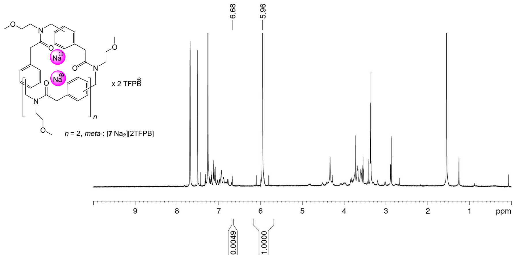
Figure S5. K_a evaluation for the complexed benzyloptoid [7 \cdot 2Na_2]^{2+} . ^1H -NMR: (600 MHz, CDCl_3 ).
