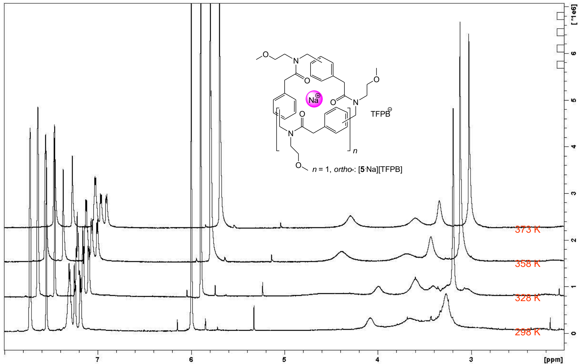
Figure S10. Variable temperature experiment on compound [\mathbf{5Na}]^+ . ^1\text{H-NMR} : 600 MHz, TCDE.
