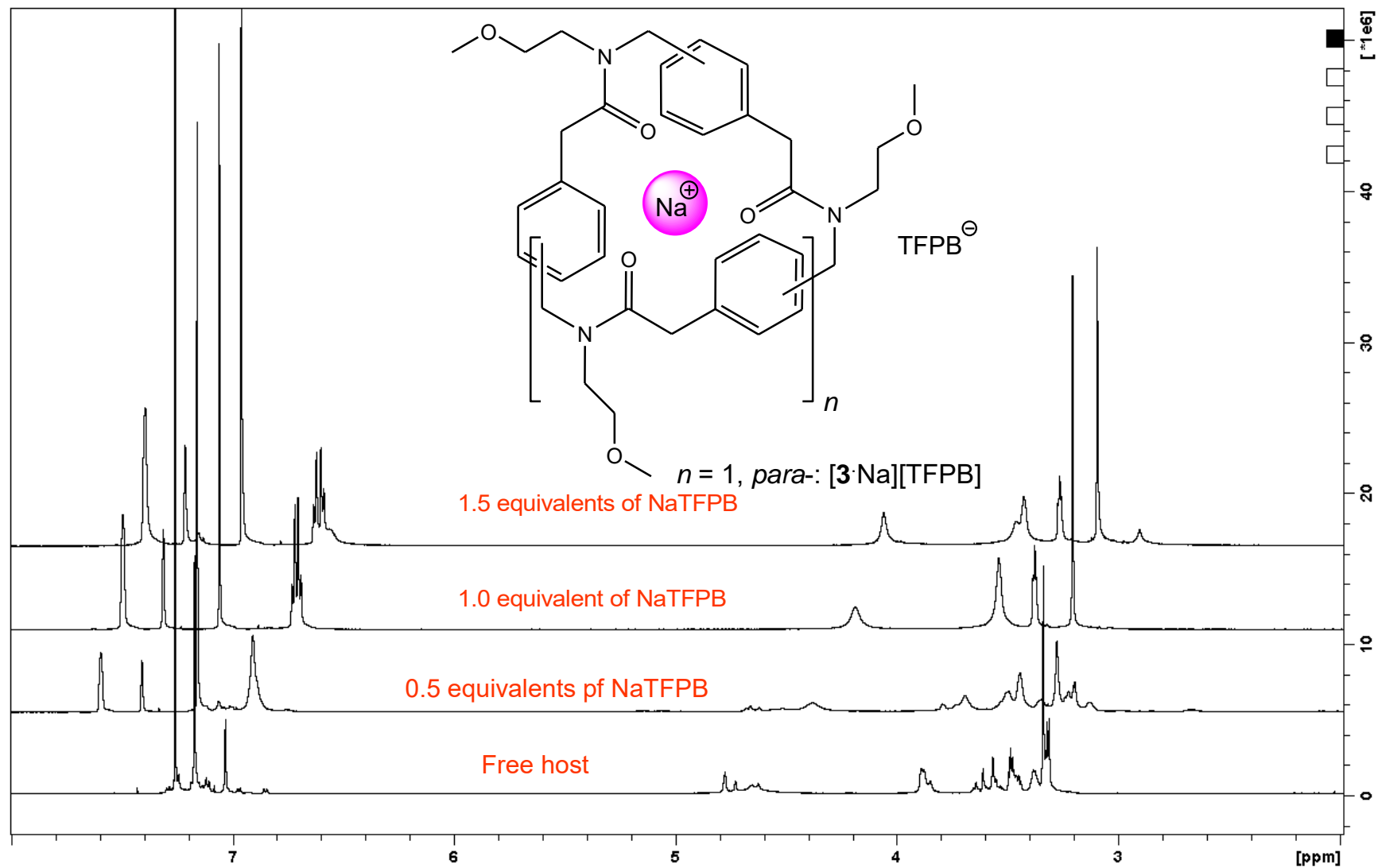
Figure S11. Titration experiment on compound 3 to give complex [\mathbf{3}\cdot\text{Na}]^+ . ^1\text{H-NMR} : 600 MHz, \text{CDCl}_3 . Offset: 0.1 ppm.
