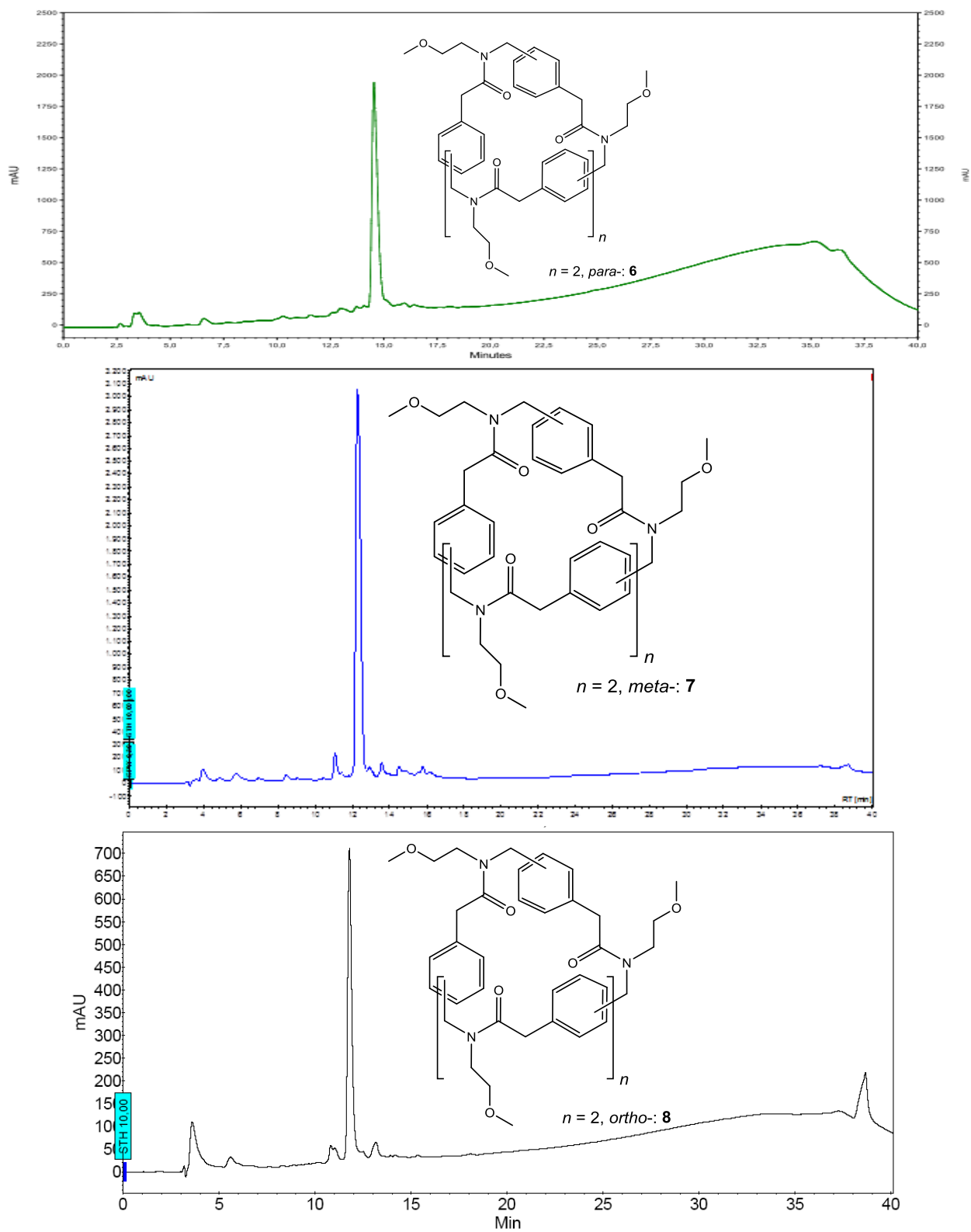
Figure S20: HPLC chromatogram of tetrameric cyclic 6-8 as crude mixture Conditions: 5 → 100% A in 30 min (A, 0.1% TFA in acetonitrile, B, 0.1% TFA in water); flow: 1 mL min -1 , 220 nm
