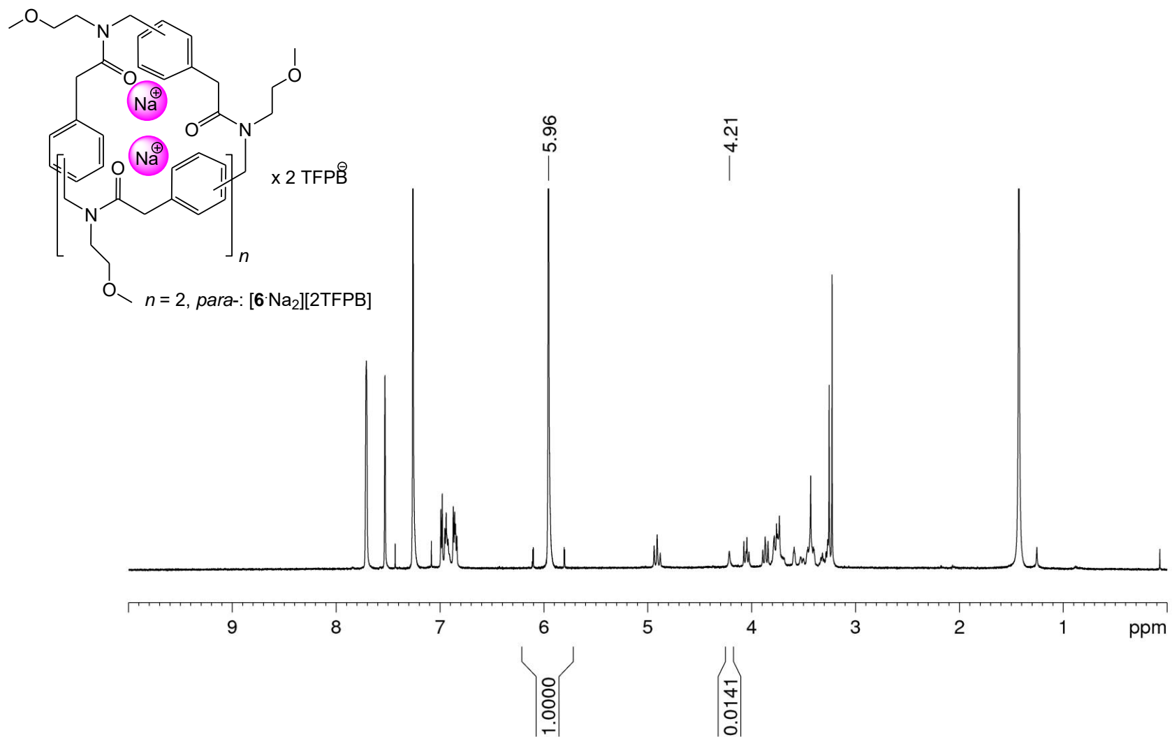
Figure S4. K_a evaluation for the complexed benzyloptoid [6 \cdot 2Na]^{2+} . ^1H -NMR: (600 MHz, CDCl_3 ).
