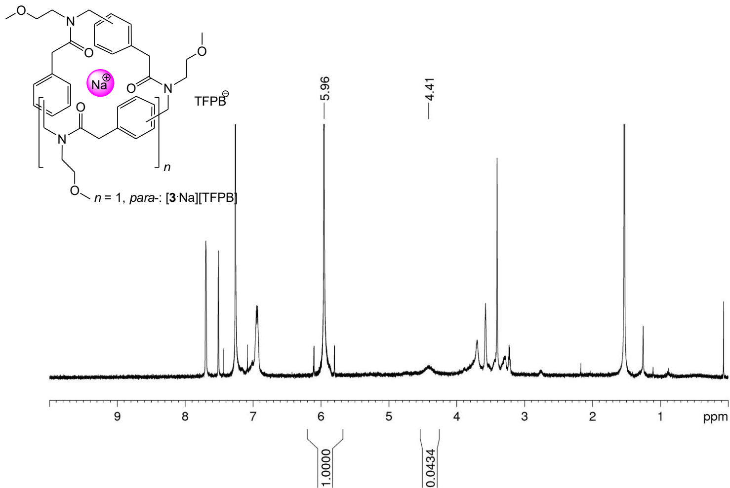
Figure S1. K_a evaluation for the complexed benzyloptoid [3-Na]^+ . ^1H -NMR: (600 MHz, CDCl_3 ).
