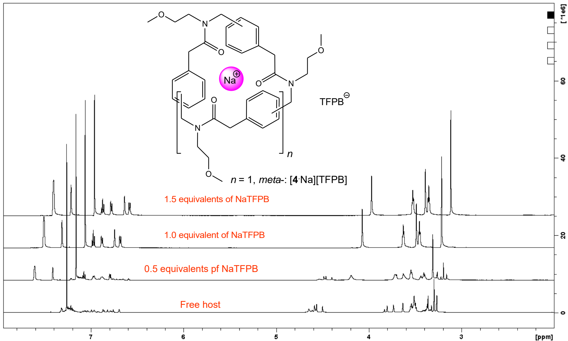
Figure S12. Titration experiment on compound 4 to give complex [4 \cdot \text{Na}]^+ . ^1\text{H-NMR} : 600 MHz, \text{CDCl}_3 . Offset: 0.1 ppm.
