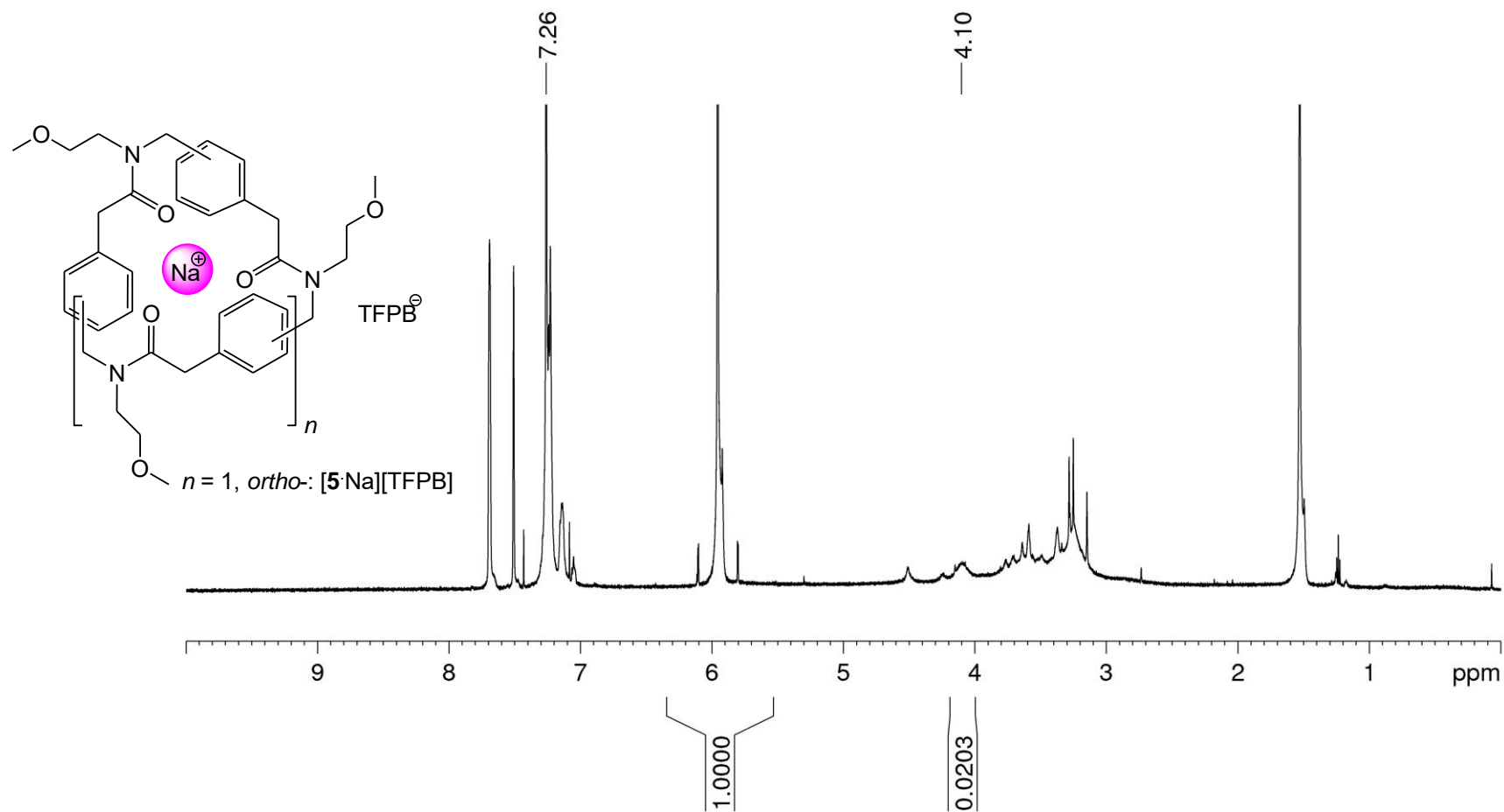
Figure S3. K_a evaluation for the complexed benzyloptoid [5\text{Na}]^+ . ^1\text{H-NMR} : (600 MHz, \text{CDCl}_3 ).
