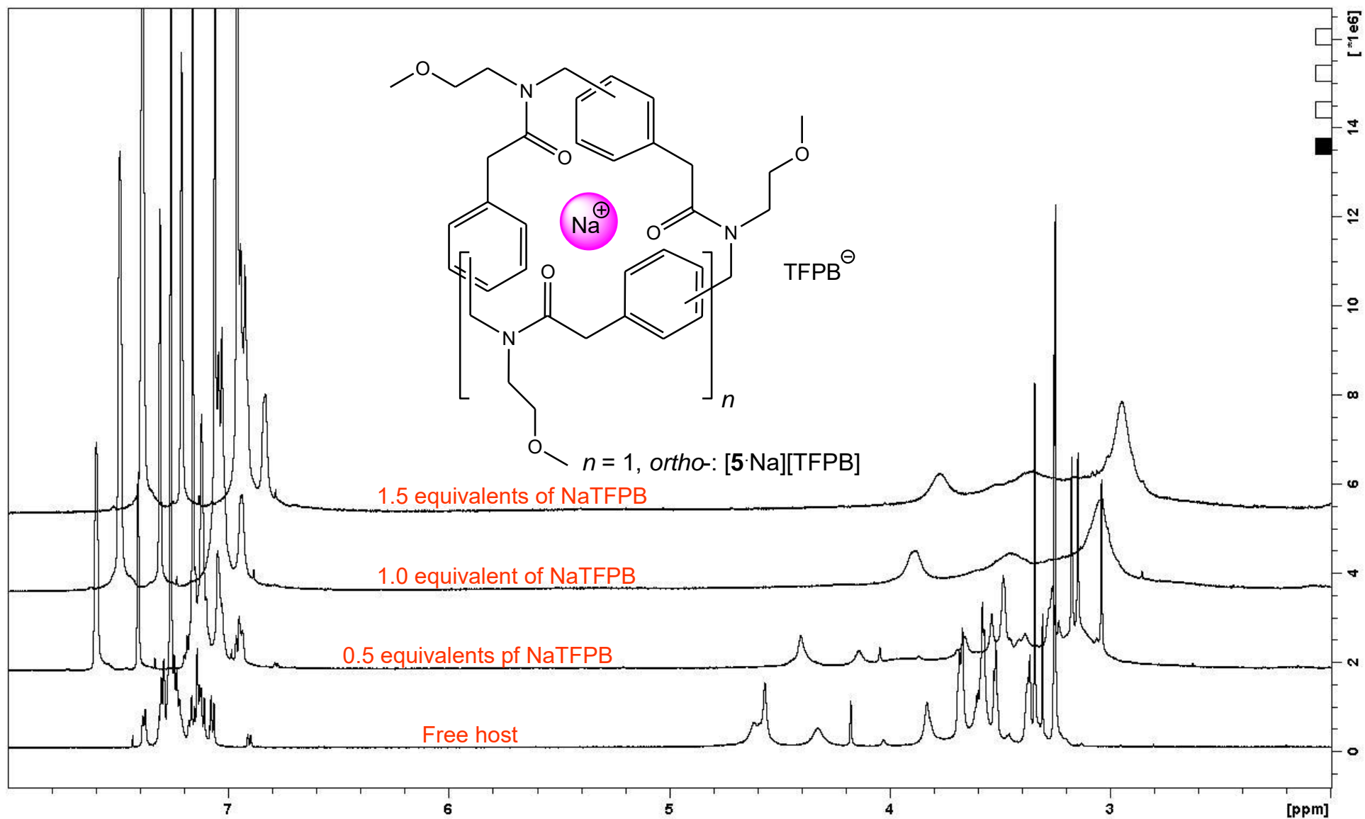
Figure S13. Titration experiment on compound 5 to give complex [5 \cdot \text{Na}]^+ . ^1\text{H-NMR} : 600 MHz, \text{CDCl}_3 . Offset: 0.1 ppm.
