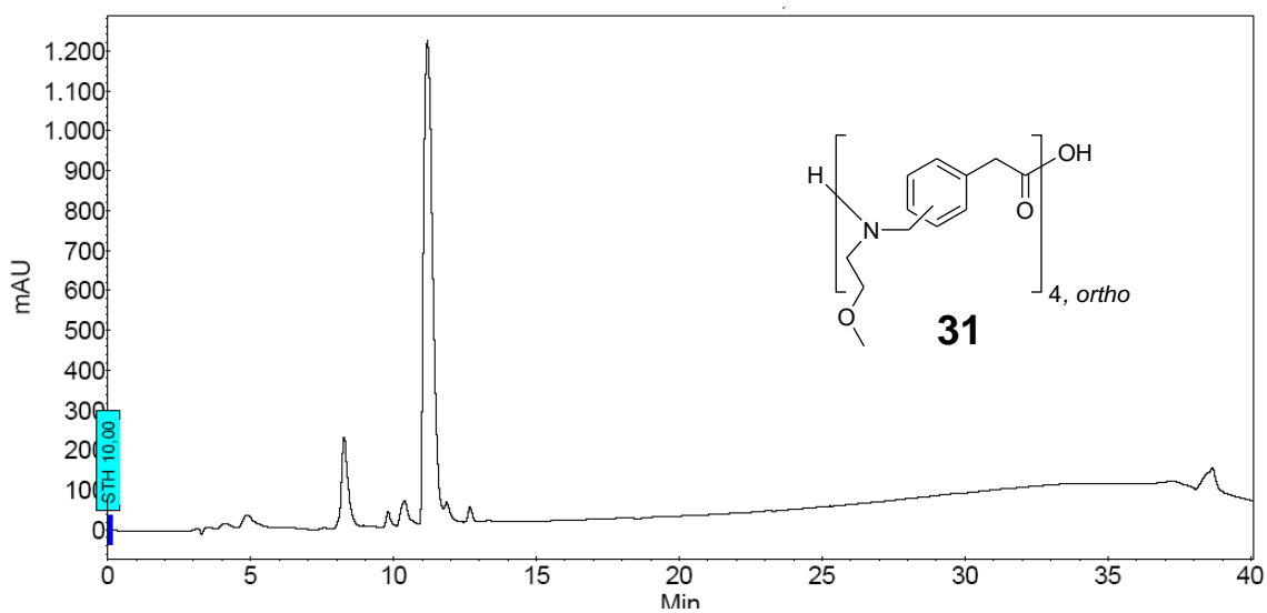
Figure S18: HPLC chromatograms of tetrameric linear 29-31 as crude mixture. Conditions: 5 → 100% A in 30 min (A, 0.1% TFA in acetonitrile, B, 0.1% TFA in water); flow: 1 mL min -1 , 220 nm.
