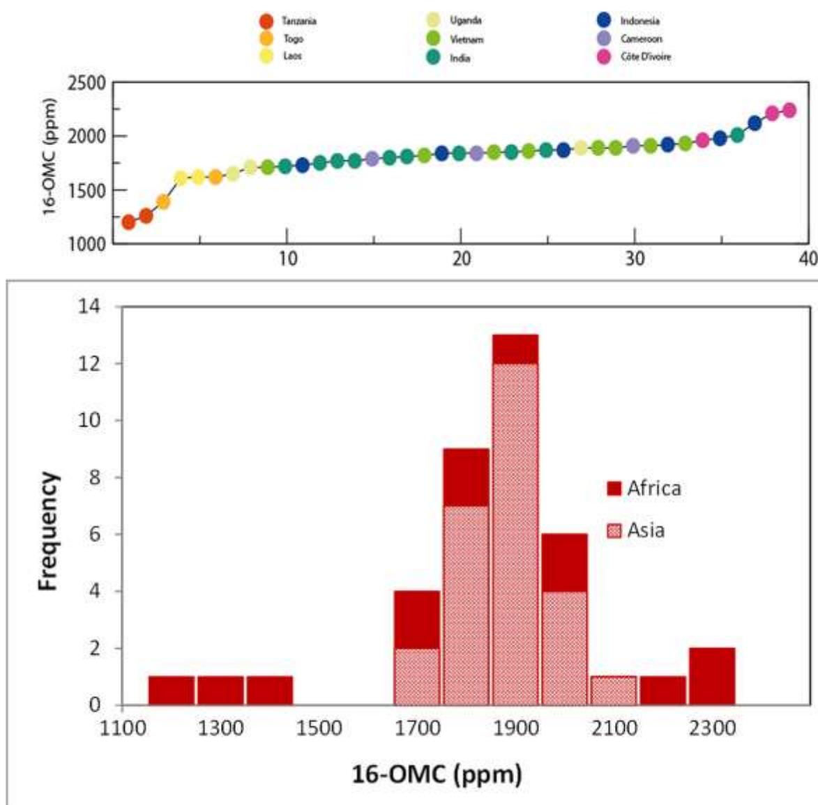
Figure 3 (top) Content of 16-OMC esters (expressed as 16-OMC free form) as determined by NMR for the 39 samples of roasted Robusta coffee. The geographical origin is indicated. (bottom) Histogram showing the frequency distribution of 16-OMC esters content for the Africa Robusta coffee samples (red) and for the subset originating from Asia (light red).
