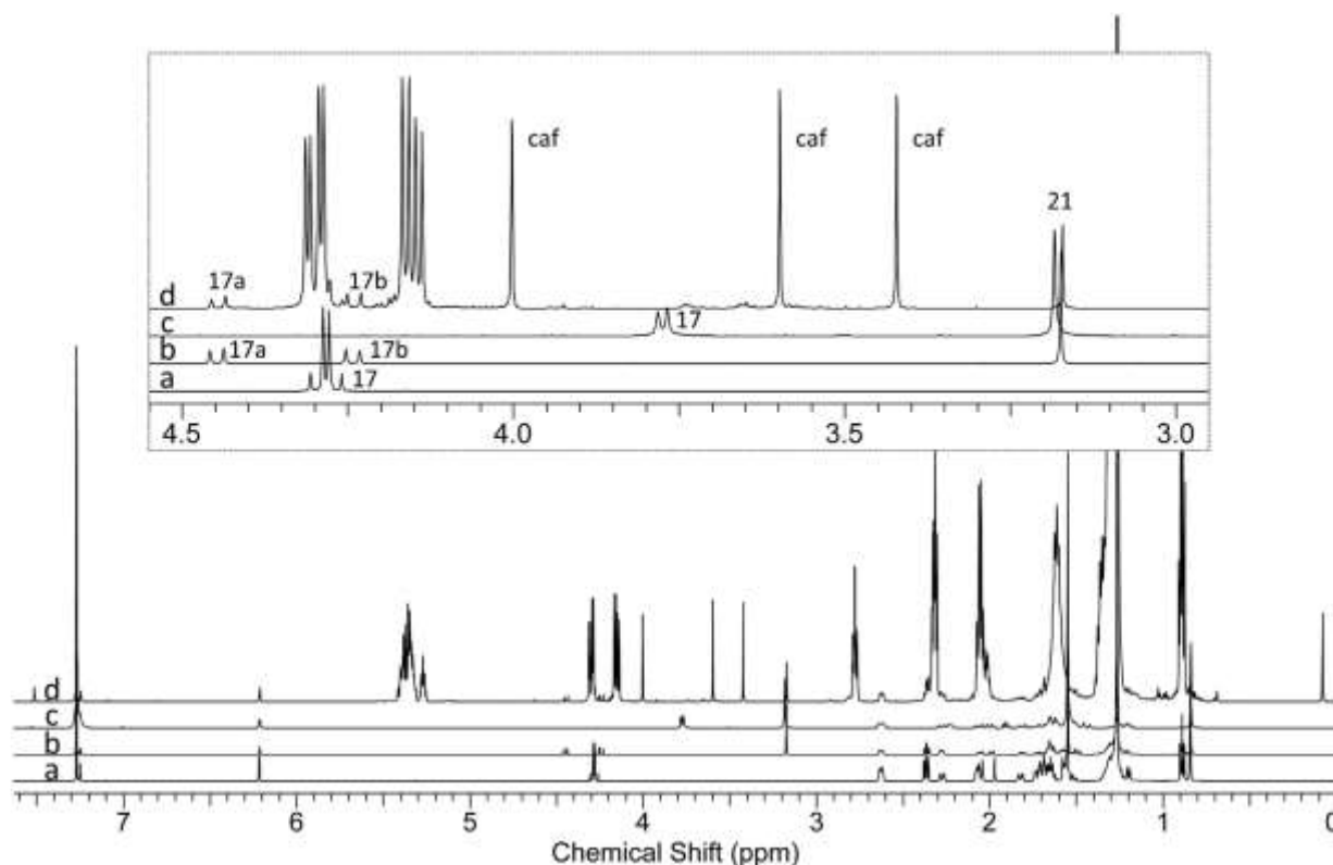
Figure 2 1 H NMR spectra of cafestol palmitate (a), 16-OMC palmitate (b), 16-OMC (c) and of the chloroform extract of a roasted Robusta coffee (d). The spectral region between 2.9 ppm and 4.6 ppm is enlarged in the insert
