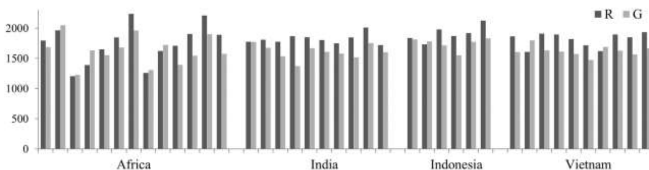
Figure 4 Content of 16-OMC (mg/kg) in roasted (R) and green (G) coffee samples.
