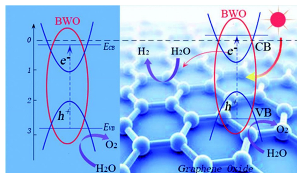
Figure 20. Schematic representation of the \text{Bi}_2\text{WO}_6 (left side) and the \text{Gr}-\text{Bi}_2\text{WO}_6 band edges energy level and the mechanism of the photocatalytic WS process. Reproduced from Ref. [161] with permission from The Royal Society of Chemistry.
