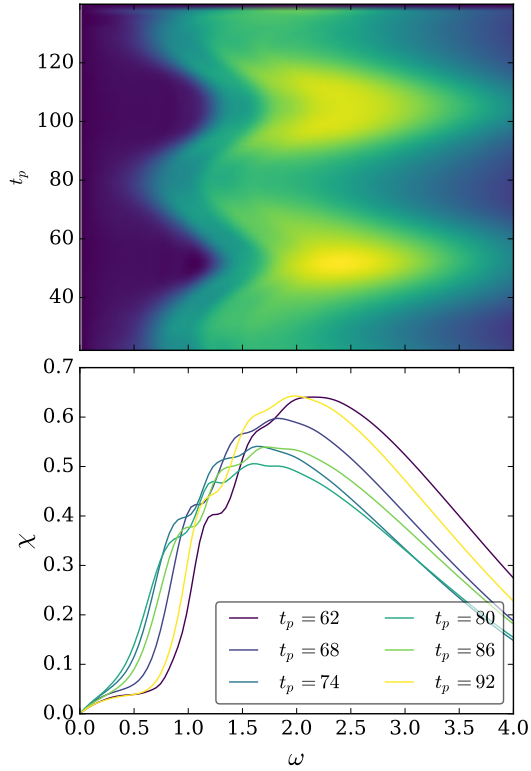
Figure 3.11: a) Out-of-equilibrium paramagnetic part of the optical susceptibility \chi^{\text{pm}}(t_p, \omega) as a function of frequency \omega and of time t_p . b) Out-of-equilibrium paramagnetic part of the optical susceptibility \chi^{\text{pm}}(t_p, \omega) as a function of frequency \omega for selected t_p .
