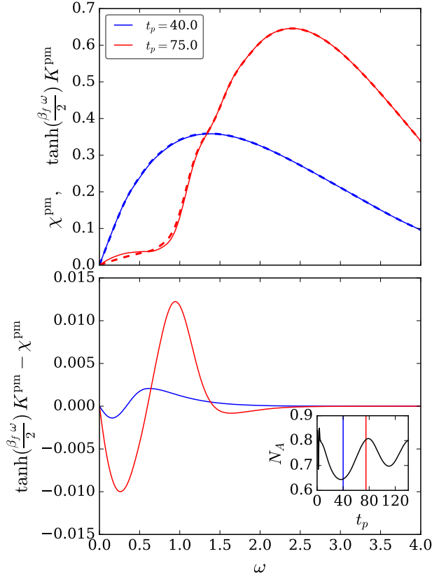
Figure 3.16: a) \text{Im}\chi^{\text{pm}}(t_p, \omega) (solid) and best-fit \tanh(\frac{\beta_f \omega}{2})K^{\text{pm}} (dashed) for t_p = 40 (blue) and t_p = 75 (red). b) Difference between the corresponding dashed and solid lines of panel a .
