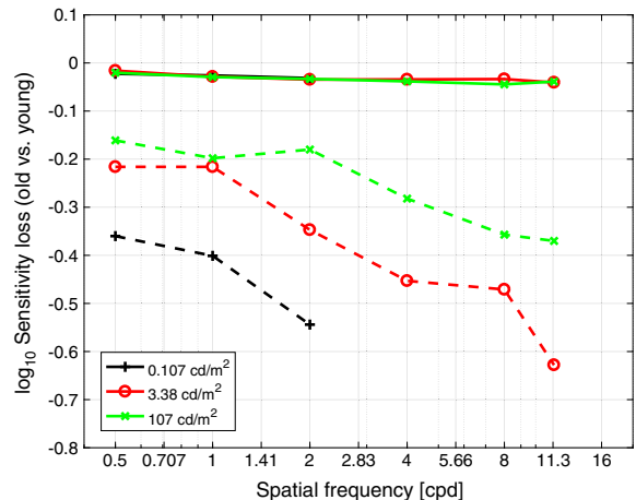
FIGURE 3 — The predicted loss of sensitivity due to disability glare (solid lines). The plotted values indicate the difference in sensitivity between elderly (mean 73 years) and young (mean 24 years) observers. Different line colors and markers denote different luminance levels. Note that disability glare has very small effect in sensitivity, which is almost identical for all luminance levels and almost independent of spatial frequency. The dashed lines show the measurements of Sloane et al. , 16 which indicate a much stronger drop in sensitivity for older observers and a significant variability of this drop with respect to both spatial frequency and luminance.
