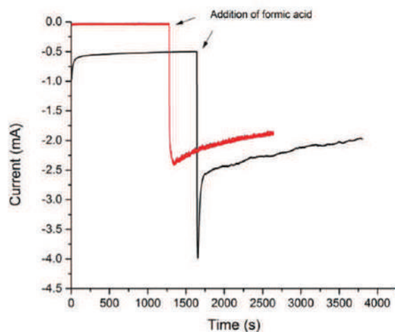
Fig. 4 Chronoamperometry of the GC electrode modified with the Pd@ \text{TiO}_2 /ox-SWCNHs at -0.2 \text{ V} (vs. RHE) in PBS at pH 6.5 under an Ar flow with the addition of formic acid (black line) and chronoamperometry of the Pd@ \text{TiO}_2 /ox-SWCNHs at -0.13 \text{ V} (vs. RHE) in \text{NaClO}_4 at pH 3.6 under an Ar flow with the addition of formic acid (red line). Quantity of formic acid added: 70 \mu\text{L} , final concentration of formic acid 0.23 M.
