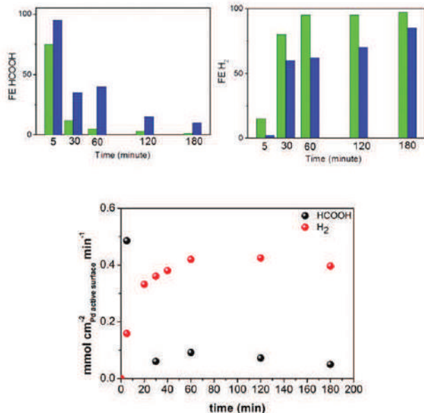
Fig. 5 Top: Faradaic efficiency in formic acid (left) and in hydrogen (right) over time at different times of the chronoamperometric experiments in PBS (green bars) and NaClO 4 (blue bars); bottom: rates of formation of H 2 and HCOOH by the Pd@TiO 2 /ox-SWCNHs in NaClO 4 electrolyte over three hour long electrocatalytic experiments.
