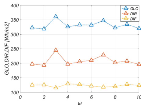
Fig. 2 – The mean yearly values of irradiance: Global, Direct and Diffuse on the horizontal plane
