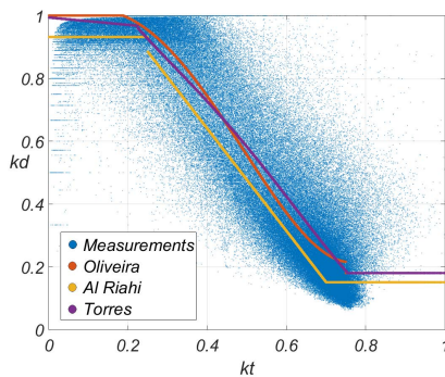
Fig. 4 – The Oliveira, Al Riahi, and Torres models
