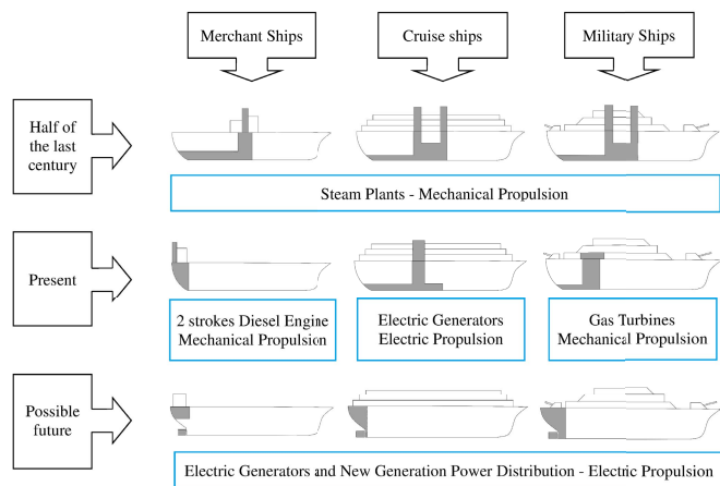
Fig. 1. Ship configuration [2].
