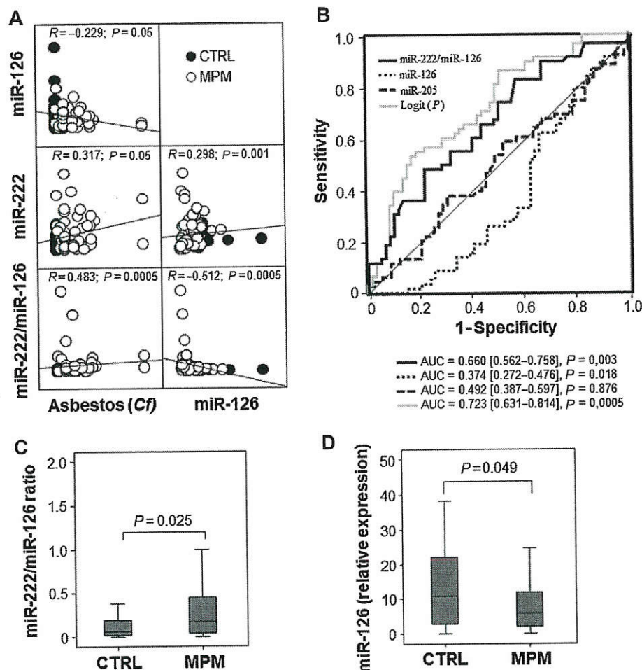
Figure 3. Relationship between asbestos fibers and miRNAs, and their performance to discriminate MPM from CTRL. Correlation between cumulative asbestos fibers (Cf) and miRNAs. Correlation coefficient ( R ) was determined using the Spearman test (A). ROC curve of miR-126, miR-222/miR-126 ratio and Logit ( P ) value in MPM and CTRL are documented. Area under the ROC curves (AUC) and 95% CI are shown (B). Distribution of miR-222/miR-126 ratio (C) and miR-126 (D) in MPM and CTRL group are presented. Significant differences were determined using Student t test.
