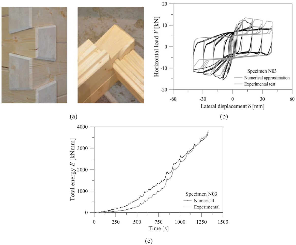
Fig. 10. ‘Tirol’ carpentry joint (‘N03’ type, in accordance with [3,23]). (a) Geometrical configuration and (b) FE calibration of its load-displacement cyclic behaviour, with (c) corresponding numerically and experimentally derived energies.
