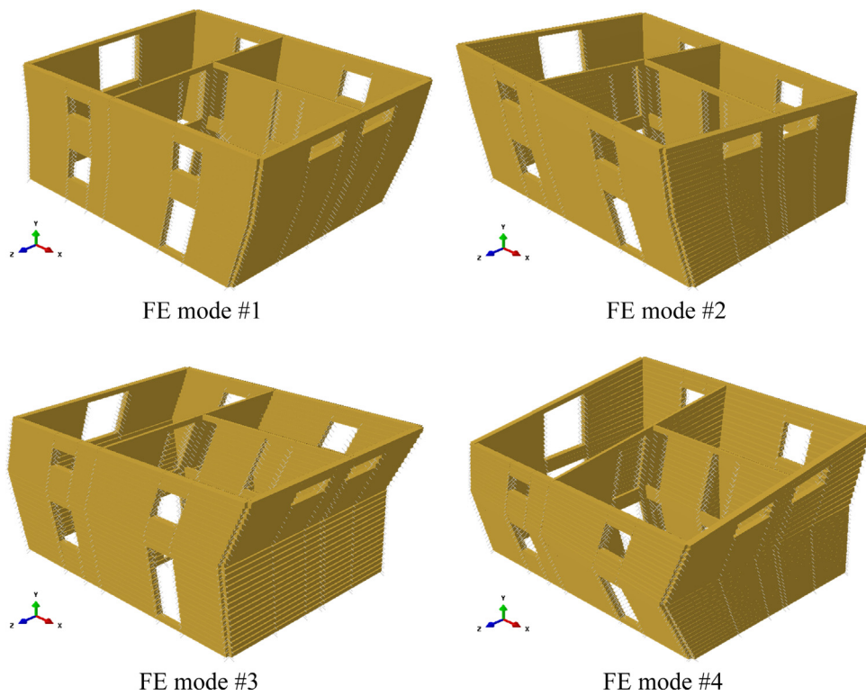
Fig. 5. Numerically predicted fundamental vibration shapes for the 'Rusticasa building' (ABAQUS).
