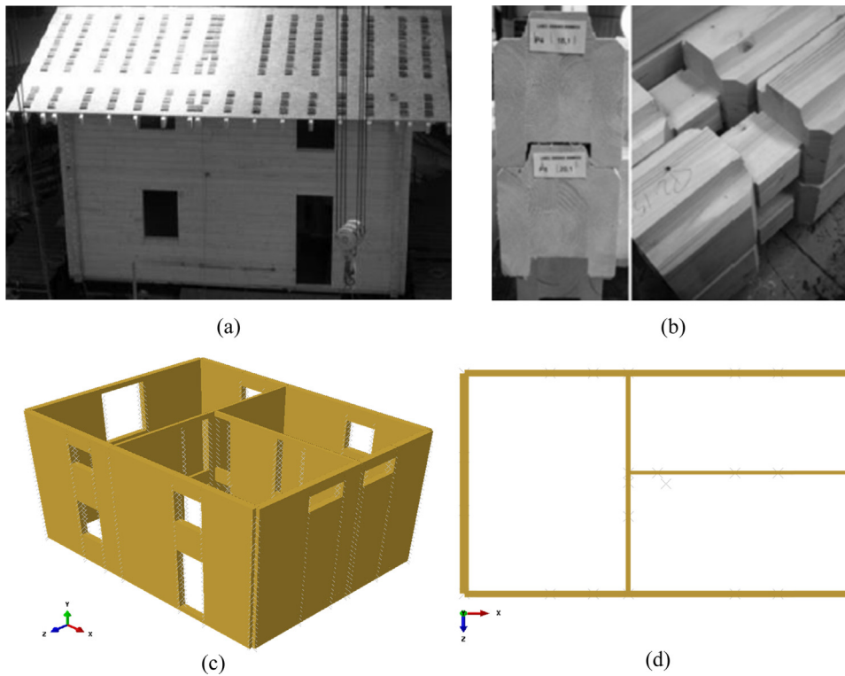
Fig. 4. FE modelling of the ‘Rusticasa building’. (a) Overview of the experimental full-scale specimen and (b) detail of timber logs [18,19], with (c) extruded 3D and (d) plan views of the corresponding FE model (ABAQUS).
