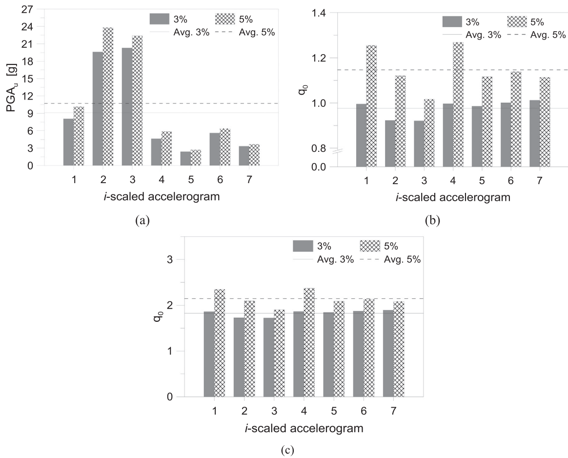
Fig. 14. q-factor estimation for the B01 case study building. (a) PGA_{u,i} and (b) q_0 -factor values, according to Method 1; and (c) q_0 -factor values, based on Method 2 (ABAQUS).
