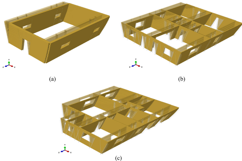
Fig. 8. Fundamental vibration modes for the (a) B01, (b) B02 and (c) B03 buildings (extruded 3D view, ABAQUS).
