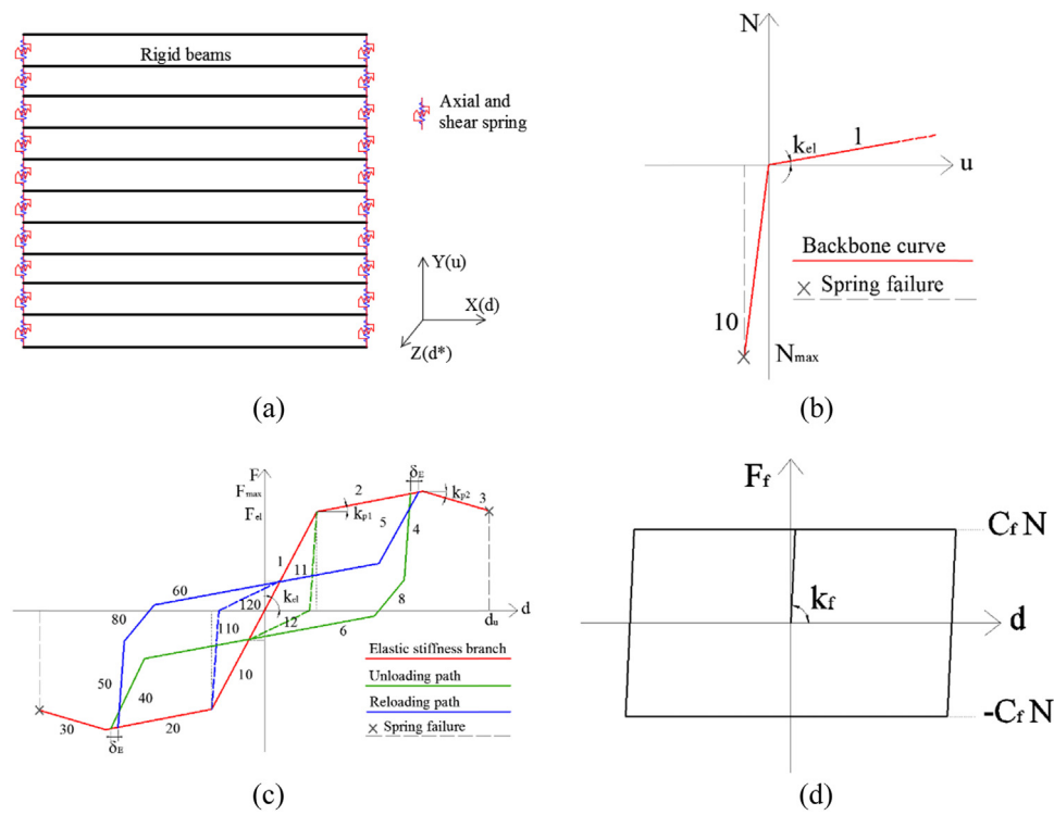
Fig. 3. FE assembly of the typical log-house system. (a) Schematic view of a single log-wall, with constitutive laws in springs representative of (b) axial DOF, (c) shear DOFs and (d) friction.
