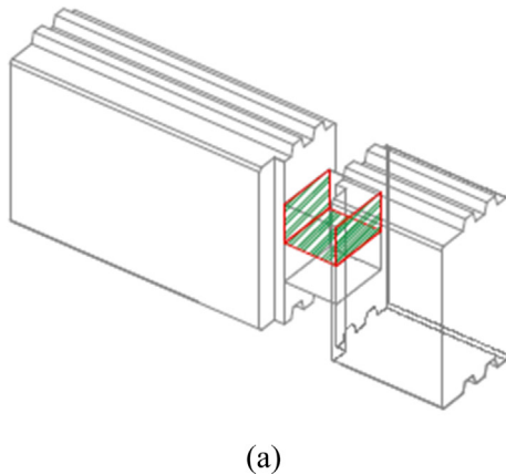
Fig. 13. Reference resisting surfaces for a N01 type carpentry joint, with evidence of (a) shear or (b) compressive failure mechanisms.
