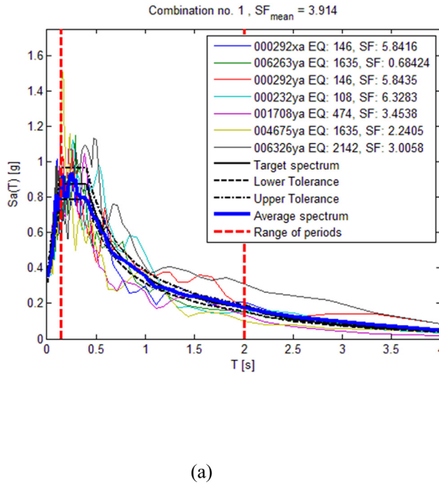
Fig. 9. (a) Reference set of natural seismic records obtained from REXEL v.3.5, with (b)-(c) typical deformed configuration of the B03 building under seismic events (0.35 g), scale factor: 5000, ABAQUS).
