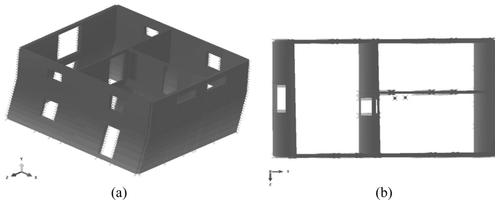
Fig. 6. Typical deformed configuration of the 'Rusticasa building' FE-model under the 1979 Montenegro seismic record (0.28 g), scale factor: 500). (a) Extruded 3D view and (b) top view (ABAQUS).
