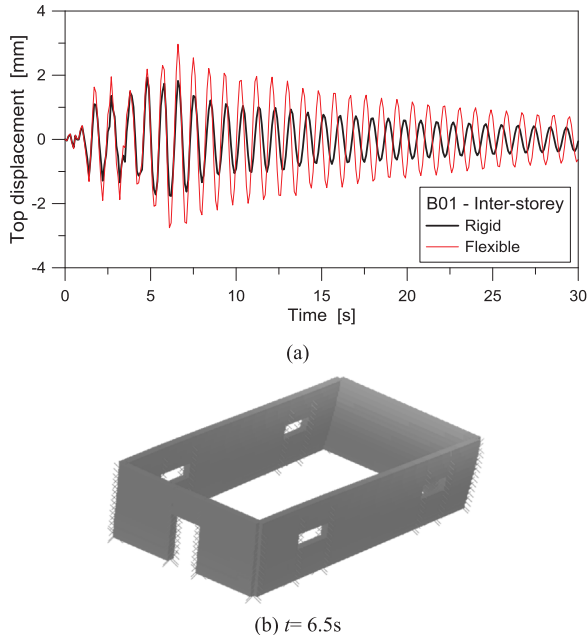
Fig. 12. Effect of in-plane fully rigid or flexible diaphragms on the seismic performance of the B01 case study building. (a) Monitored top displacement as a function of time, with (b) corresponding (extruded) 3D view for the B01 building with flexible floor (scale factor: 300, ABAQUS).
