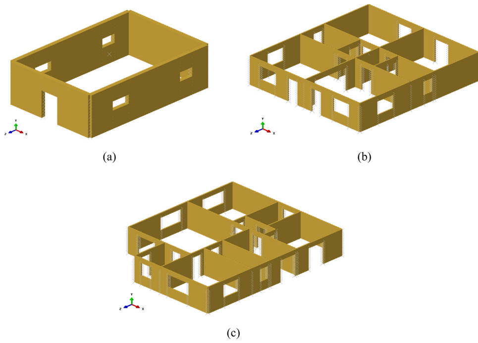
Fig. 7. 3D models of the log-house buildings investigated through the parametric study (extruded 3D view, ABAQUS). Case studies labelled as (a) 'B01', (b) 'B02' and (c) 'B03' buildings.
