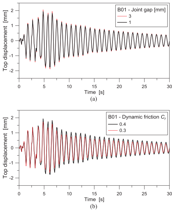
Fig. 11. Effect of (a) joint gap and (b) dynamic friction coefficient on the seismic performance of the B01 case study building (PGA = 0.35 g), in terms of time-top displacement history (ABAQUS).
