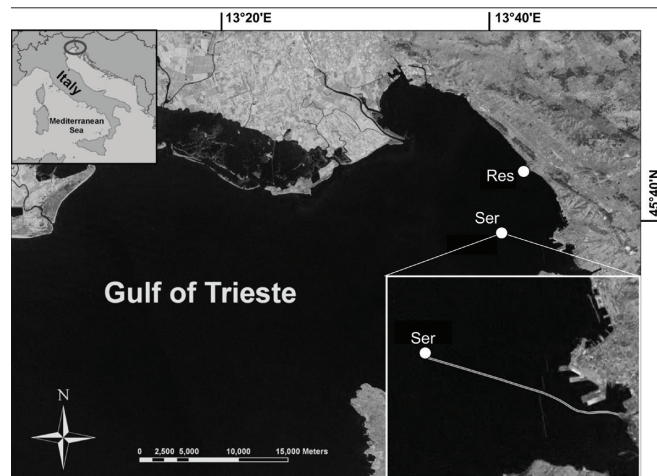
Fig. 1: Study area and location of the Ser (Servola) and Res (Riserva Naturale Marina di Miramare) stations. The Servola pipeline is evidenced in the enlarged square.
