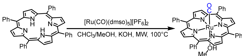
Scheme 2. Ruthenation of TPP with the chloride-free Ru(II) carbonyl precursor [Ru(CO)(dmsO) 5 ][PF 6 ] 2 ( 5 ). See text for reaction time and yields.
