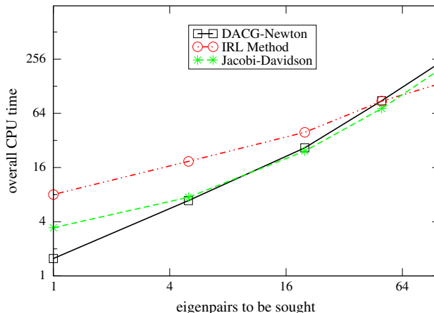
Figure 4. CPU times in seconds versus number of eigenpairs for DACG–Newton, Jacobi–Davidson, and implicitly restarted Lanczos (IRL) methods. Matrix monte-carlo .
