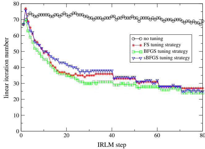
Figure 2. Number of iterations for the preconditioned conjugate gradient solution of the inner systems with implicitly restarted Lanczos in the solution of the mat268515 test problem. Comparison against the fixed preconditioner of CASE #1 and the three tuned preconditioners with l_{\max} = 20 .
