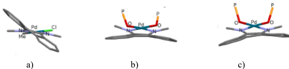
Figure 9. Fragments cut out from the structures of: a) 2b ; b) trimer 2c ; c) dimer 1c . They put in evidence the decreased twisting of the Ar-BIP ligand on passing from the mononuclear to the multinuclear molecules.
