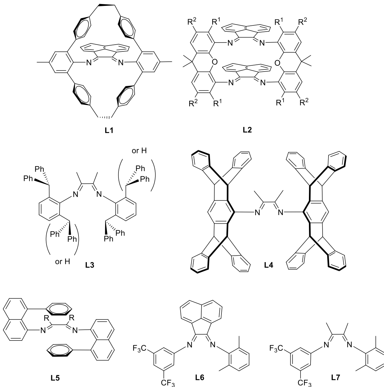
Chart 2. Examples of reported \alpha -dimine ligands.
