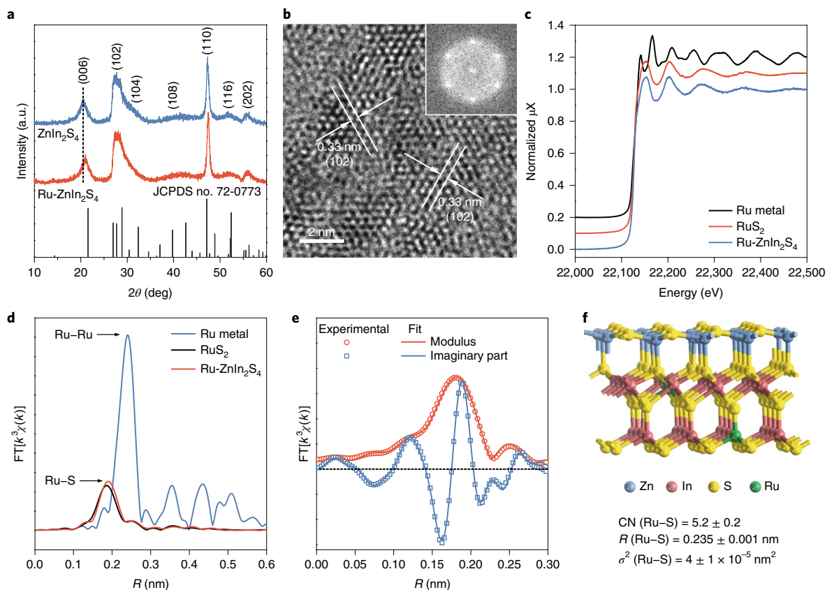
Fig. 2 | Characterization of the Ru-ZnIn 2 S 4 photocatalyst. a , XRD patterns of Ru-ZnIn 2 S 4 and undoped ZnIn 2 S 4 , indexed accordingly to the hexagonal P6 3 mc space group (JCPDS card no. 72-0773). The dashed line highlights the shift of the pattern induced by Ru doping. b , Representative high-resolution TEM image of Ru-ZnIn 2 S 4 , with arrows highlighting the (102) interplanar distance. Inset, the corresponding FFT of Ru-ZnIn 2 S 4 . c , Stacked XANES spectra of Ru-ZnIn 2 S 4 , Ru metal and RuS 2 recorded at the Ru K edge. \mu\text{X} is the X-ray absorption. d , Extracted k^3\chi(k) EXAFS signals of Ru-ZnIn 2 S 4 , Ru metal and RuS 2 . e , Fit of the FT k^3\chi(k) of the EXAFS signals of Ru-ZnIn 2 S 4 at the Ru K edge. f , Schematic of the Ru-ZnIn 2 S 4 structure and the fitting results of Ru-S coordination.
