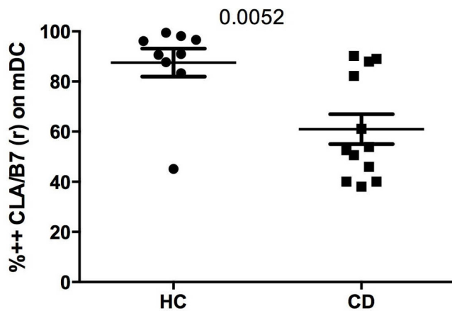
Figure 1: CLA/β7 double positive expression on mDC in Crohn's disease and healthy controls
