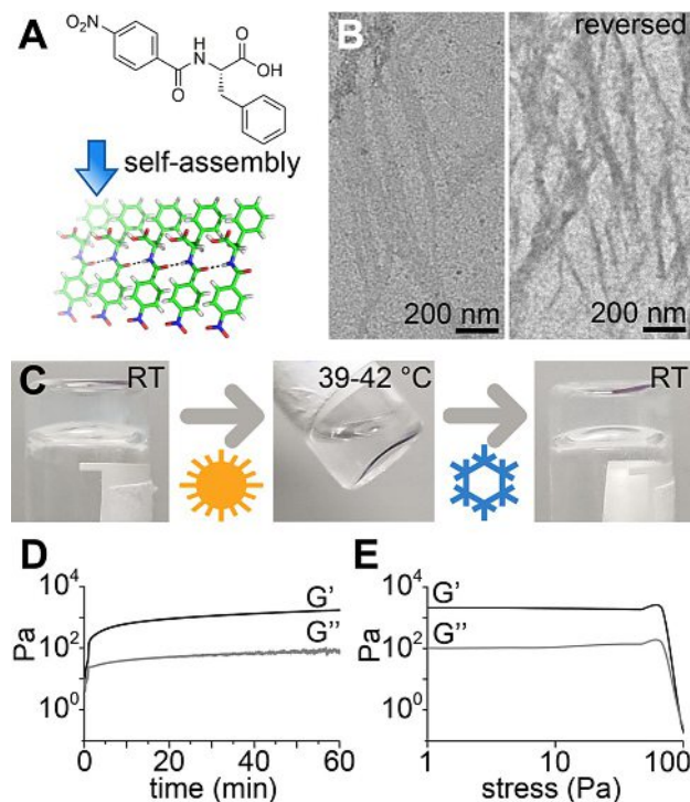
Figure 1. A) N -(4-Nitrobenzoyl)-Phe self-assembles into parallel displaced stacks held together by hydrogen bonding ( d = 3.1 \text{ \AA} ) between the amide groups, as revealed by single-crystal XRD data. B) TEM images reveal low-contrast bundles of fibrils as thin as 5 nm, which are present also in the thermoreversed gel (right). C) The 20 mM hydrogel is transparent and thermoreversible within a range compatible with physiological conditions. D,E) Rheology time (D) and stress (E) sweeps show rapid gelation kinetics with plateau reached within 1 hour and high resistance of the gel with failure occurring at nearly 100 Pa.
