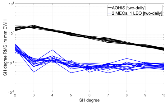
Fig. 9. Degree RMS of 2-daily gravity field solutions resolved up to SH degree 10. The full AOHIS signal is included in the observations, and recovered in the retrieval process. For details see text.
