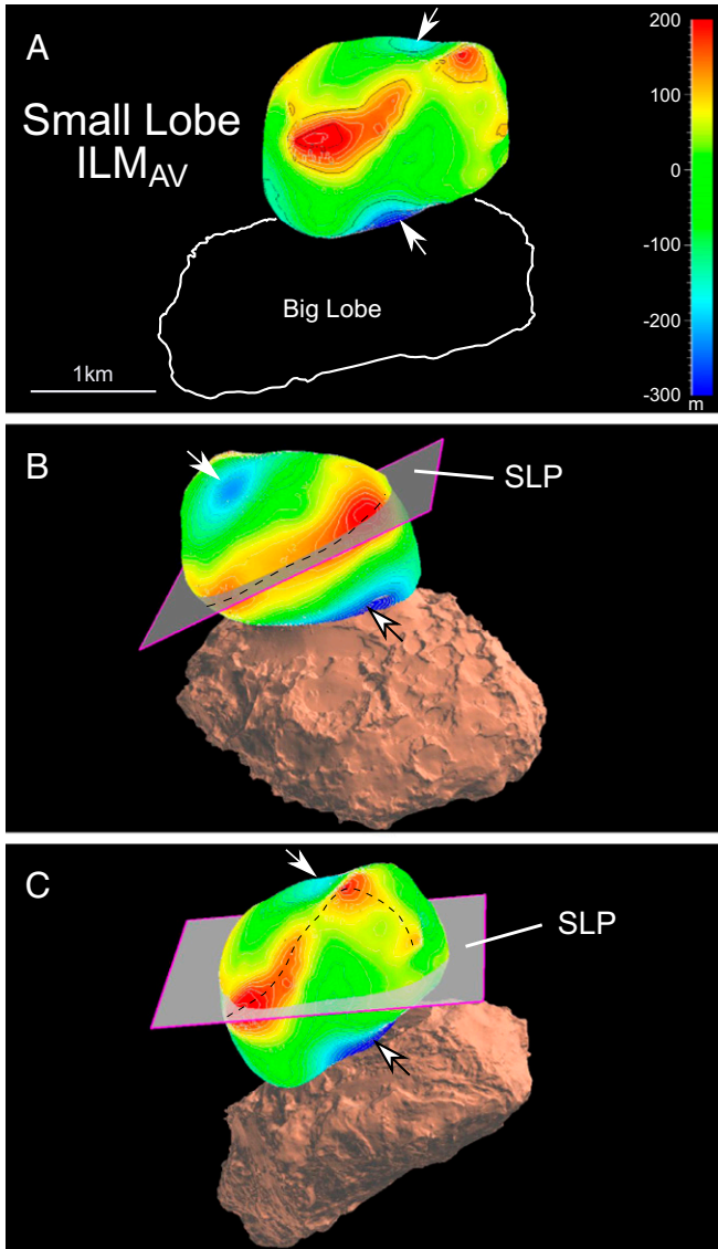
Fig. 3. Comparison between the ILM_{AV} and the EM_{AV} models of the Small Lobe. ILM_{AV} is colored in function of its distance from EM_{AV} . Negative differences (blue) correspond to areas where the ILM_{AV} is located in internal position with respect to EM_{AV} . Positive differences (red) correspond to areas where the ILM_{AV} is external with respect to the EM_{AV} . Arrows mark the areas with negative differences (blue color) located in antipodal position on the Small Lobe ILM_{AV} that are compatible with compression that occurred at the impact between two lobes having roughly ellipsoidal layered structure. (A) Small Lobe's ILM_{AV} shell with differences from EM_{AV} shell. (B) View of the northern hemisphere of the Small Lobe ILM_{AV} shell. SLP is a plane that best fits the maxima of the positive-differences ridge surrounding the ILM_{AV} . The ridge (black dashed line) on the northern hemisphere lays on SLP. (C) View of the southern hemisphere. Here, the ridge (black dashed line) does not lay on SLP and is asymmetrically folded.
