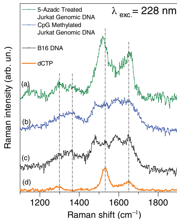
FIGURE 6 UVRR spectra of 5-azadact treated Jurkat genomic hypo -methylated gDNA, 0.10\text{ mg/mL} (green), CpG Jurkat genomic hyper -methylated gDNA 0.10\text{ mg/mL} (blue), B16 cell extracted DNA 0.10\text{ mg/mL} (black), dCTP (yellow) aqueous solutions; collected by using an excitation wavelength of 228\text{ nm} . Vertical dotted lines are guide for the eyes. gDNA, genomic DNA; UVRR, ultraviolet resonant Raman
