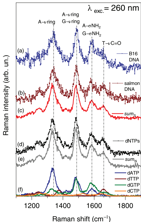
FIGURE 3 UVR spectra at 260 nm of: (a) gDNA extracted from B16 cells 0.10 mg/mL, (b) salmon sperm gDNA 0.10 mg/mL, (d) dNTP mix aqueous solution, (f) dATP (blue), dGTP (green), dCTP (yellow) and dTTP (red) aqueous solutions. The curves (c), and (e), represent the sum_N and sum_S curves, calculated as explained in the text. Spectral intensities of (a), (b), (c), (d), and (e), are normalized to the 1350\text{ cm}^{-1} intensity. Spectral intensities of (c), have been normalized to the \text{SO}_4^{2-} peak at 981\text{ cm}^{-1} . Normalizations have been carried out before the solvent contribution subtractions. Vertical dotted lines are guide for the eyes. dNTP, deoxynucleoside triphosphates; gDNA, genomic DNA; UVR, ultraviolet resonant Raman
