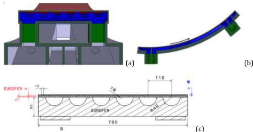
Fig. 6. CAD model images of the SL illustrating the poloidal (a) and toroidal (b) cross sections and schematic drawing of the poloidal section showing the dimensions (c).
