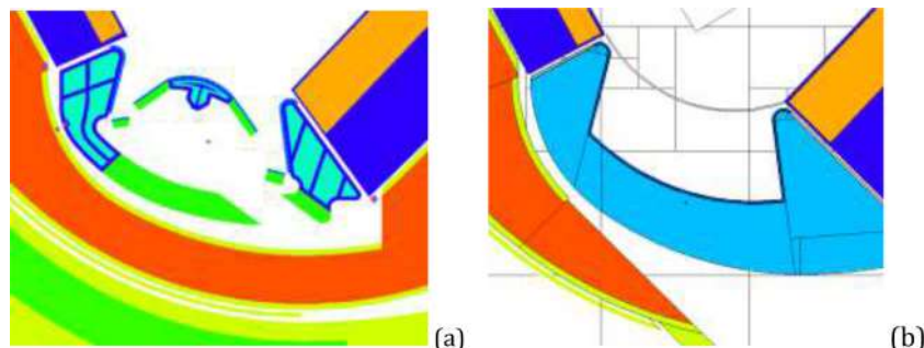
Fig. 10. Divertor region of the global MCNP model of the HCPB DEMO plant
