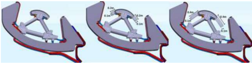
Fig. 4. Three different variants of divertor dome design: cap only (left), with a small (middle) and large wing extension (right), respectively.
