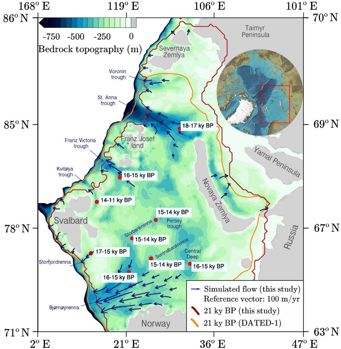
Fig. 1. Bathymetric map of the Barents and Kara seas, based on the International bathymetric chart of the Arctic Ocean (IBCAO) (Jakobsson, 2014) and interpolated in the 20 km horizontal resolution ice sheet model grid. The DATED-1 (Hughes et al., 2016) (dark yellow line) and simulated (this study, dark red line) BSIS extent during the LGM are shown. Blue arrows indicate the simulated (this study) ice velocities during the LGM (velocities lower than 45 m/yr masked out), whereas red dots indicate the location of the grid points used to estimate the individual ice streams deglaciation timing (Fig. 11). The time intervals for each location refer to its deglaciation timing range between the DATED-1 (Hughes et al., 2016) minimum and maximum reconstructions. (For interpretation of the references to color in this figure legend, the reader is referred to the Web version of this article.)
