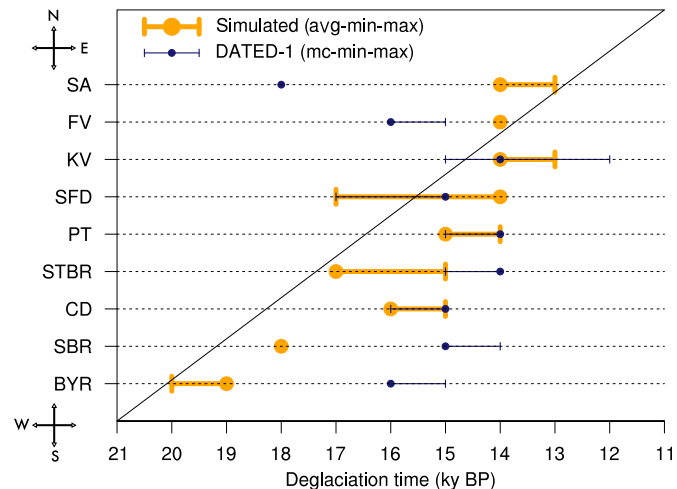
Fig. 11. Simulated (orange dots and lines) and DATED-1 (dark blue dots and lines) deglaciation timing for the individual ice streams shown in Fig. 1. Dots represents the deglaciation timing in the average simulated scenario and DATED-1 most-credible reconstruction, whereas lines indicate the deglaciation timing in the minimum and maximum simulated and DATED-1 scenarios. As shown by the black arrow, the ice streams are ordered on the y-axis from south-west (SW) to north-east (NE). BYR = Bjørnøyrenna, SBR = Sentralbankrenna, CD = Central Deep, STBR = Storbankrenna, PT = Persey Trough, SFD = Storfjordrenna, KV = Kvitøya Trough, FV = Franz Victoria Trough, SA = St. Anna Trough. (For interpretation of the references to color in this figure legend, the reader is referred to the Web version of this article.)
