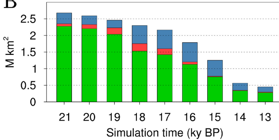
Fig. 10. (A) Time-slice evolution of the model-data agreement between the min-max-avg simulated scenarios and the DATED-1 min-max-mc reconstruction between 21 and 13 ky BP, shown every 1000 years. The green area indicates region where there is model-data agreement, whereas red and blue areas indicate regions of model-data underestimation and overestimation, respectively (see Subsection 3.6 ). (B) Model-data agreement, underestimation and overestimation total area at each time slice shown in (A) and with the same color legend. (For interpretation of the references to color in this figure legend, the reader is referred to the Web version of this article.)
