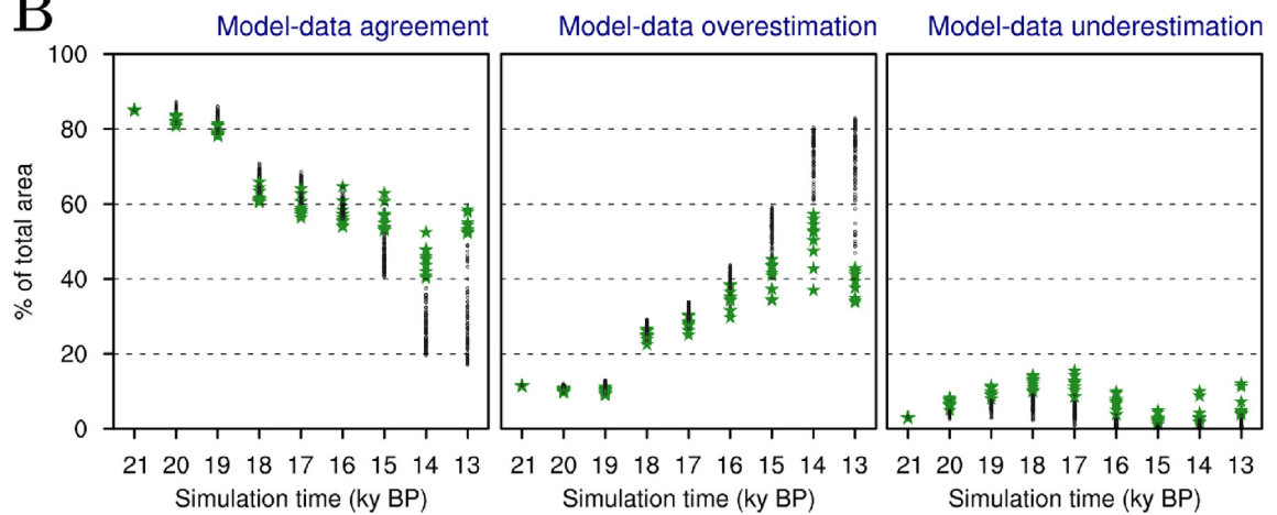
Fig. 4. (A) Evolution of the simulated BSIS at 1000 yr time-slices between 21 and 13 ky BP for all the simulations in the ensemble (black lines). Admissible simulations (see Subsection 3.6) are shown in green. In the background, the DATED-1 min-mc-max scenarios are shown in light blue. (B) Simulated/DATED-1 ice sheet area agreement (left panel), overestimation (central panel) and underestimation (right panel) for all the members of the simulations ensemble between 21 and 13 ky BP. Admissible simulations (see Subsection 3.6) are marked in green. (For interpretation of the references to color in this figure legend, the reader is referred to the Web version of this article.)
