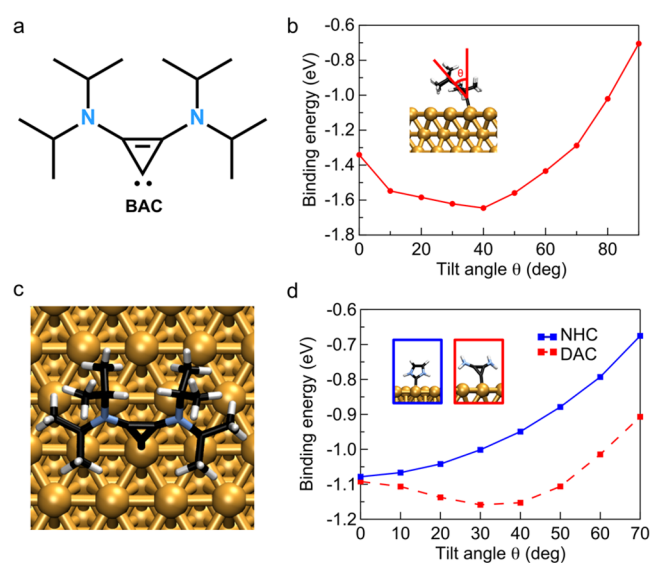
Figure 1. (a) Chemical structure of BAC. (b) Calculated binding energy of BAC as a function of tilt angle \theta . (c) Structure of BAC absorbed on the Au(111) surface for \theta = 40^\circ . (d) Calculated binding energy of DAC and NHC cores on the Au(111) surface as a function of tilt angle \theta .
