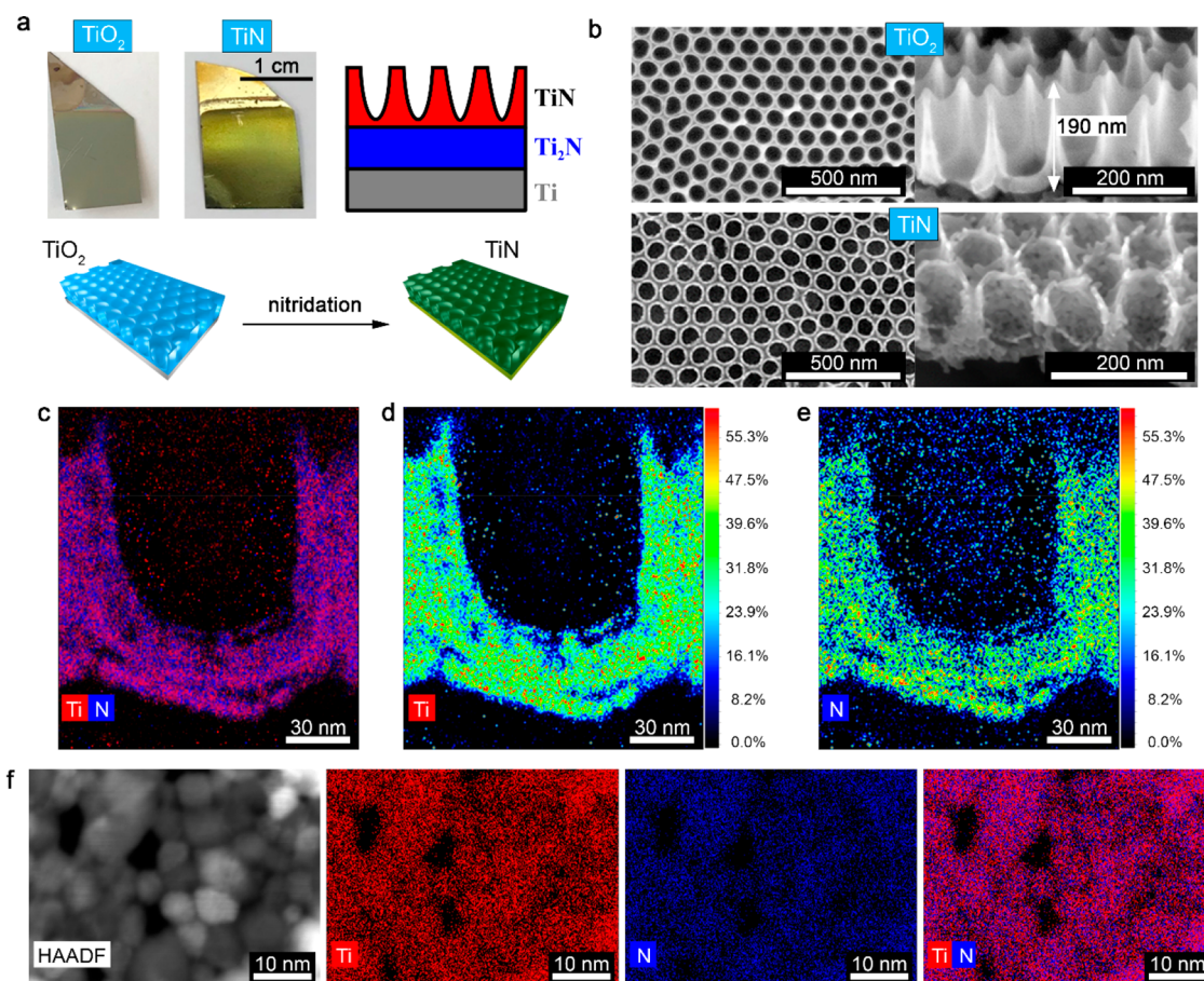
Figure 1. Structure and composition of TiN nanofurnaces. (a) Photographic image and schematic representation of \text{TiO}_2 nanocavities and TiN nanofurnaces. (b) SEM images showing top and cross-sectional views of \text{TiO}_2 nanocavities and TiN nanofurnaces. (c) HRTEM micrographs obtained by EDS elemental mapping for Ti (red) and N (blue) of a lamella prepared by focused ion beam micromachining. (d,e) Deconvoluted elemental mapping for Ti and N showing their atomic concentrations in the same lamella. (f) HAADF scanning TEM image and EDS elemental mapping for Ti (red) and N (blue) of crystallites forming the bottom of a single TiN nanofurnace.
