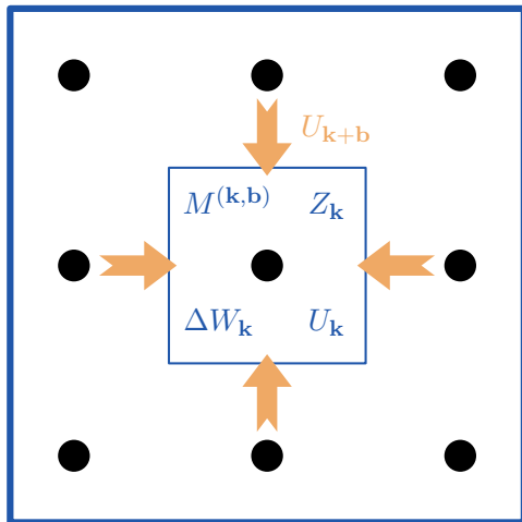
Figure 2. Illustration of the parallelisation scheme for a 3 \times 3 mesh of k -points (black dots) and one MPI process per k -point. The calculation of the M^{(\mathbf{k},\mathbf{b})} , Z_{\mathbf{k}} , \Delta W_{\mathbf{k}} and U_{\mathbf{k}} matrices are distributed over processes by k -point. The U_{\mathbf{k}+\mathbf{b}} matrices for the neighbouring k -points are sent from process to process (orange arrows) for the calculation of the M^{(\mathbf{k},\mathbf{b})} and Z_{\mathbf{k}} matrices.
