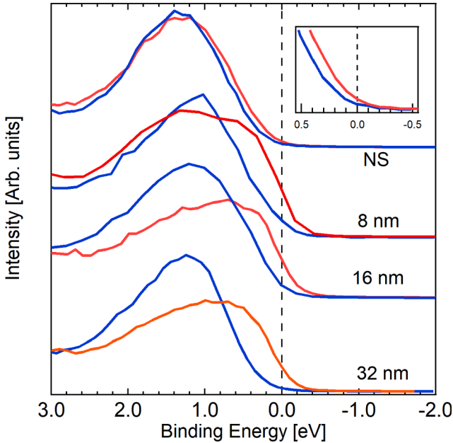
Fig. 3. VB spectra of the unpaired 3d electrons band in the BE range (-2; 3) eV in the insulating (blue) and metallic (red) phase of \text{VO}_2 . From top to bottom: the NS disordered sample, samples 8, 16 and 32 nm thick. The inset shows the increase of the population at the FL for the NS sample. (For interpretation of the references to colour in this figure legend, the reader is referred to the web version of this article.)
