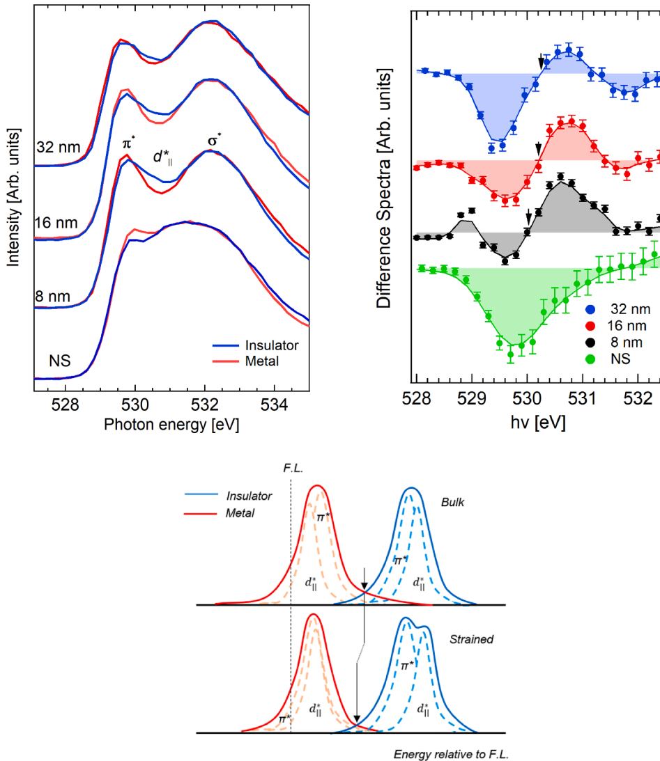
Fig. 2. Left panel: comparison of the O K edge XANES (527–535 eV) of VO 2 crystalline film of 32, 16 and 8 nm and the NS disordered film for metallic (red, 90° C) and insulating (blue, 30° C) phases. XANES spectra of the strained films are normalized respect to the maximum intensity of the \sigma^* feature at 532.2 eV; the spectra of the NS disordered films are normalized to the maximum of the intensity around the \sigma^* energy region: h\nu = 531.6 eV. Right panel: comparison of the difference spectra of the O K edge XANES in the range h\nu: 528 –532 eV. The dots represent experimental points while the continuous line (a guide for the eye) is the smoothed curve of the experimental points (binomial algorithm). From top to bottom: films of 32, 16 and 8 nm and the NS film. The black vertical arrows indicate the turning point of the difference from negative to positive contributions. Spectra are vertically shifted for sake of clarity. Bottom panel: the schematic empty band model for bulk and strained VO 2 in the insulator (blue) and metal (red) phases. The intersection point (marked by arrows) between the insulator and metal empty DOS shifts toward lower energy for the strained sample, because of the concurrent \pi^* , d_{||}^* separation in the insulating phase and \pi^* , d_{||}^* inversion in the metallic phase. (For interpretation of the references to colour in this figure legend, the reader is referred to the web version of this article.)
