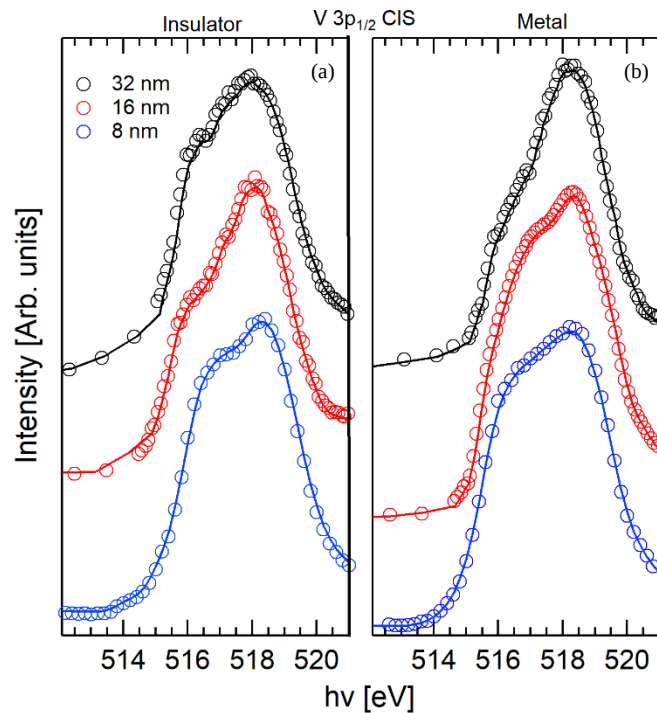
Figure 7. Comparison of CIS_{1/2} ( BE = 43.6 eV) spectra in the photon energy range 512.1–521.1 eV for the 32 nm, 16 nm and 8 nm thick films (black, red and blue lines, respectively). (a): the insulating phase spectra; (b): the metallic phase spectra.
