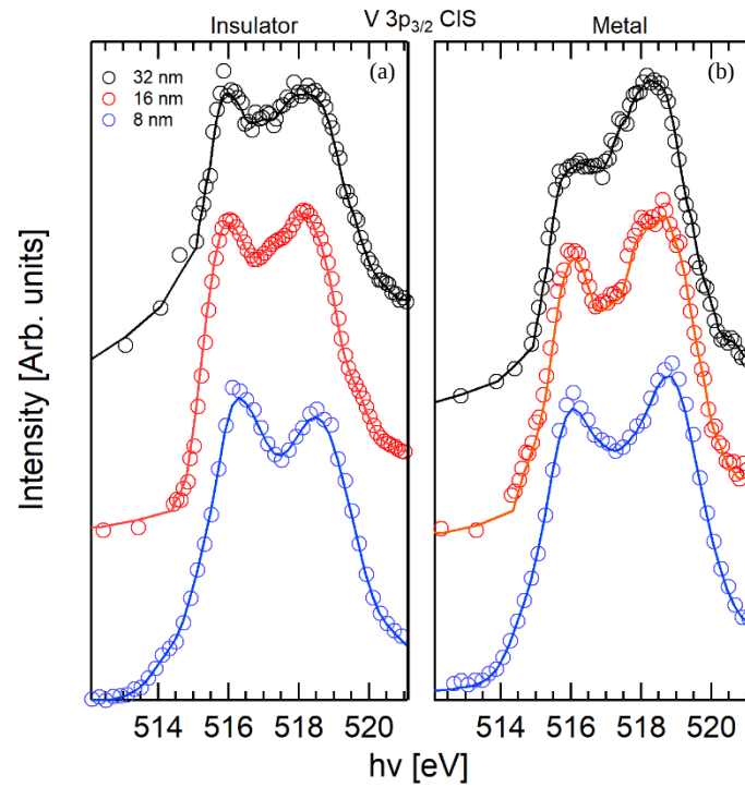
Figure 6. Comparison of CIS_{3/2} spectra ( BE = 41.2 eV) in the photon energy range 512.1–521.1 eV for the 32 nm, 16 nm and 8 nm thick films (black, red and blue lines, respectively). (a): The insulating phase spectra; (b): the metallic phase spectra.
