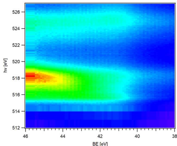
Figure 5. V 3p ResPes map of the sample of 32 nm thickness in the insulating phase. The map was collected in the photon energy range h\nu = 512\text{--}527 eV across the V L_3 ( \sim 518 eV) and L_2 ( \sim 526 eV) resonances. The color bar indicates the intensity scale: blue for low intensity and red for high intensity.
