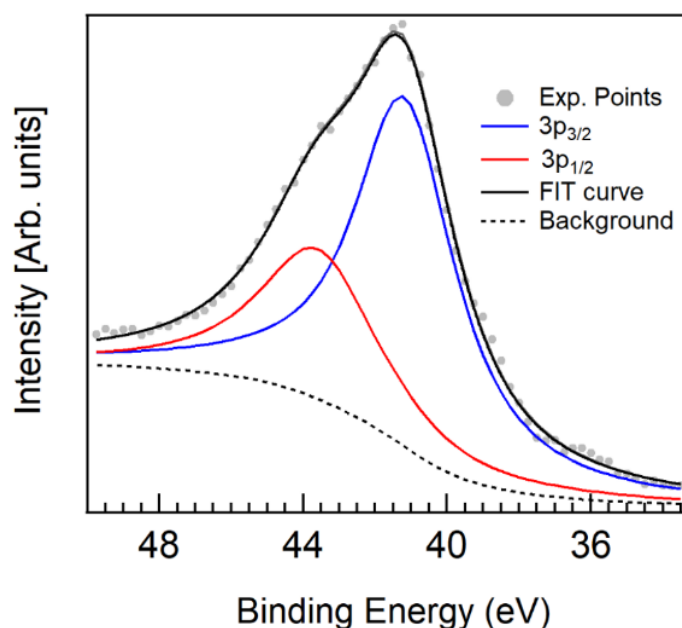
Figure A3. V 3p XPS spectrum of the 8 nm (−24 °C) films collected at h\nu = 510 eV. The experimental points (grey dots) are compared to the fit components (blue 3p_{3/2} ) and (red 3p_{1/2} ) and their sum (continuous black line).
