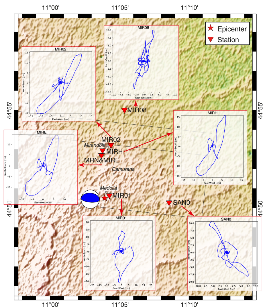
Figure 9. Particle motions of stations with impulsive signals in the 29 May 2012 (07:00) Emilia-Romagna earthquake. Stations MRN and MIRE are very close each other, and they have a very similar plot of the horizontal displacement.
