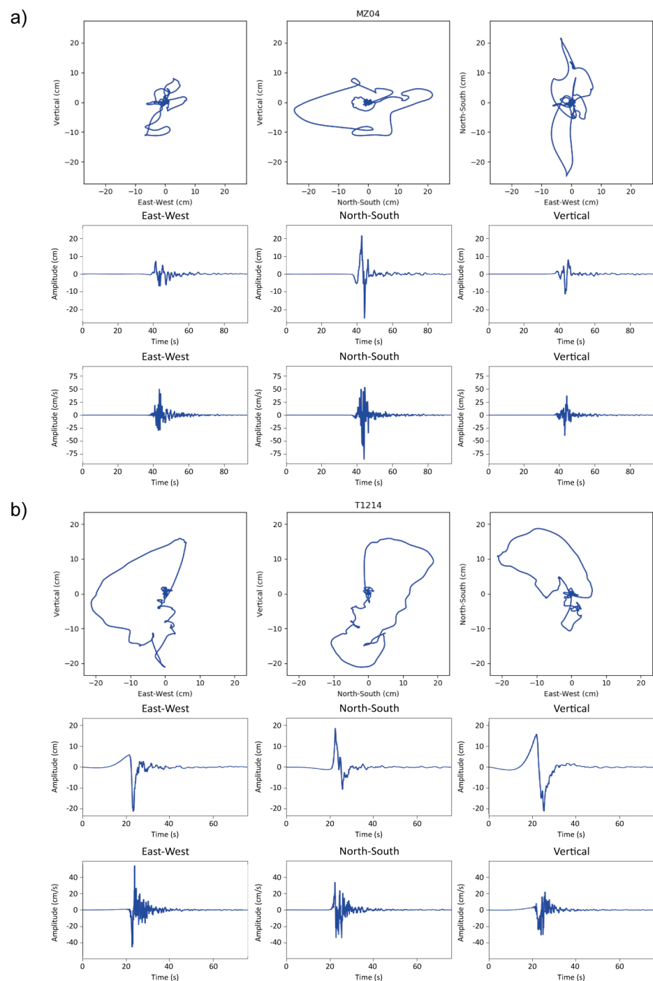
Figure 8. Ground motions of orthogonal components and velocity waveforms of (a) MZ04 and (b) T1214 stations in 30 October 2016 (06:40) Amatrice earthquake, respectively.
