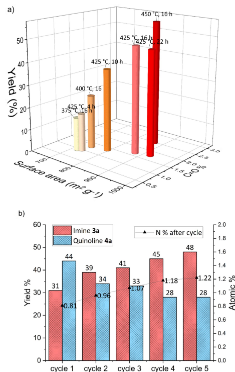
Figure 2. a) Catalytic activities against XPS analyzed C=O content and BET defined surface area of various oAC materials obtained by different oxidative treatments, b) Recycling tests for 1 a + 2 a to quinoline 4 a conversion with oAC-air(425). Reaction conditions: catalyst loading 224 mg/mmol, 110 °C, 4 h. Blue and red bars represent NMR yields of 4 a and 3 a accordingly. Triangles display the sum of pyridinic and pyrrolic atomic % content on the carbon material after each related cycle obtained from XPS analysis.
