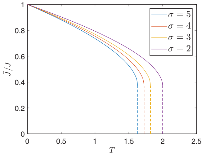
Fig. 1: Ratio \tilde{J}/J as a function of T = 1/J for different values of \sigma (with J defined in (20)). For each \sigma we find a jump of \tilde{J} to zero at a temperature denoted in the text and in fig. 2 as T_c .
