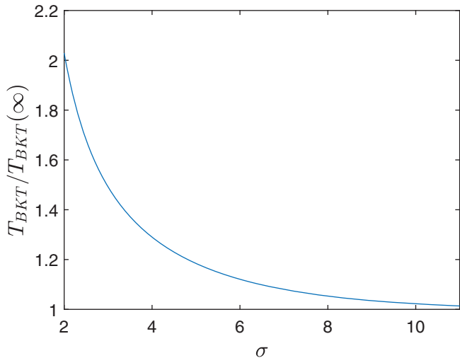
Fig. 4: Estimate of T_{BKT}(\sigma) in units of the \sigma \rightarrow \infty value T_{BKT}(\infty) .
