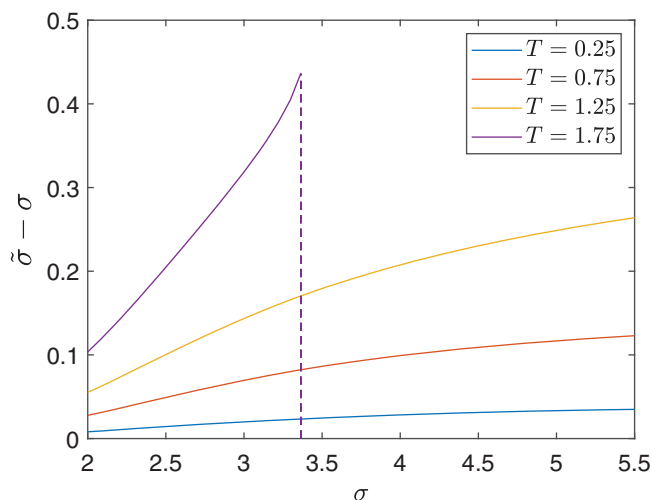
Fig. 3: Behavior of \tilde{\sigma} - \sigma as a function of \sigma for different values of the temperature T . It is seen that \tilde{\sigma} > \sigma everywhere.
