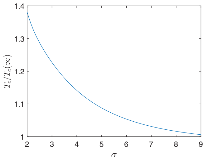
Fig. 2: T_c(\sigma) at which \tilde{J} jumps, in units of the \sigma \rightarrow \infty value T_c(\infty) = \frac{4}{e} . We see that the temperature is finite for \sigma \rightarrow 2 .
