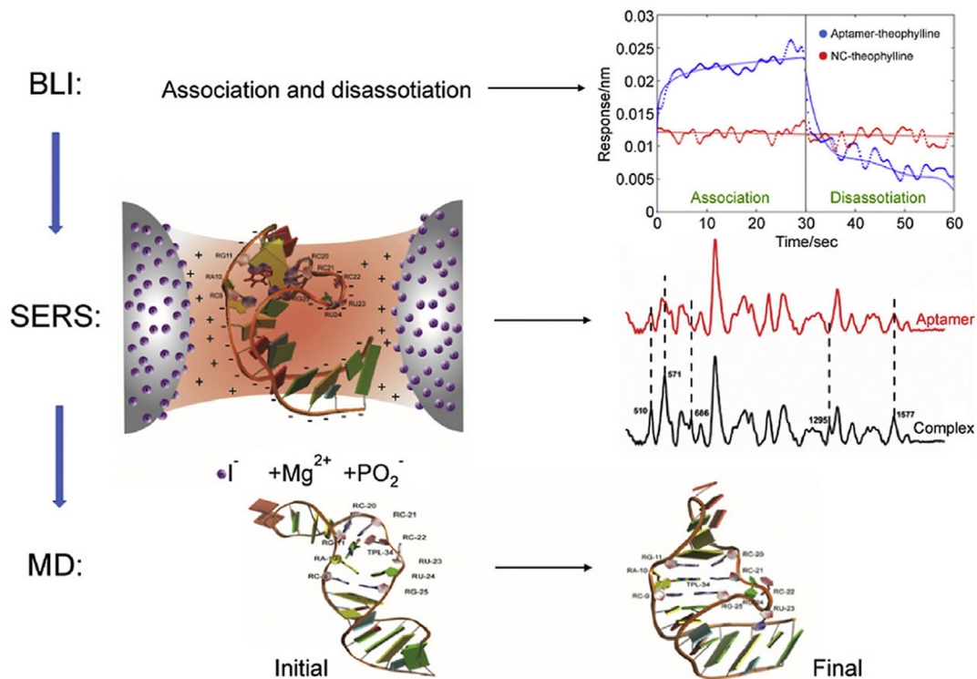
Fig. 6. The kinetic parameters of theophylline binding to its aptamer were determined using BLI. The combination with SERS and MD simulations allowed the authors to analyse the conformational changes of the aptamer and finally an in-depth understanding of the aptamer-theophylline binding process was obtained. Reprinted with permission from Ref. [106]. Copyright (2020) Elsevier.
