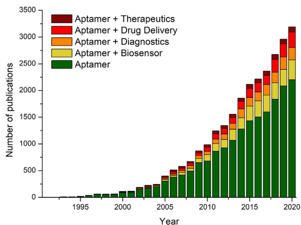
Fig. 1. Number of publications per year related to aptamers and their applications. The plot shows the exponential growth of the publications in the field over the last 15 years. Bibliographic analysis performed with Scopus searching for the following keywords: "aptamer*", "aptamer* AND biosensor*", "aptamer* AND therapeutic*", "aptamer* AND drug delivery*" and "aptamer* AND diagnostic*" per year. Data from Scopus retrieved on January 14, 2021.
