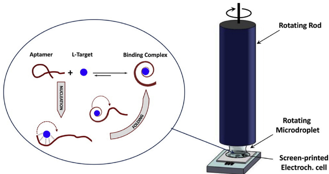
Fig. 4. Scheme of the kinetic rotating droplet electrochemistry (RDE) setup developed by Limoges using a screen-printed three-electrode electrochemical microcell (with a carbon working electrode, a silver reference electrode and a carbon counter-electrode), on the right. Aptamer-target interaction processes investigated with the RDE method, on the left. Reprinted with permission from Ref. [29]. Copyright (2016) American Chemical Society.
