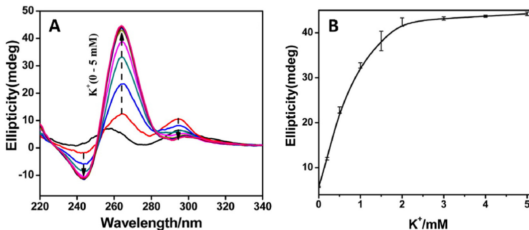
Fig. 8. A) CD spectra of the PW17 aptamer with G-quadruplex structure. Spectra are recorded with K + concentrations from 0.02 mM to 5 mM from bottom to top. B) The CD intensity at 264 nm is plotted in function of the K + concentration. The CD spectroscopy results show the G-quadruplex formation induced by the presence of K + and that from 2 mM K + onwards a stable structure is formed. Reprinted with permission from Ref. [139]. Copyright (2016) American Chemical Society.
