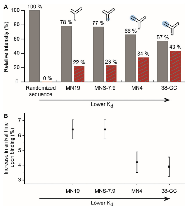
Fig. 3. Native IM-MS measurements of four cocaine-binding aptamers (MN19, MNS-7.9, MN4, and 38-GC) and a randomized sequence in complex with quinine. A) The relative abundance of the aptamer and complex are shown in grey and red, respectively. B) Changes in IM-behaviour, i.e. the arrival time, for all aptamers. More rigid aptamers (MN4 and 38-GC) were found to undergo smaller conformational changes than flexible aptamers (MN19 and MNS-7.9). Reprinted with permission from Ref. [57]. Copyright (2021) Elsevier.
