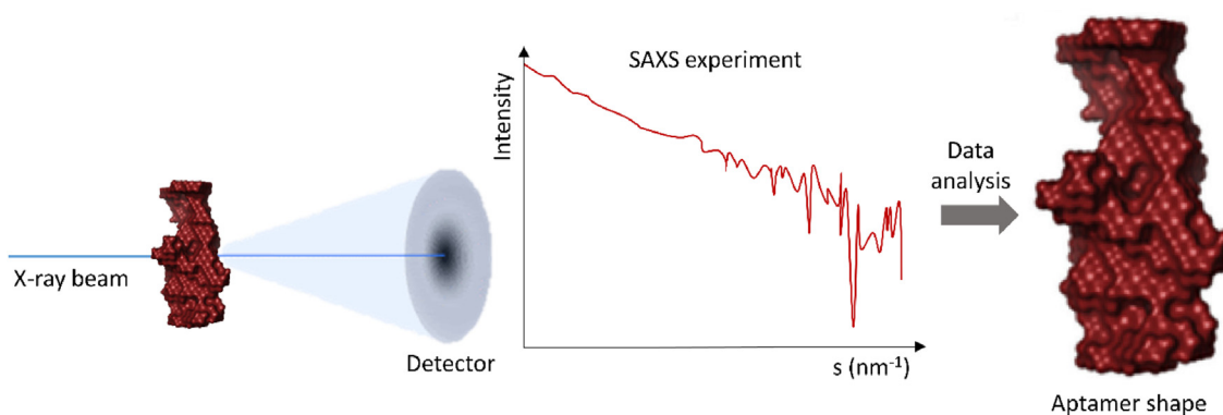
Fig. 9. The general working principle to obtain information on the aptamer shape using SAXS. SAXS experiments are performed on an aptamer in solution and consequently a structural envelope is built from these SAXS results. Adapted from Tomilin et al. [146].
