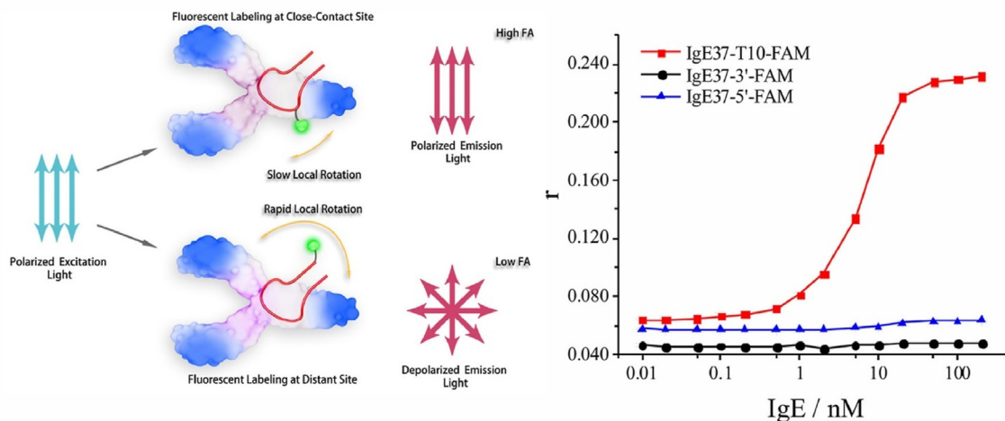
Fig. 5. Fluorescence anisotropy analysis of IgE and its aptamer with a single fluorescein label (FAM). The site of the label influences the movement of the label and therefore also the light emitted. Slow local rotations lead to emission of polarised light, while rapid rotations lead to depolarised emission. The results show the label at the T10 position can detect binding of the aptamer to IgE, while the aptamer with label at the 3' or 5' end does not detect the binding. Reprinted with permission from Ref. [70]. Copyright (2020) Elsevier.
