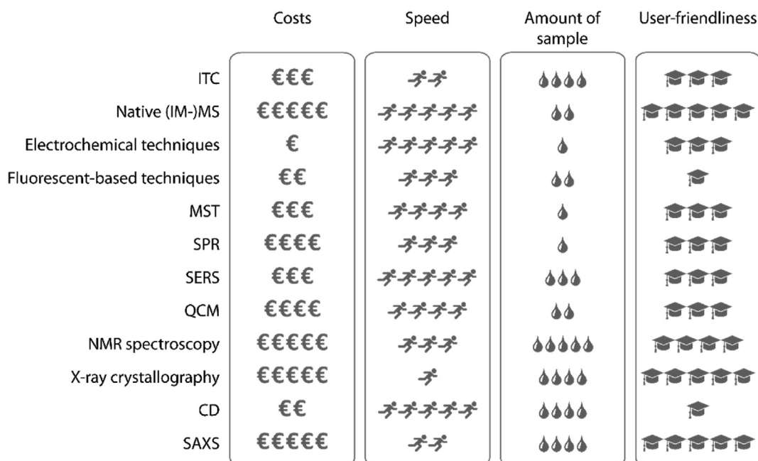
Fig. 11. Comparison of the discussed techniques in terms of costs, speed, amount of sample required and user-friendliness.
