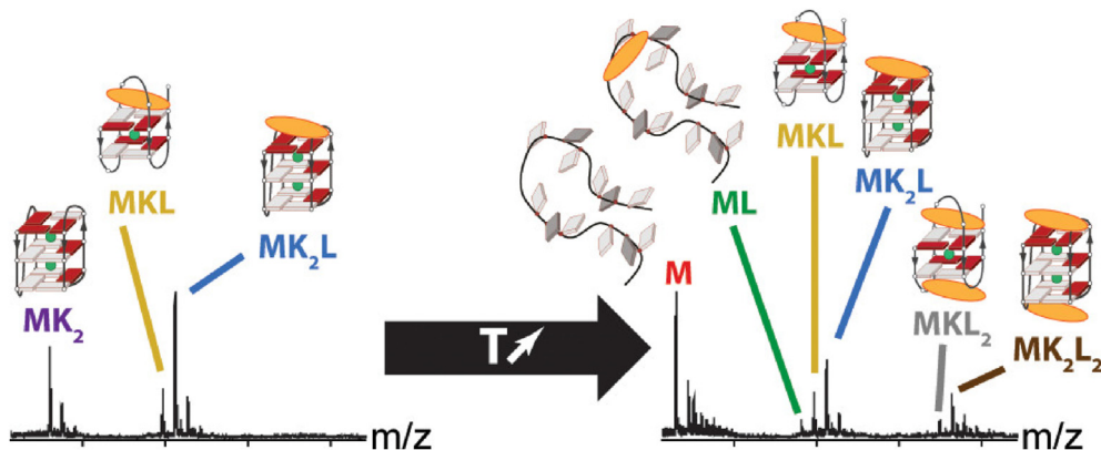
Fig. 2. Native MS was used to detect and quantify each specific stoichiometry: number of strands in the G-quadruplex, number of potassium ions (in green) and number of ligands (in yellow). By using a temperature-controlled electrospray source, the behaviour of the complex at different temperatures was monitored. From this, temperature-dependent equilibrium constants and thus the enthalpic and entropic contributions to the formation of each stoichiometry were determined. Reprinted with permission from Ref. [54]. Copyright (2018) American Chemical Society.
