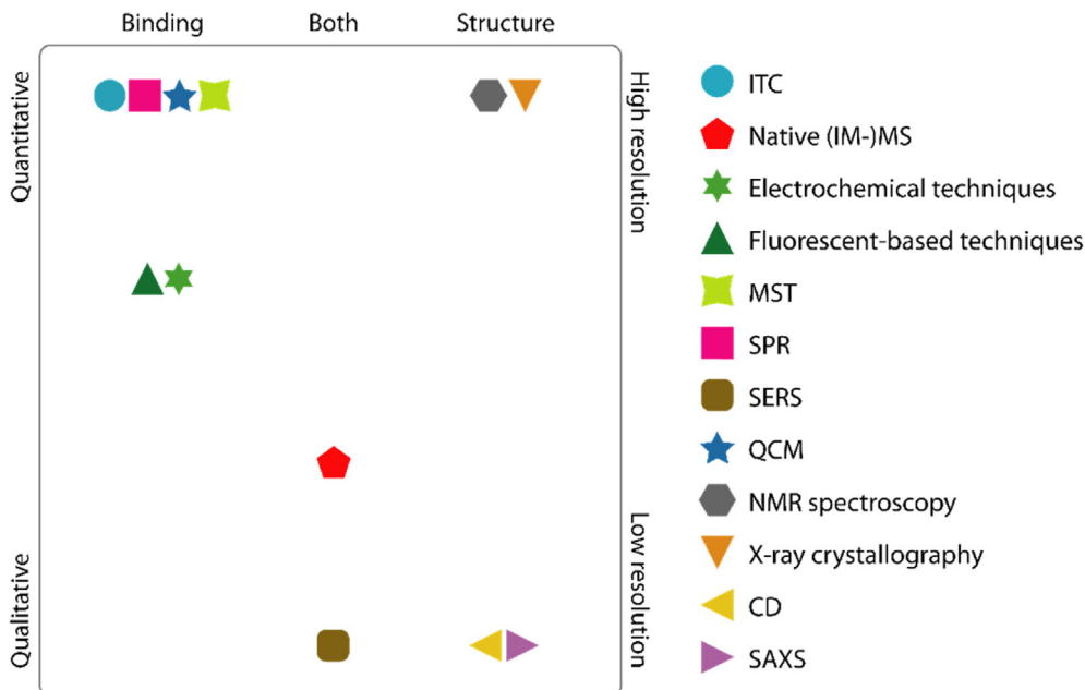
Fig. 10. Overview of the information on aptamer-target complexes obtained using each of the discussed techniques. The information concerns the binding, the structure or both. Binding information can be the quantitative, semi-quantitative or qualitative while for structural information the level of resolution is considered (high or low).
