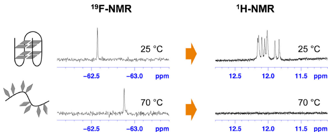
Fig. 7. ^{19}\text{F} NMR and ^1\text{H} NMR spectra of the thrombin-binding aptamer with an ^{19}\text{F} -labelled nucleotide at the T10 position at 25 or 70°C. The quadruplex is unfolded at 70°C which results in a change of chemical shift in ^{19}\text{F} NMR and a disappearance of the signals in ^1\text{H} NMR. Reprinted with permission from Ref. [129]. Copyright (2017) American Chemical Society.
