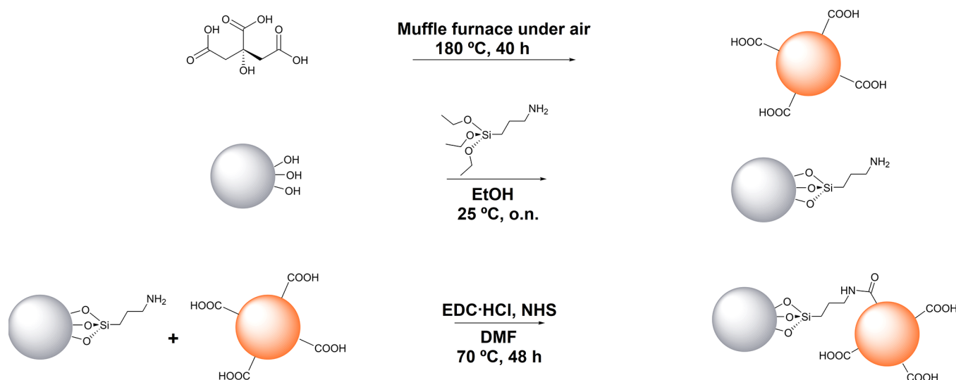
Scheme 1. Synthesis Routes of \alpha -CDs, Amino-Terminated \text{SiO}_2 Nanoparticles, and Hybrids of \alpha -CDs Coupled to a- \text{SiO}_2
