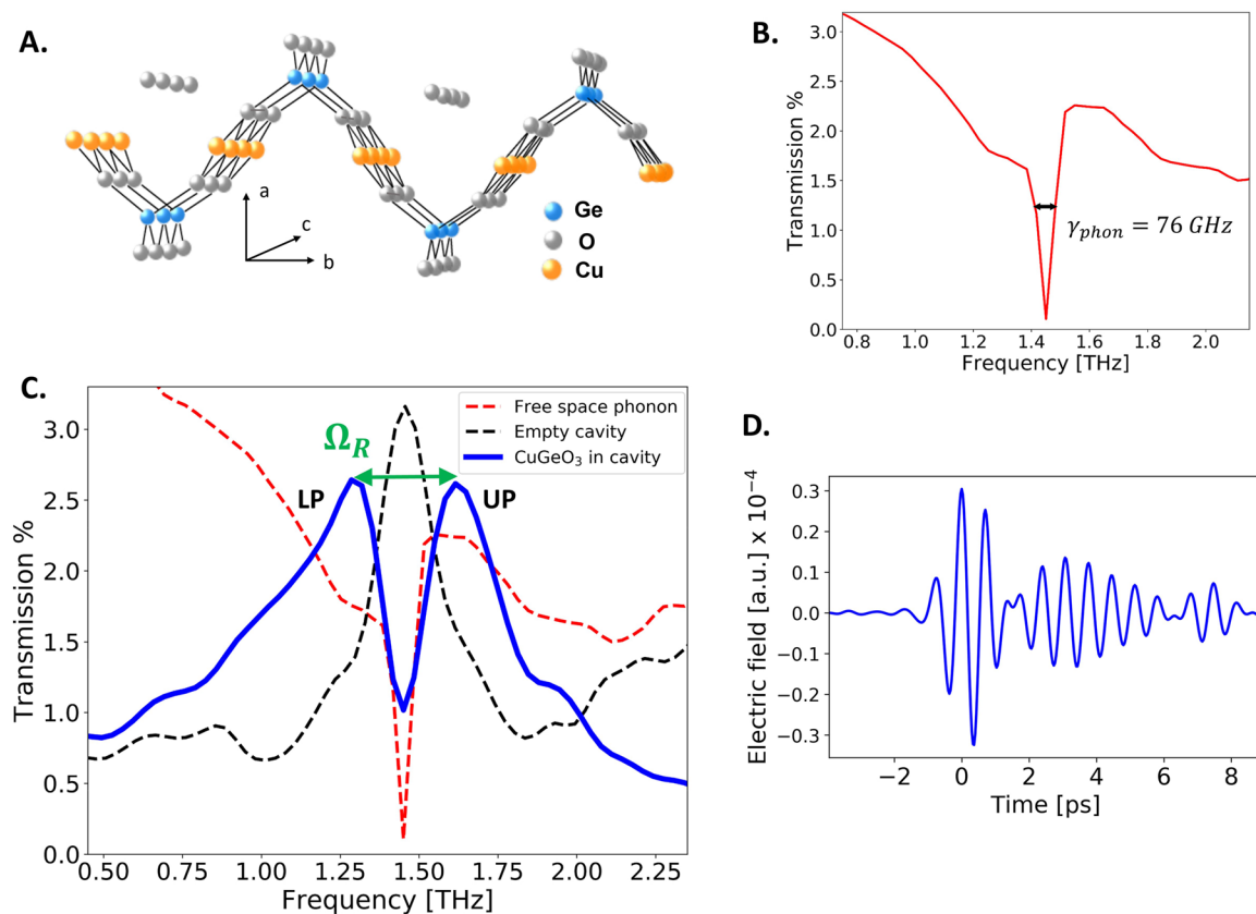
FIG. 4. Demonstration of the phonon strong coupling regime in CuGeO 3 at 80 K. (a) CuGeO 3 crystal structure in the normal phase. (b) Open cavity CuGeO 3 transmission at 80 K of THz light polarized along the b axis, showing an IR-active mode at 1.45 THz with a linewidth \gamma_{phon} = 76 GHz. (c) Static transmission of CuGeO 3 at 80 K in a cavity of length with the fundamental frequency resonant to the phonon one. Strong coupling between the phonon and the cavity modes results in a spectral splitting into two new modes: Upper Polariton (UP) and Lower Polariton (LP) with a separation \Omega_R greater than either the free-space phonon linewidth (red dashed curve) and the empty cavity linewidth at the resonance frequency (black dashed curve). (d) Time-dependent THz field at the resonance filtered in the range of 0.5–2.3 THz showing coherent Rabi oscillations associated with the strong coupling regime.
