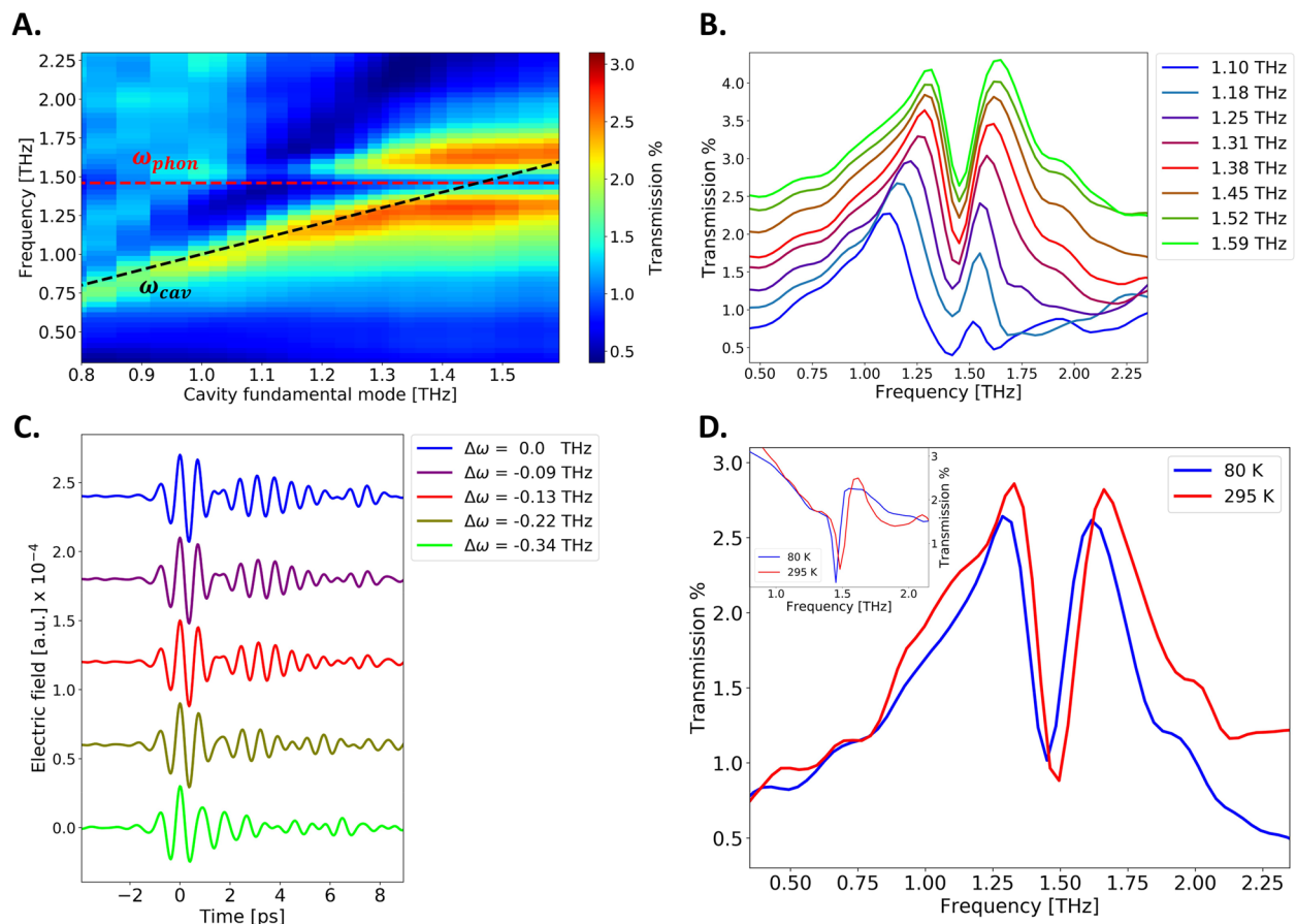
FIG. 5. (a) Phonon-polariton dispersion in the strong coupling regime of CuGeO 3 at 80 K. The red dashed line marks the uncoupled phonon frequency \omega_{\text{phon}} = 1.45 THz, while the black dashed one marks the uncoupled cavity mode \omega_{\text{cav}} . (b) Evolution of the cavity transmission spectra at 80 K with cavity fundamental frequencies (indicated in legend) across the phonon resonance (c). Evolution of the filtered THz fields exiting the cavity at 80 K for different cavity detunings \Delta\omega = \omega_{\text{cav}} - \omega_{\text{phon}} (d). Comparison of the strongly coupled cavity-phonon transmission at 80 and 295 K. The shift of the polaritons' frequencies is consistent with a phonon frequency shift, as highlighted in the open cavity transmission spectra shown in the inset.
