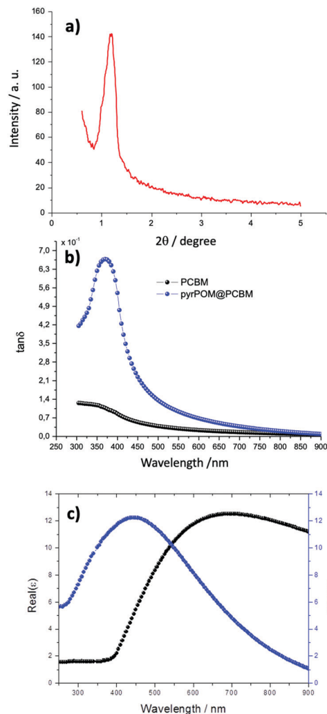
Fig. 4 (a) XRD measurement shows a periodicity of (7.6 \pm 0.2) nm of the LS pyrPOM@PCBM layer. (b and c) The dielectric loss of pyrPOM@PCBM, dramatically different from that one of PCBM, suggests that an electric dipole is created at the opposite edges of the nanodomains. Increasing the frequency, the dielectric permittivity of pyrPOM@PCBM LS film becomes negligible.
