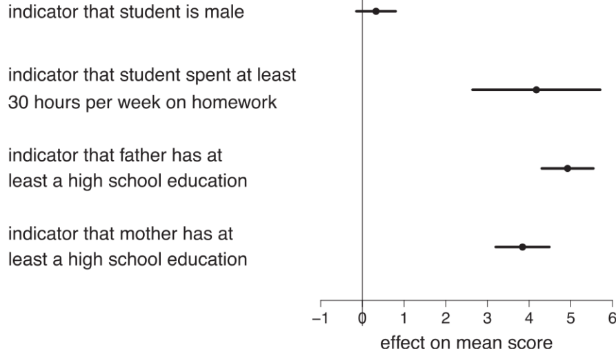
Figure 6. Approximate posterior means (solid dots) and 95% credible intervals (line segments) for \beta_2, \dots, \beta_5 for the mean field variational Bayes, with product restriction III, fit of (12) to data from the National Education Longitudinal Study of 1988.
