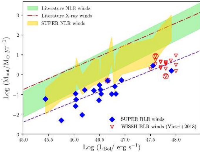
Fig. 14. Outflow mass rate as a function of the logarithm of the bolometric luminosity for the BLR winds in the SUPER sample. Values from the WISSH sample ( Vietri et al. 2018 ) (triangles) are also reported. BAL AGNs are denoted with red circles. The blue dashed line is the best-fit correlation of the CIV winds (SUPER+WISSH samples). Mass outflow rates of NLR winds from the SUPER sample are also reported (gold shaded area). The green shaded area shows the range probed by the outflow ionised phase in the NLR as found by Fiore et al. (2017) , after rescaling the relation with the same assumption as for the Type-1 SUPER targets (see Kakkad et al. 2020 for further details). The dot-dashed line shows the log linear best-fit correlation of the X-ray winds.
