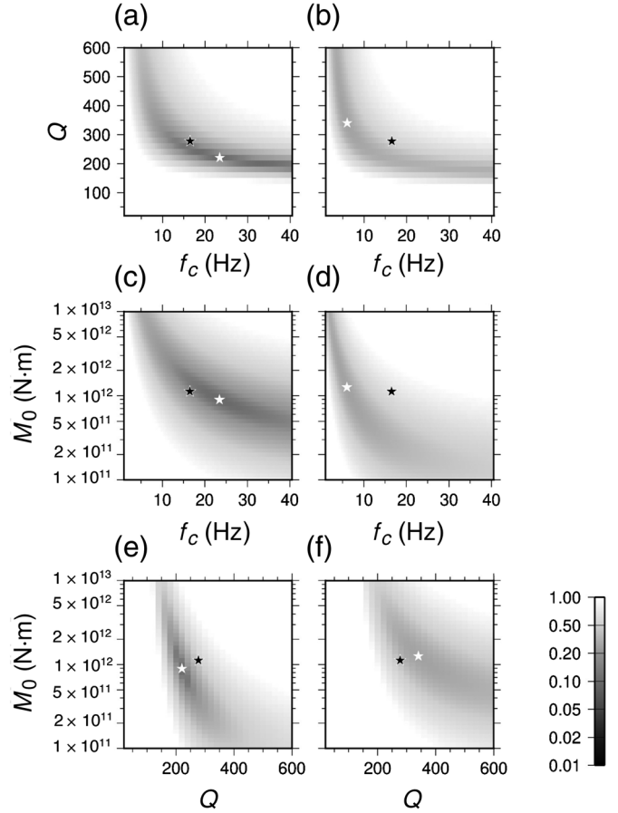
Figure 18. Misfit value on planes crossing the best-fit solution for an M_w 2.0 event and considering the M2q_s model. The white star indicates the minimum misfit solution, and the black star depicts the real values used for the synthetic seismogram calculation. (a,c,e) Results for epicentral distance of 15 km: (a) visualization on the Q - f_c plane, (c) visualization on the M_0 - f_c plane, and (e) visualization on the M_0 - Q plane. (b,d,f) Results for epicentral distance of 25 km: (b) visualization on the Q - f_c plane, (d) visualization on the M_0 - f_c plane, and (f) visualization on the M_0 - Q plane.
