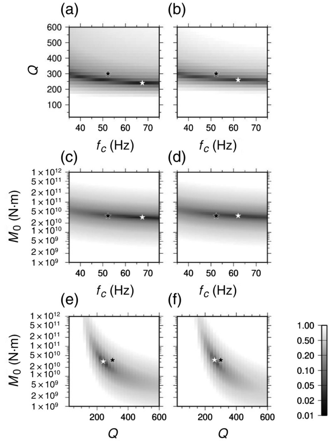
Figure 8. Misfit value on planes crossing the best-fit solution for an M_w 1 event and considering the M1q model. The white star indicates the minimum misfit solution, and the black star depicts the real values used for the synthetic seismogram calculation. (a,c,e) results for epicentral distance of 15 km: (a) visualization on the Q - f_c plane, (c) visualization on the M_0 - f_c plane, (e) and visualization on the M_0 - Q plane. (b,d,f) Results for epicentral distance of 25 km: (b) visualization on the Q - f_c plane, (d) visualization on the M_0 - f_c plane, (f) and visualization on the M_0 - Q plane.
