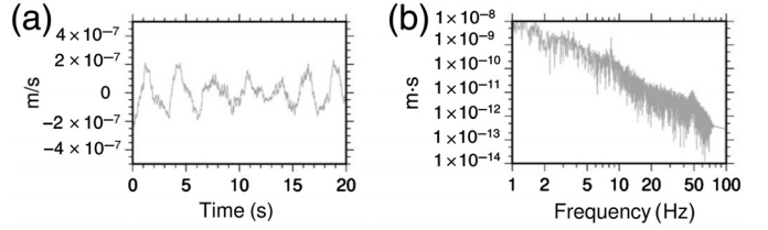
Figure 2. (a) Seismic noise time series. (b) Fourier spectrum of the seismic noise time series in displacement.
