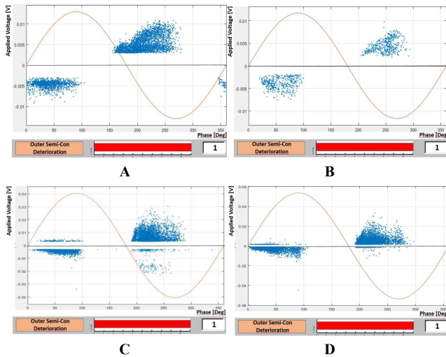
Fig.6. PRPD patterns due to discharges occurring due to deterioration of outer stress-grading layer. PD patterns recorded testing A) a MV cable at its rated voltage of 16kV; B) and artificial defect obtained testing an abraded semi-con material; C) and D) a new cable provided by a joint in the middle. Test performed using a C_k=2nF (C) and a HFCT (D).
