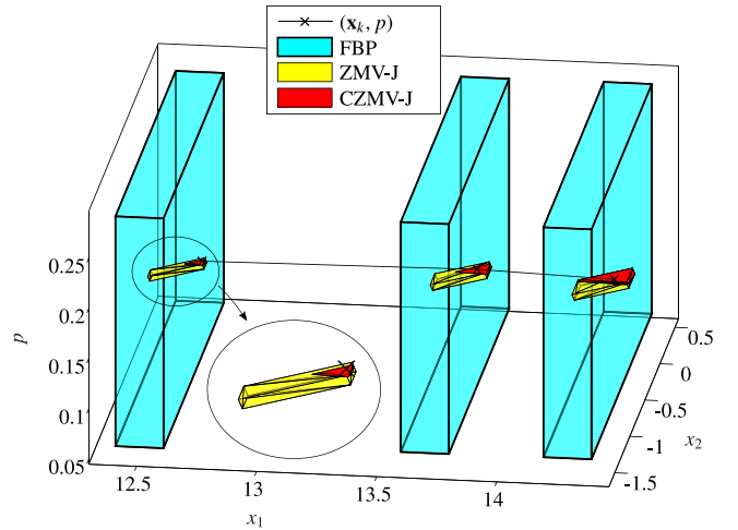
Fig. 2. The variables (\mathbf{x}_k, p) ( \times ), and the sets obtained using ZMV-J (yellow), CZMV-J (red), and interval arithmetic (cyan), for the nonlinear system (16) at k \in \{3, 15, 149\} . (For interpretation of the references to color in this figure legend, the reader is referred to the web version of this article.)
