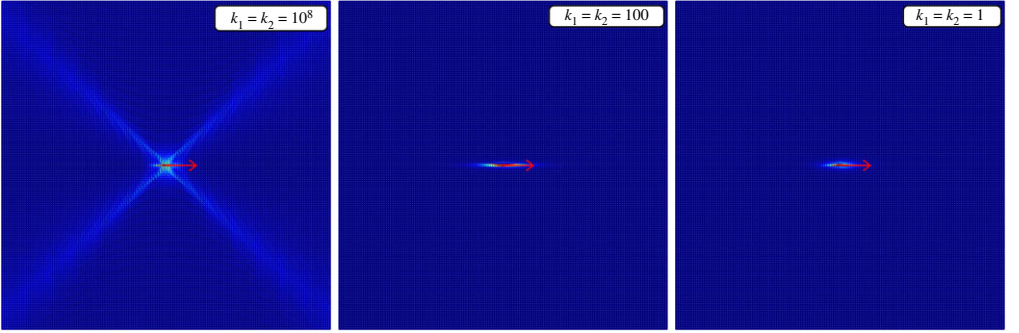
Figure 6. As for figure 5, except that the frequency \Omega = 3.0 is investigated for \kappa = \{10^8, 100, 1\} . The selected frequency falls within the low-frequency band gap of figure 4 for \kappa = 100 and 1, so propagation is here suppressed.
