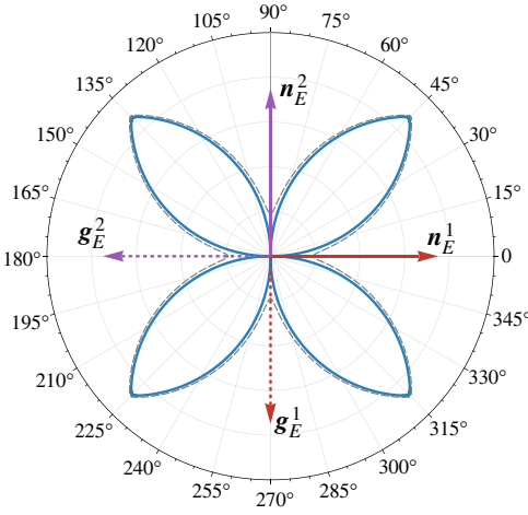
Figure 18. As for figure 13, except that the preload is equibiaxial, p_1 = p_2 . Polar plots are reported of the square root of the lowest eigenvalue of the acoustic tensor of the solid equivalent to the elastic grid, for an equibiaxial prestress state at failure of ellipticity in: (a) compression ( p_1 = p_2 = p_E^- = -4.74102 ); (b) tension ( p_1 = p_2 = p_E^+ = 34.06669 ).
