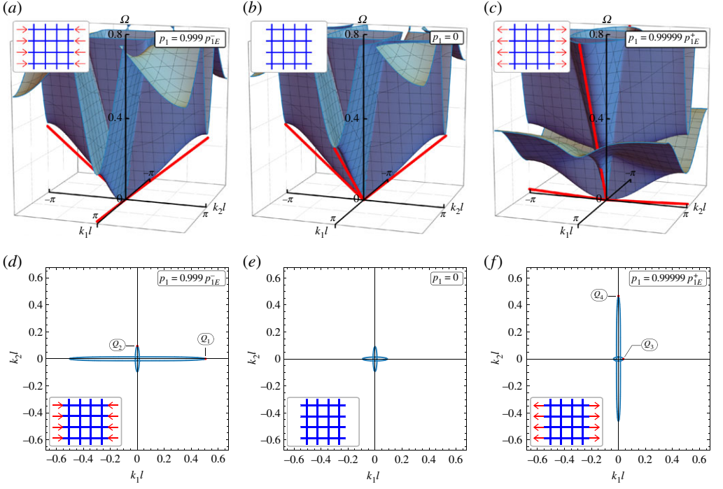
Figure 12. Dispersion surfaces (a–c) and slowness contours (d–f) at low frequency \Omega = 0.01 for preload levels near macro bifurcation in compression (a,d) and tension (c,f), compared with the case of null preload (b,e). The infinite-wavelength bifurcation occurs at the vanishing slope of one of the acoustic branches at the origin when the preload reaches the critical values reported in table 1. Red lines are tangent to the surfaces at the origin and represent the response of the equivalent continuum.
