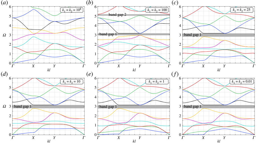
Figure 4. (a–f) Dispersion curves for a square grid of elastic rods without preload, for different values of the slider stiffness \kappa = 10^8, 100, 25, 10, 1, 10^{-2} . The diagrams have been evaluated along the boundary of the first irreducible Brillouin zone (path \Gamma-X-Y-\Gamma sketched in figure 3). The relative band gaps are highlighted in figures b–f. ‘Twin band gaps’ are visible in panel b.
