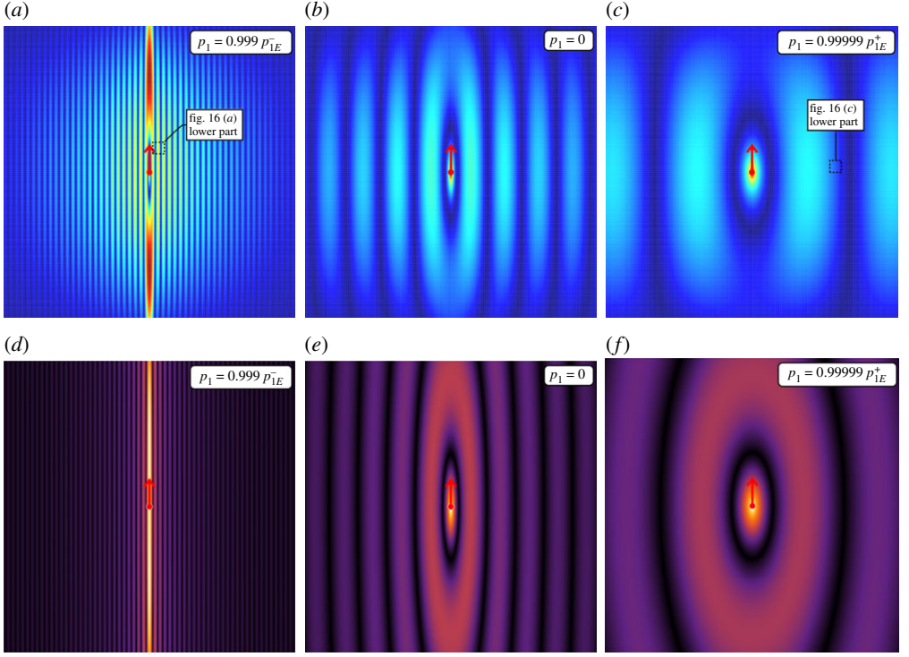
Figure 14. Displacement amplitude field during vibrations of a grid of Rayleigh rods with \kappa = 100 , excited by a vertical time-harmonic force pulsating at frequency \Omega = 0.01 . The preload in the horizontal rods is applied up to near the critical values p_{1E}^- and p_{1E}^+ , see table 1. The plots show shear band formation (a,d) near ellipticity loss, contrasted with the elliptic case (where shear bands are excluded, b,e) and the other case of loss of ellipticity in tension (where shear bands do not emerge, c,f).
