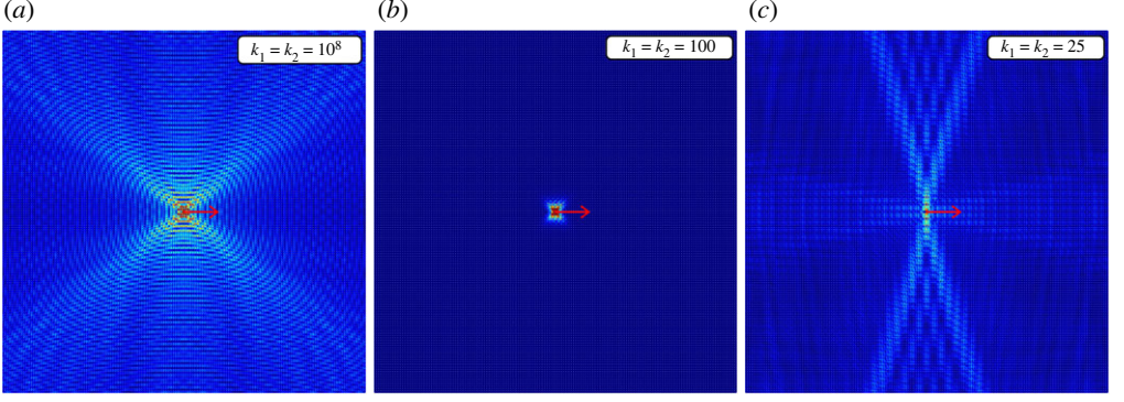
Figure 7. (a–c) As for figure 6, except that the vibration frequency, \Omega = 5.1 , is internal to the high-frequency band gap visible in figure 4 at \kappa = 100 . Here propagation is suppressed. Decreasing the stiffness of the sliders to \kappa = 25 , the high-frequency-band gap closes and propagation is again possible.
