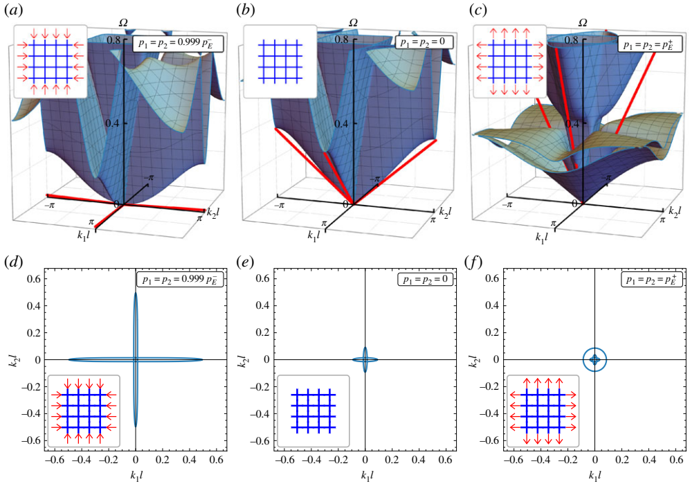
Figure 17. As for figure 12, except that the preload is biaxial p_1 = p_2 . Dispersion surfaces (a–c) and slowness contours (d–f) are shown at low frequency \Omega = 0.01 for preload levels near macro bifurcation in compression (a,d) and micro bifurcation in tension (c,f), compared with the case of null preload (b,e).
