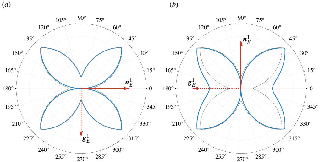
Figure 13. Polar plots of the square root of the lowest eigenvalue of the acoustic tensor of the solid equivalent to the elastic grid, as a function of the propagation direction \mathbf{n} = \cos \theta \mathbf{e}_1 + \sin \theta \mathbf{e}_2 , for a uniaxial prestress state at failure of ellipticity in: (a) compression ( p_1 = p_{1E}^- = -5.01017 ); (b) tension ( p_1 = p_{1E}^+ = 34.066669 ), see table 1. The dashed grey line reports the behaviour of the solid without prestress, where loss of ellipticity does not occur.
