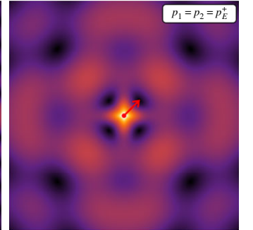
Figure 19. As for figure 14, except that the preload is equibiaxial, p_1 = p_2 and that the concentrated force is diagonally inclined (at \pi/4 ). The displacement field is shown during vibrations of a grid of Rayleigh rods at a frequency \Omega = 0.01 , with the critical preload values, p_E^- and p_E^+ listed in table 2. Differently from the uniaxial preload, shear bands do not emerge at the failure of ellipticity in tension (c,f), where a micro bifurcation occurs simultaneously with the macro bifurcation and prevails on the latter. In compression (a,d) the inclined force excites both a horizontal and a vertical shear band.
