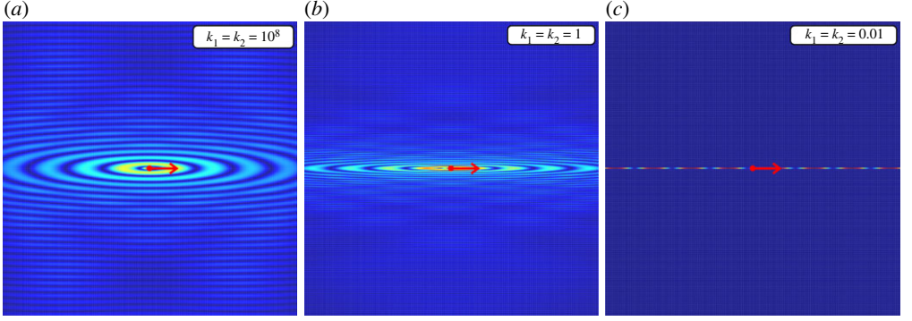
Figure 5. (a–c) Maps of displacement amplitude (obtained through F.E. analyses) for different stiffness of the sliders \kappa = \{10^8, 1, 10^{-2}\} of a grid of Rayleigh rods (without preload). The latter is excited by a time-harmonic concentrated force (aligned parallel to the horizontal direction) vibrating at low frequency, \Omega = 0.05 . When the slider stiffness becomes vanishing small a strong localization of the signal is observed, visible on the right.
