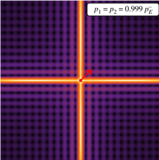
Figure 19. As for figure 14, except that the preload is equibiaxial, p_1 = p_2 and that the concentrated force is diagonally inclined (at \pi/4 ). The displacement field is shown during vibrations of a grid of Rayleigh rods at a frequency \Omega = 0.01 , with the critical preload values, p_E^- and p_E^+ listed in table 2. Differently from the uniaxial preload, shear bands do not emerge at the failure of ellipticity in tension (c,f), where a micro bifurcation occurs simultaneously with the macro bifurcation and prevails on the latter. In compression (a,d) the inclined force excites both a horizontal and a vertical shear band.
