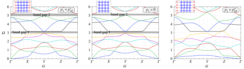
Figure 11. Evolution of the dispersion curves with uniaxial preload ( p_2 = 0 ). The slider stiffness is assumed equal to \kappa = 100 . The curves on the left correspond to the compressive critical preload in table 1, the ones in the centre correspond to the grid without preload, and the curves on the right to the grid with tensile critical preload in table 1.
