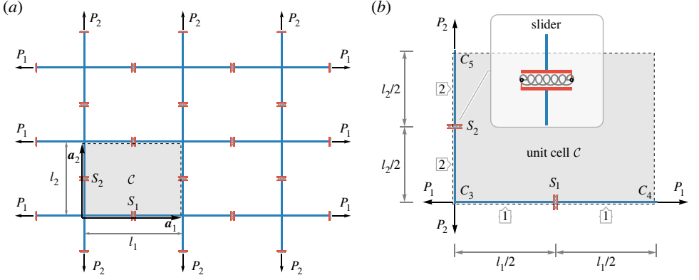
Figure 2. (a) A rectangular lattice of axially preloaded rods, endowed with sliding constraints, realizes an architected material capable of losing ellipticity under both tensile and compressive loadings. Linear springs are introduced to stiffen the sliders, thus preventing the occurrence of ‘floppy modes’. (b) The unit cell with two sliders.
