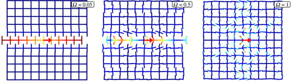
Figure 9. Details of figure 8 showing localization of the vibrational displacement, in the proximity of the row where the load is applied at \Omega = 0.05 and 0.5 , while at high frequency \Omega = 1 , waves spread through the ‘quasi-overdetermined’ grid of rods, characterized by small slider stiffness \kappa_1 = \kappa_2 = 0.01 .
