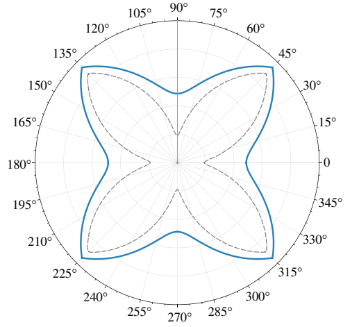
Figure 18. As for figure 13, except that the preload is equibiaxial, p_1 = p_2 . Polar plots are reported of the square root of the lowest eigenvalue of the acoustic tensor of the solid equivalent to the elastic grid, for an equibiaxial prestress state at failure of ellipticity in: (a) compression ( p_1 = p_2 = p_E^- = -4.74102 ); (b) tension ( p_1 = p_2 = p_E^+ = 34.06669 ).
