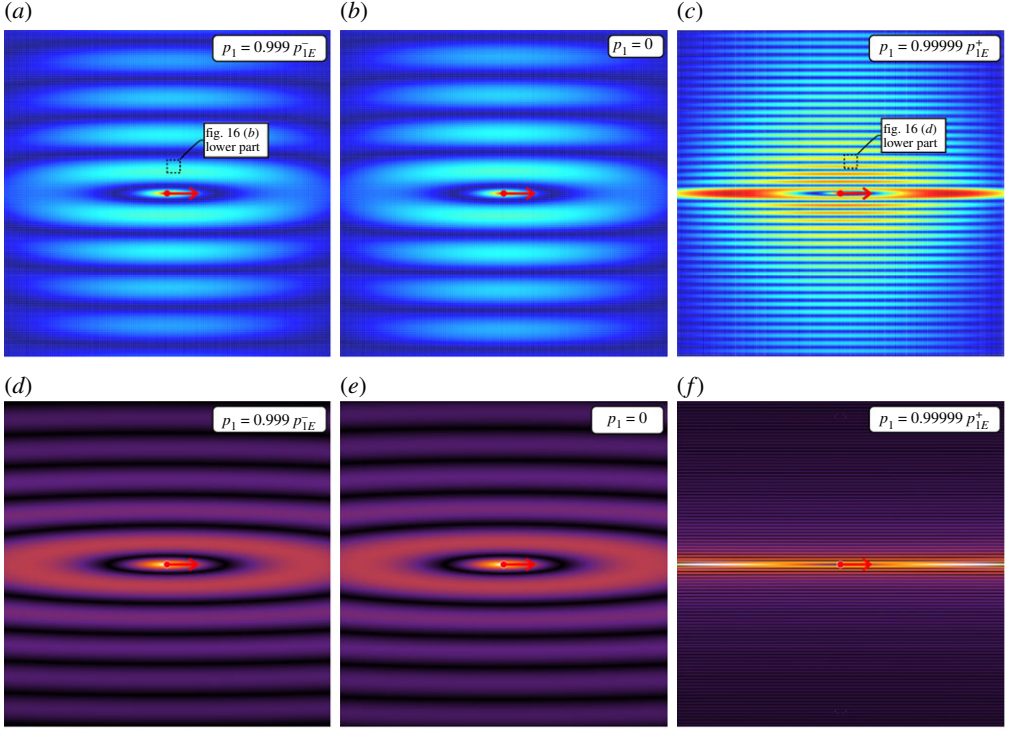
Figure 15. As for figure 14, except that the force is horizontal. Now shear bands appear near the boundary of ellipticity loss in tension (c,f), but not in compression (a,d).
