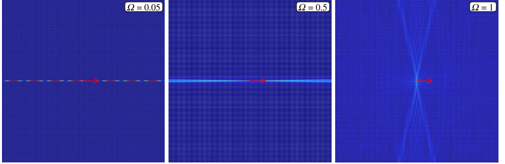
Figure 8. Vibrations of a ‘quasi-overdetermined’ grid of Rayleigh rods, characterized by a low slider stiffness \kappa_1 = \kappa_2 = 0.01 , in the absence of preload and excited by a time-harmonic horizontal force pulsating at different frequencies. The displacement field is strongly localized at low frequencies \Omega = 0.05 and 0.5 , as the effect of the low compliance of the sliders, while at high frequency, \Omega = 1 , the wave spreads to the entire lattice.
