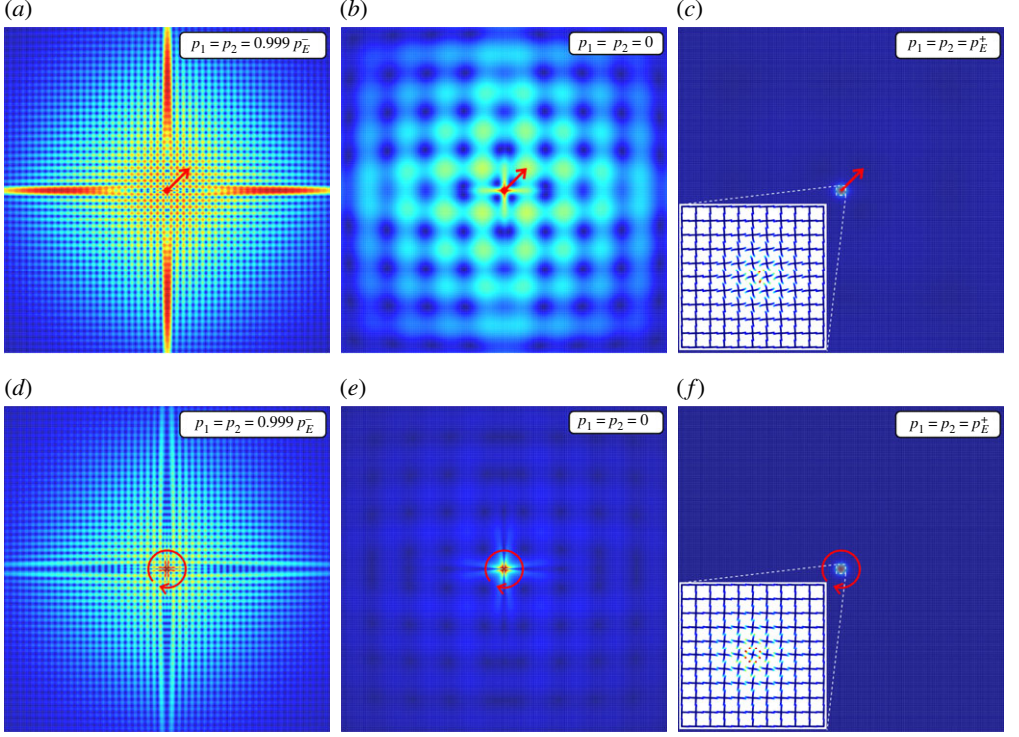
Figure 20. As for figure 19, except that the inclined force is applied on a slider face, instead of at the central node of the grid ( a–c ), and a concentrated moment is applied at the central node of the grid ( d–f ). While for compressive and null preloads the plots are very similar to those reported in figure 19 a,b , the results pertaining to the failure of ellipticity in tension ( c,f ) show that a micro instability prevails so that the response to the applied force or moment remains strongly localized in a vanishing small neighbourhood of the application point.
