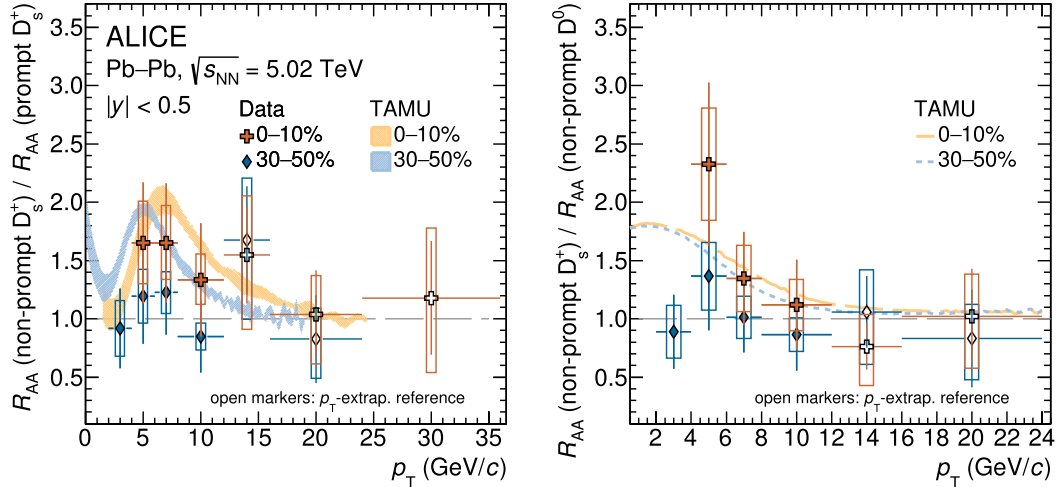
Fig. 7. The R_{AA} of non-prompt D_s^+ mesons divided by the one of prompt D_s^+ mesons [19] (left panel) and non-prompt D^0 mesons [21] (right panel) for the 0–10% and 30–50% centrality intervals in Pb-Pb collisions at \sqrt{s_{NN}} = 5.02 TeV. The measurements are compared with TAMU model predictions [70]. Statistical (bars) and systematic (boxes) uncertainties are shown.
