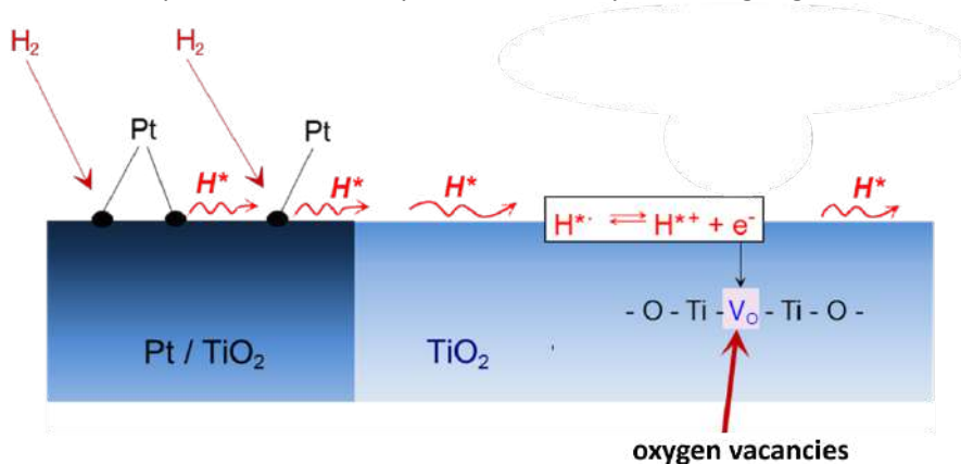
Figure 1: Elementary processes occurring at an impedance sensor for hydrogen detection.
