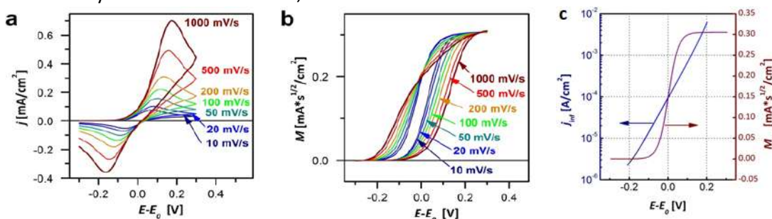
Simulated CVs (a), their semiintegrals (b), and the calculated j_{\text{inf}} and M_{\text{rev}} functions (c). Simulation parameters: D_{\text{red}} = D_{\text{ox}} = 10^{-5} \text{ cm}^2/\text{s} , c_{\text{red}} = 10^{-6} \text{ mol/cm}^3 , c_{\text{ox}} = 0 \text{ mol/cm}^3 , E_0 = 0 , k_0 = 0.001 \text{ cm/s} , \alpha = 0.5 .
