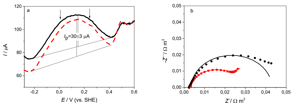
Fig. 1. a) DPVs recorded on the third (solid line) and fifth day (dashed line) of culturing at polarization; b) Nyquist plots obtained at the 15 th (squares) and 120 th h of poisoning for biofilm formation, dots - measured data, lines –fitted data.
