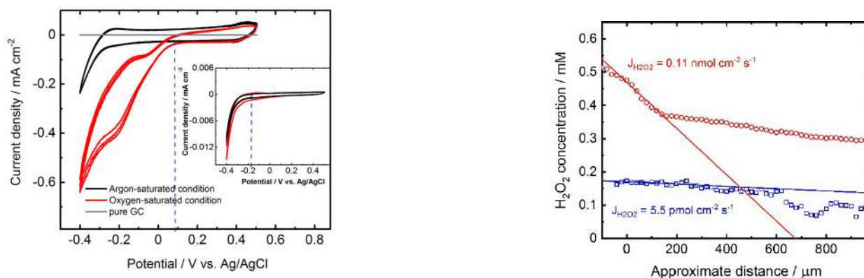
(Left) Cyclic voltammograms recorded at GC modified with LiB waste powder, 5 mV s -1 . (Right) H 2 O 2 concentration gradient at unmodified (blue) and modified (red) trifluorotoluene|0.1 M HClO 4 aqueous interface. From Ref. [4].
