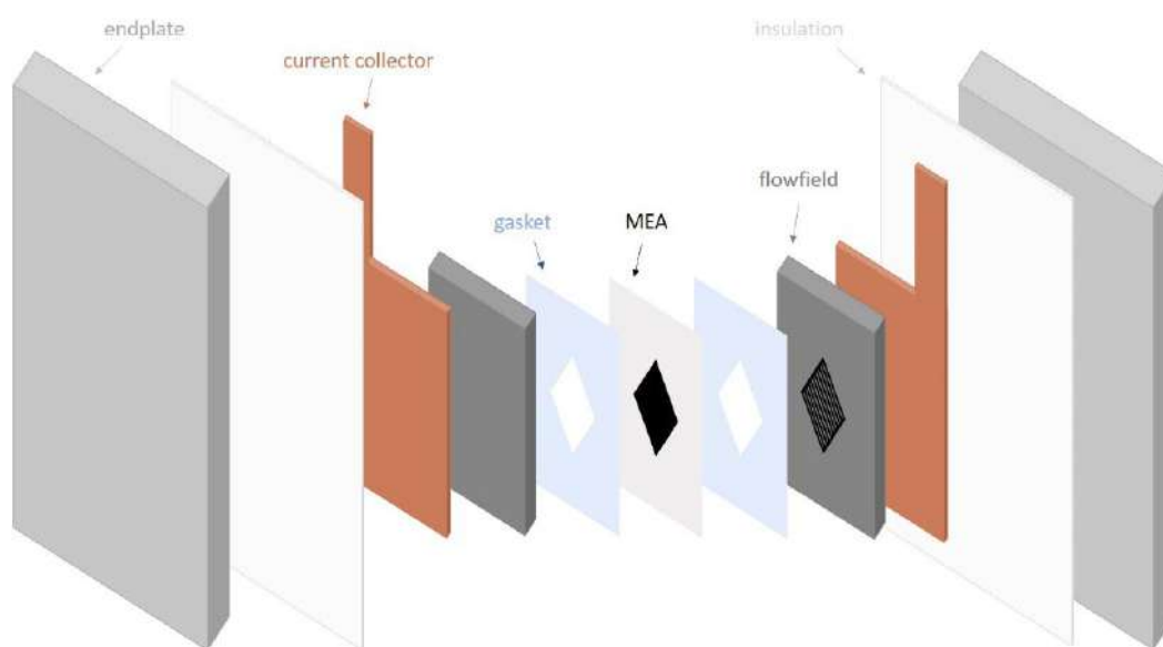
Figure 1: Simplified exploded view of the utilized in-house fabricated ADEFC.
