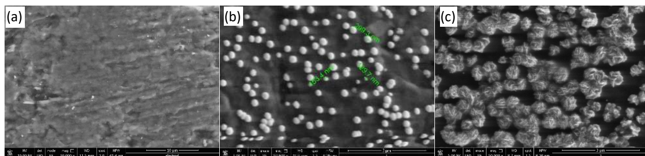
Figure 1. SEM micrographs of bare PG substrate (a) and of Pt-PG electrodes obtained by pulsed current deposition from 5 mM \text{H}_2\text{PtCl}_6 in 1 M HCl solution, at different current densities: 5 \text{mA cm}^{-2} (b) and 25 \text{mA cm}^{-2} (c).
