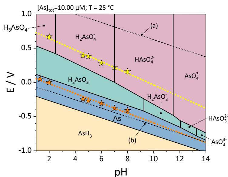
Fig. 1: Calculated Pourbaix diagram for a total arsenic content of 10.00 µmol/l at 25 °C. This represents the potential E depending on pH for red areas indicating As(V) species; turquoise areas indicating As(III) species, blue area – elemental As(0) and yellow area – gaseous AsH_3 . The stars show the positions of the peak maxima from performed anodic stripping voltammetric measurements. The dotted orange line represents the linearization of the peak maxima at the transition from As(0) \rightarrow As(III). The dotted yellow line represents the linearization of the peak maxima at the transition from As(III) \rightarrow As(V). Dashed lines (a) O_{2(g)} + 4 H^+_{(aq)} + 4 e^- \rightarrow 2 H_2O_{(l)} and (b) 2 H^+_{(aq)} + 2 e^- \rightarrow H_{2(g)} enclose the theoretical region of stability of the water to oxidation or reduction.
