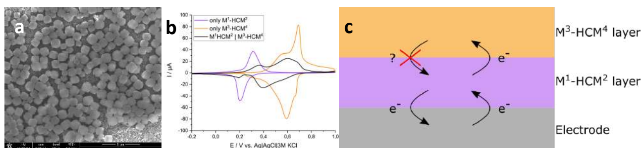
Figure 1: Two-layer M-HCM system. a) SEM image of the morphology of a composite of an electrodeposited smooth \text{M}^1\text{-HCM}^2 film coated with a second layer of bulk-synthesized crystalline \text{M}^3\text{-HCM}^4 colloids; b) Cyclic voltammogram of bilayer system revealing rectifying behavior; c) schematic illustration of proposed electronic mechanism in bilayer system.
