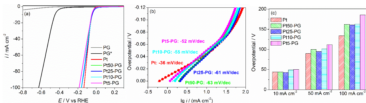
Figure 2. Polarization curves in 0.5 M \text{H}_2\text{SO}_4 solution at scan rate 50 \text{mV s}^{-1} (a). Tafel plots of Pt and Pt-PG electrodes (b). Required overpotential to reach a current density of 10, 50 and 100 \text{mA cm}^{-2} for Pt and Pt-PG electrodes (c).
