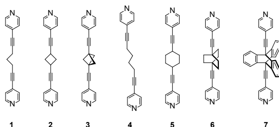
Figure 1 Structure of molecular "rods".
